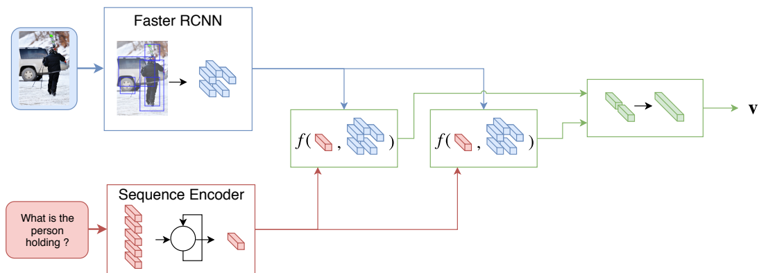
Figure 5.1 – Multi-glimpse attention. In this figure, two attention modules process the set of region vectors with respect to the question. Each of these glimpses provides a question-based image representation, both computed in parallel. Finally, the outputs of the glimpses are concatenated to provide the final image representation.
