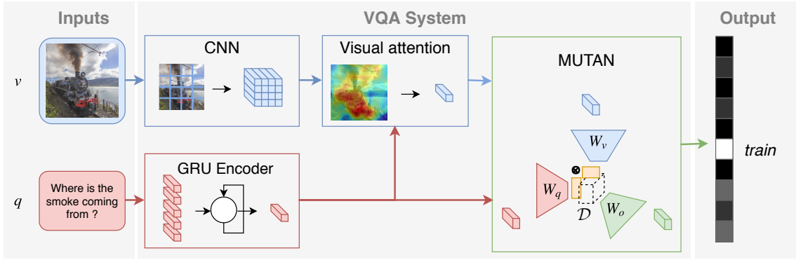
Figure 3.6 – Attention-based MUTAN architecture for VQA The question is processed by a GRU encoder to provide a single vector, and the image passes through a fully convolutional ConvNet to yield a 14 \times 14 \times d_v features map. Both these representations are fused with a MUTAN bilinear model, within an attentional framework.
