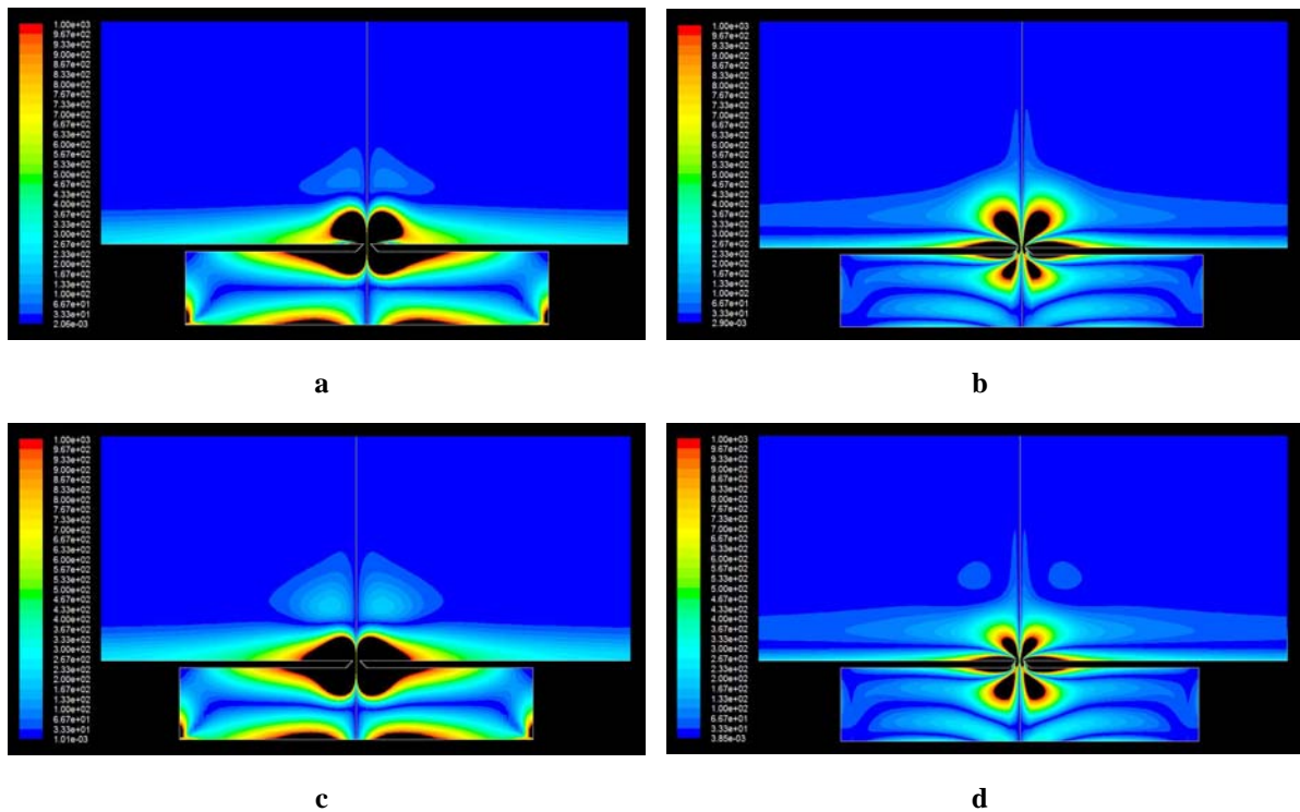
Figure 6.23 - Iso-contours de vorticit  pour le micro JS – fente type I – f = 1140 Hz, A = 7.62 \mu m a) t/T = 0.25 , b) t/T = 0.5 , c) t/T = 0.75 , d) t/T = 1
