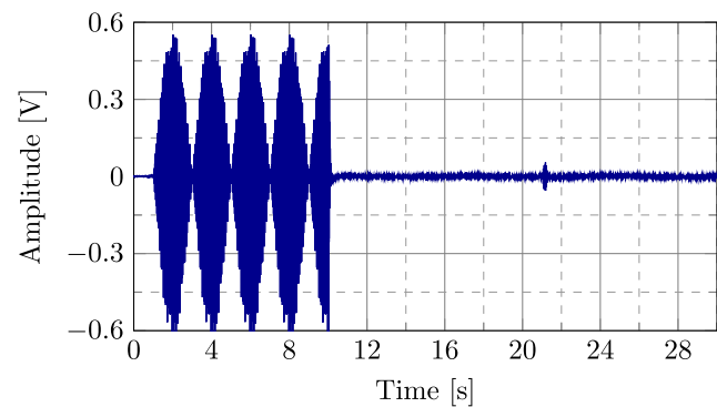
Fig. 9. Acoustic interference attenuation using an adaptive controller. Noise frequencies: 170+170.5 Hz and 285+285.5 Hz then 180+180.5 Hz and 295+295.5 Hz. Loop closed at 10 s.
