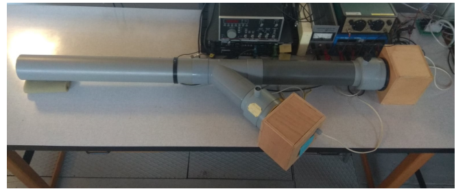
Fig. 1. Duct active noise control test-bench (Photo).
