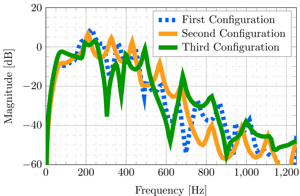
FIGURE 6.7. Identified secondary path for first, second and third test bench configurations.
