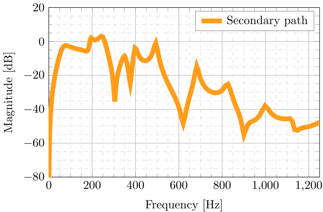
FIGURE 3.13. Third test bench configuration's identified secondary path.
