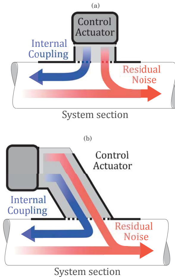
FIGURE 2.1. (a) Standard control actuator positioning. (b) Proposed control actuator positioning.
