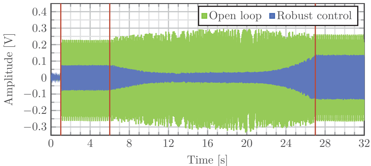
FIGURE 4.12. Residual noise in open loop vs closed loop using a robust controller under the effect of tonal disturbances with variable frequencies.
