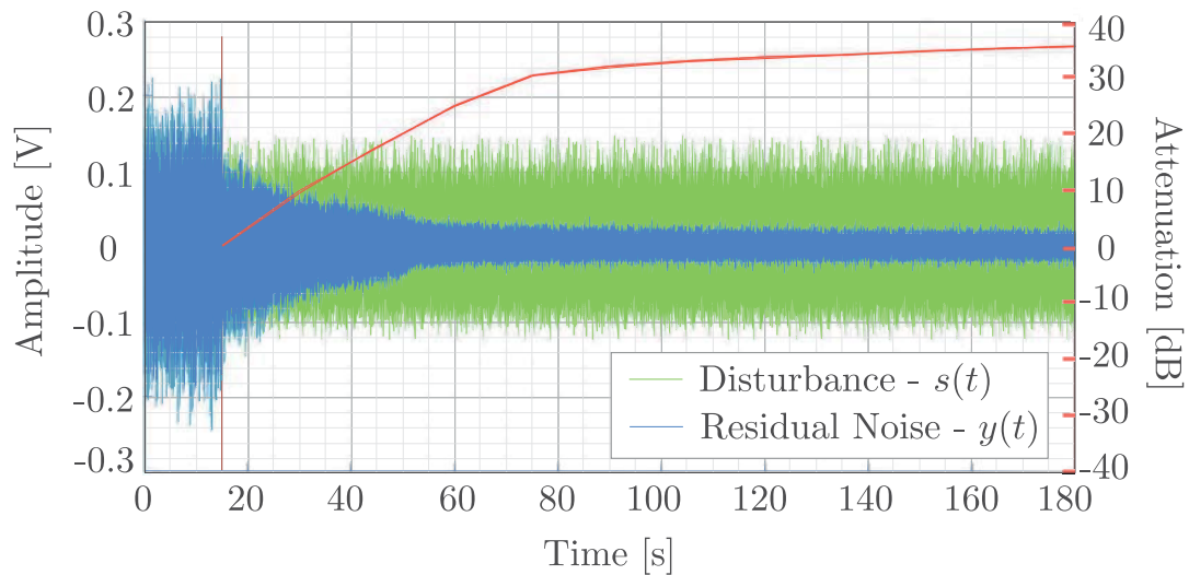
FIGURE 5.16. Performance of YK-IIR compensator order 30/30 with FuSBA PAA and constant trace profile ( \text{tr}[F]_{pp} = 0.10 ). Right side shows the level of attenuation achieved at a given point in time, with 35.6 dB achieved at 180 s. Compensation starts at 15 s.
