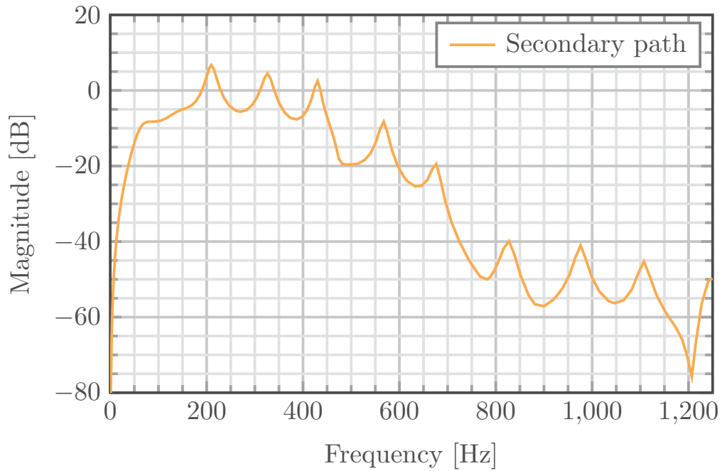
FIGURE 3.9. Identified secondary path for second test bench configuration.
