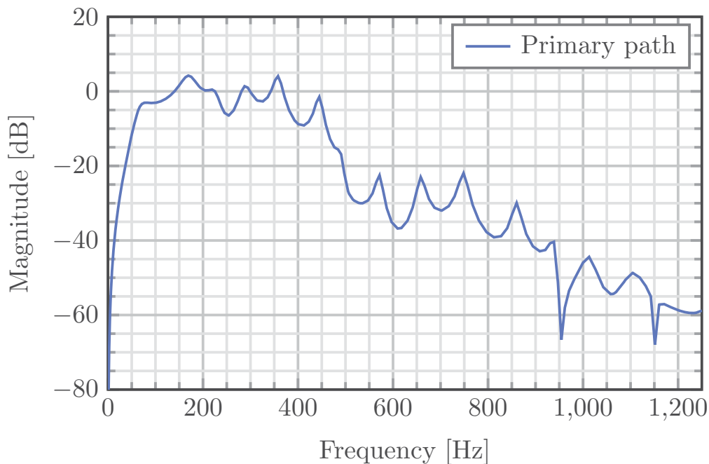
FIGURE 3.5. Identified primary path for first test bench configuration.
