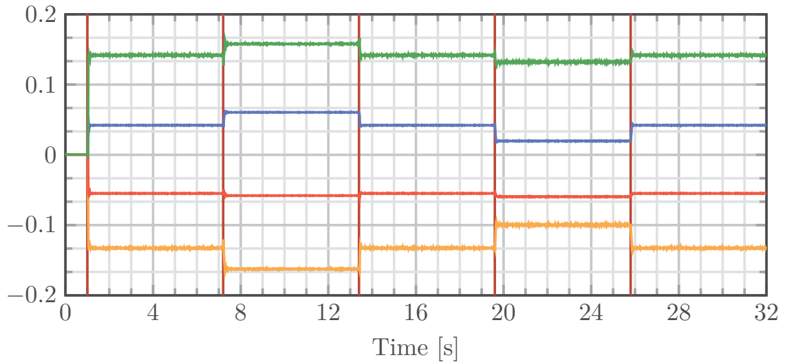
FIGURE 4.11. Parameters evolution for step changes in frequencies test using an adaptive controller with YK parametrization.
