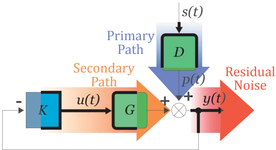
FIGURE 2.6. Feedback control scheme.
