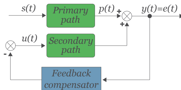
FIGURE 1.6. Feedback control problem scheme.
