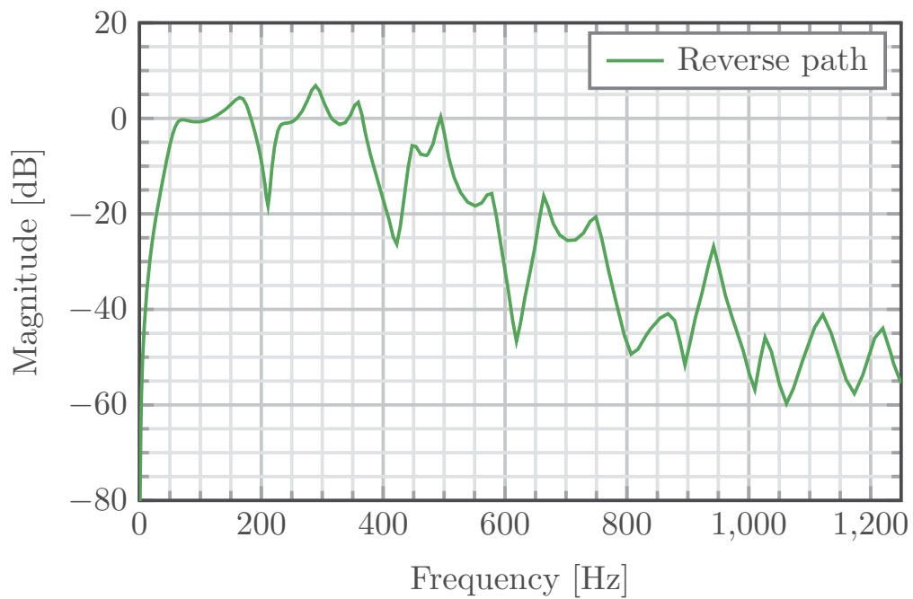
FIGURE 3.7. Identified reverse path for first test bench configuration.
