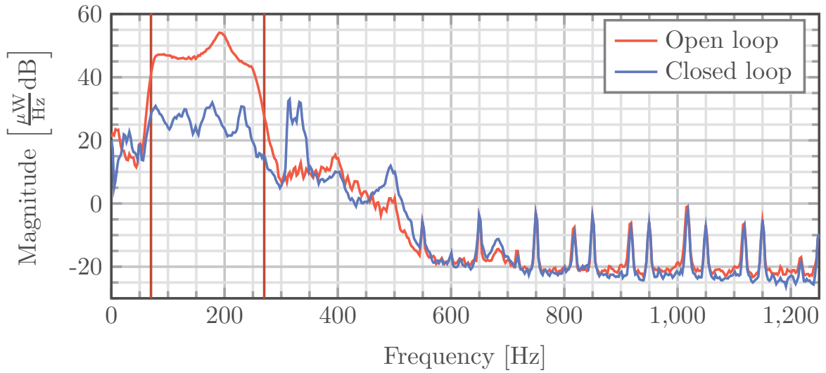
FIGURE 5.13. Comparison between measured noise's PSD of a disturbance with frequencies between 70 Hz and 270 Hz without compensation (Open loop), and measured residual noise of the system at 180 s, using a standard FuSBA PAA with a constant trace profile and \text{tr}[F]_{pp} = 0.010 (Closed loop).
