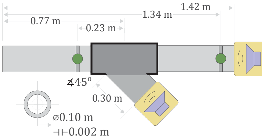
FIGURE 5.5. Third experimental test bench configuration.
