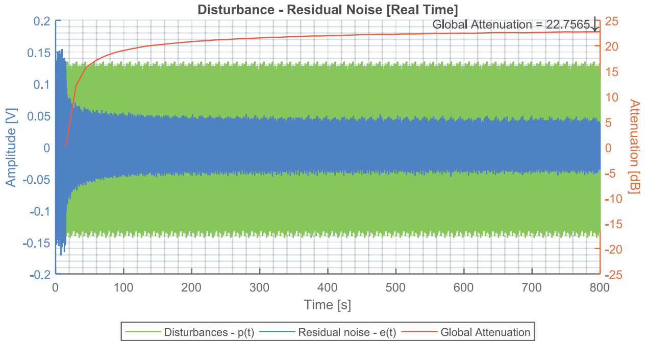
Figure 10: Performance of YK FIR adaptive compensator with 60 parameters (experimental).
