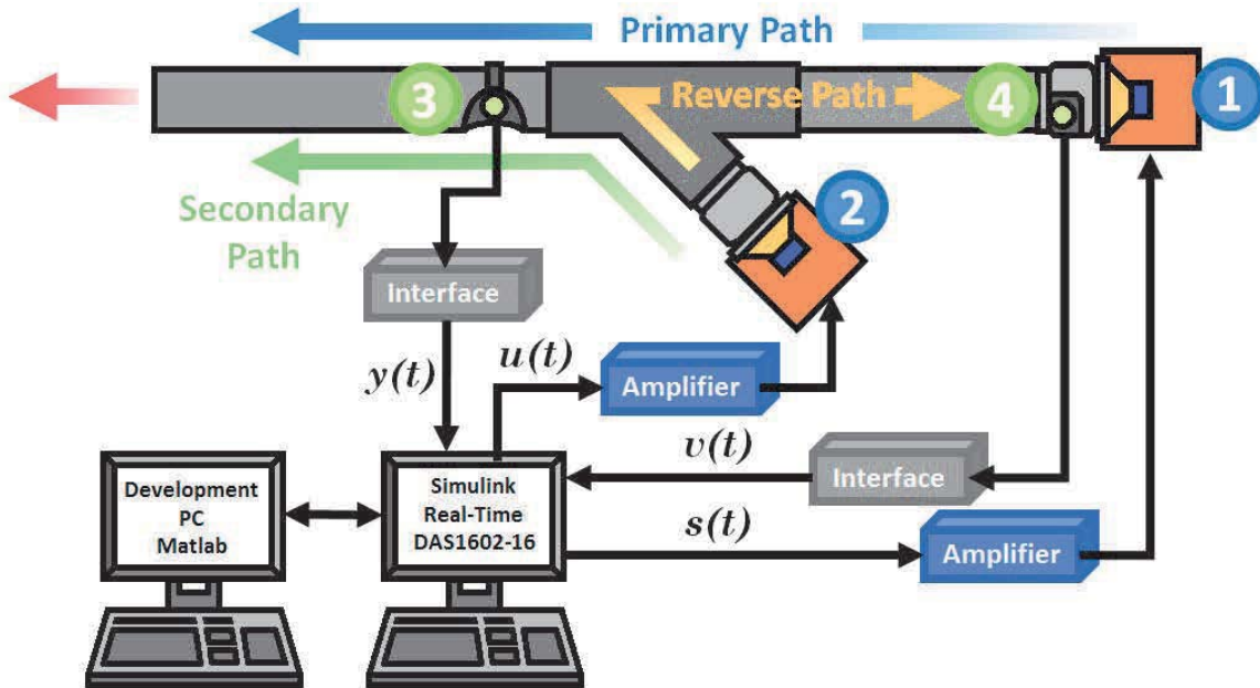
FIGURE 5.4. Schema of test bench's feedforward configuration.
