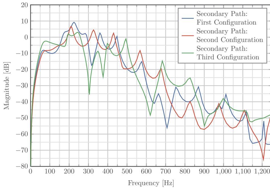
FIGURE 2.14. Secondary path models comparison. Frequency response of all test bench's configurations.
