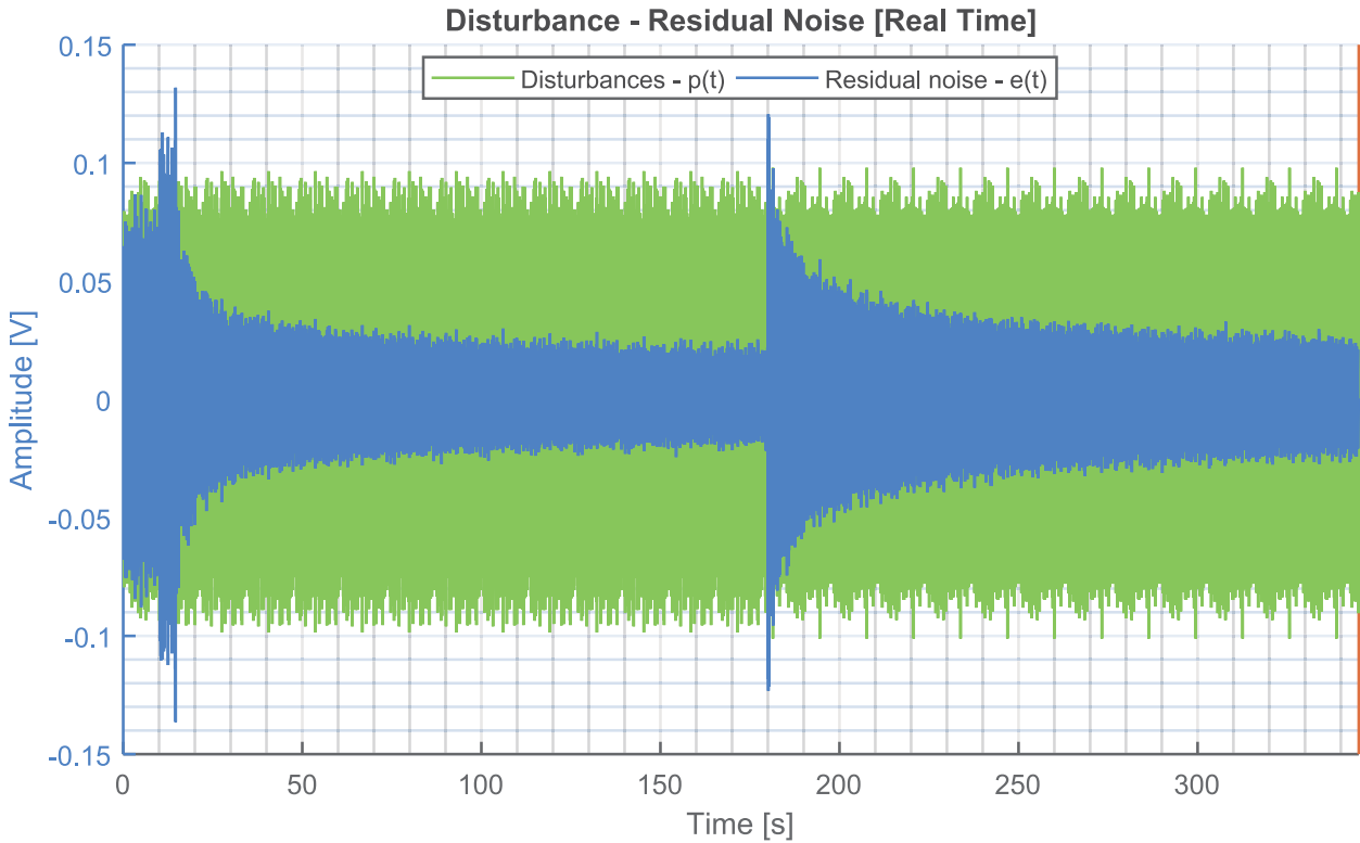
Figure 11: Transient performance of YK FIR adaptive compensator (experimental). 0 to 180s: broad-band disturbance 150-250 Hz; 180-345 s: broad-band disturbance 250-350 Hz; open loop operation: 0 to 15s
