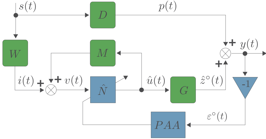
FIGURE 5.9. Feedforward control scheme with PAA.
