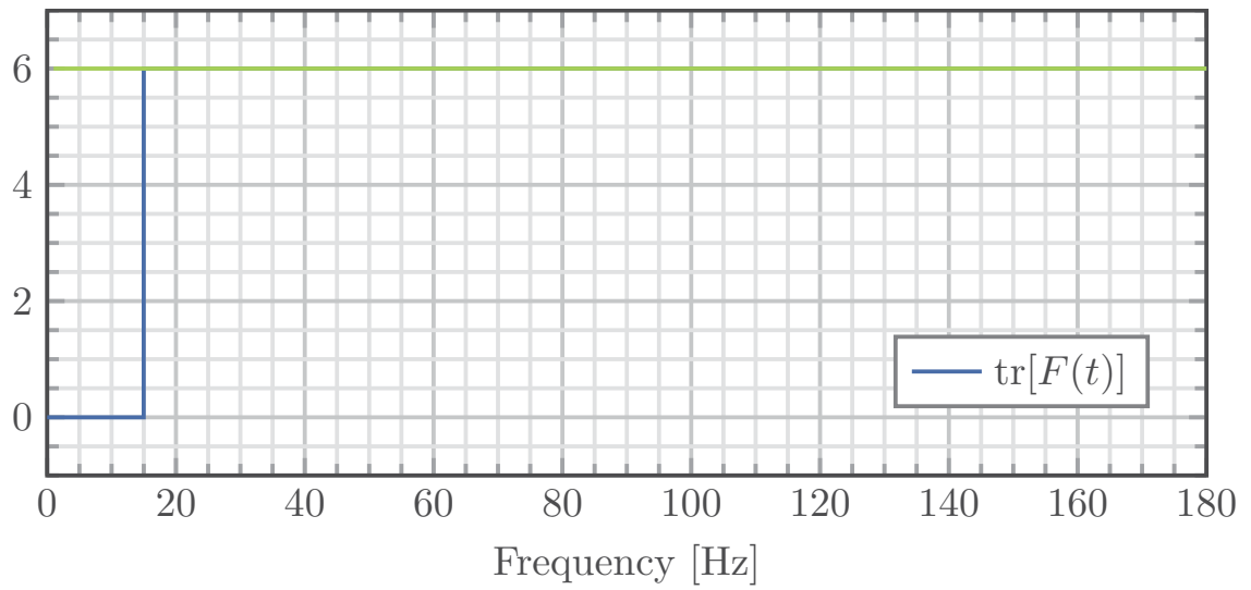
FIGURE 5.19. Evolution of adaptation matrix F 's trace for a constant trace profile of a YK FuSBA PAA. A value of \text{tr}[F]_{pp} = 0.10 was chosen, so \text{tr}[F(t)] = \text{tr}[F] = 6.0
