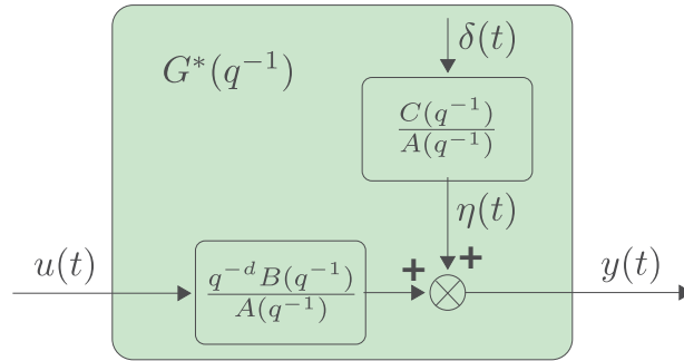
FIGURE 3.1. ARMAX process diagram.
