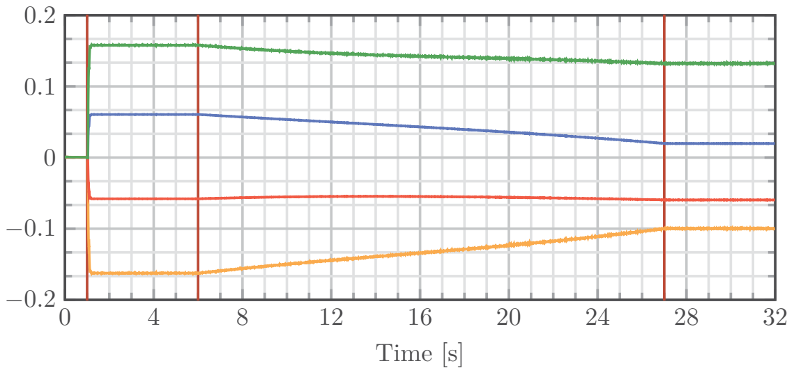
FIGURE 4.14. Parameters evolution for the tonal disturbances with variable frequencies test using an adaptive controller with YK parametrization.
