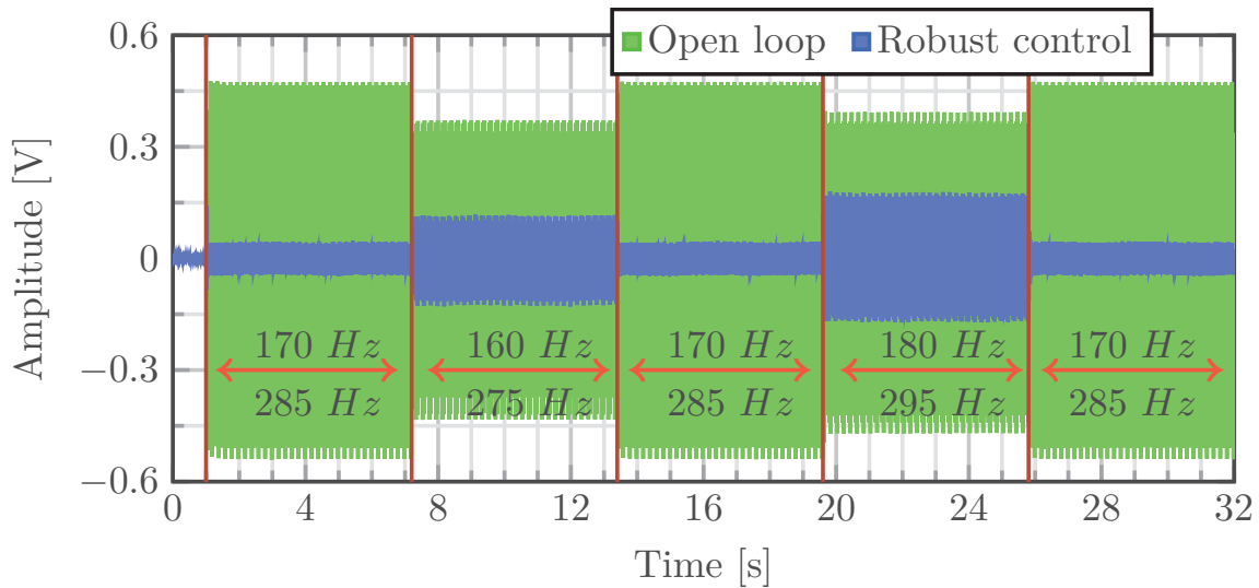
FIGURE 4.9. Step changes in frequencies using the robust controller. Residual noise: open loop vs closed loop.
