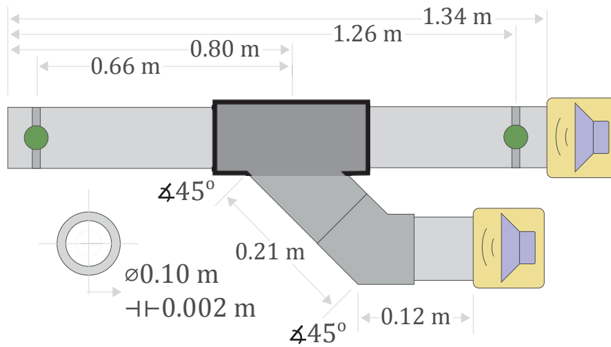
FIGURE 2.2. First experimental test bench configuration.
