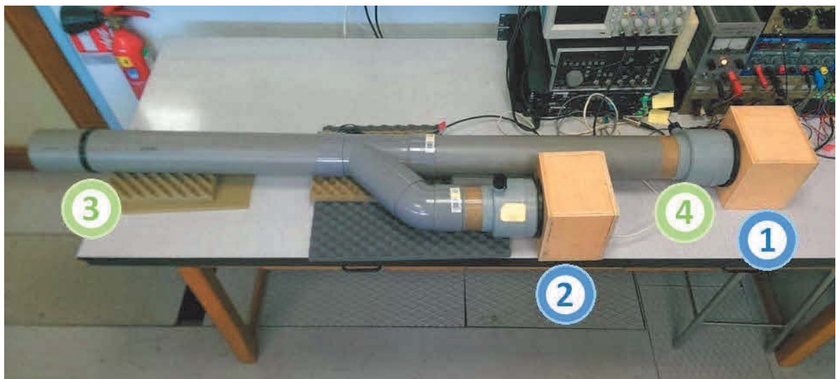
FIGURE 2.3. Photo of test bench's first configuration.
