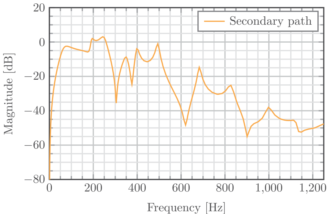
FIGURE 2.13. Third test bench configuration's identified secondary path.
