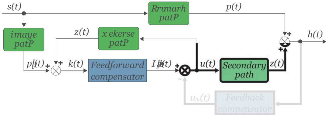
FIGURE 1.7. Reduced block diagram representation for a feedforward control problem.
