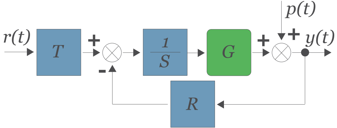
FIGURE 2.5. RST general controller scheme.
