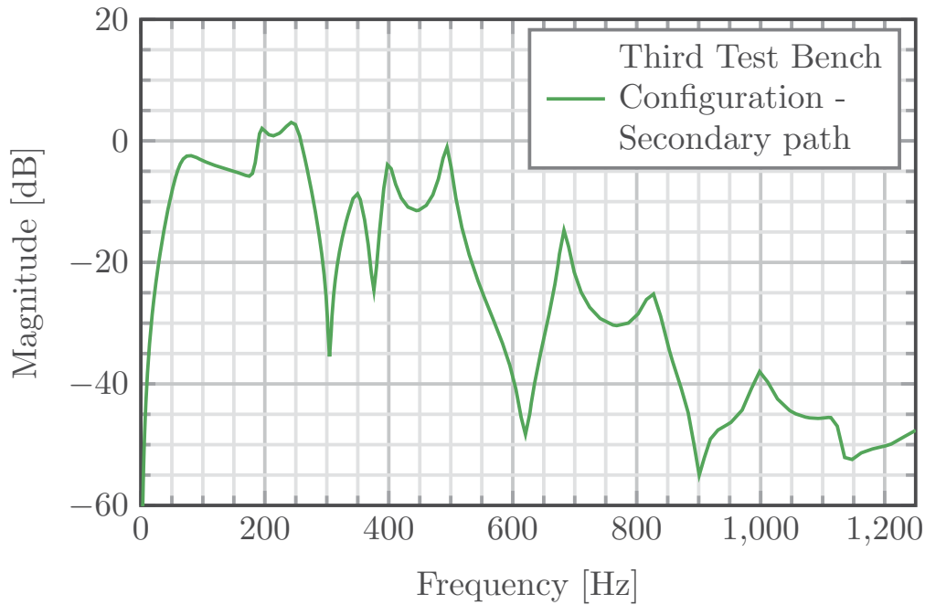
FIGURE 5.11. Identified secondary path for the third test bench configuration.
