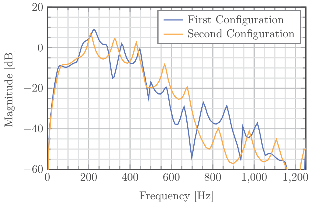
FIGURE 5.3. Identified secondary path for first and second test bench configurations.
