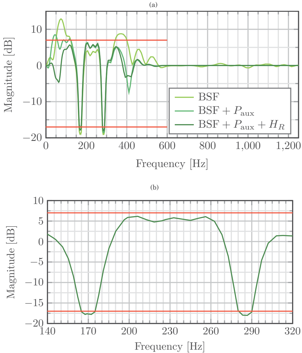
FIGURE 4.4. Output sensitivity function S_{yp} : a) Evolution of the fixed robust controller, and b) final controller zoomed region of interest.
