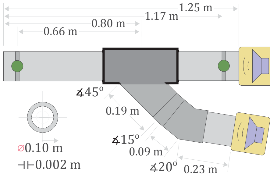
FIGURE 2.8. Second experimental test bench configuration.
