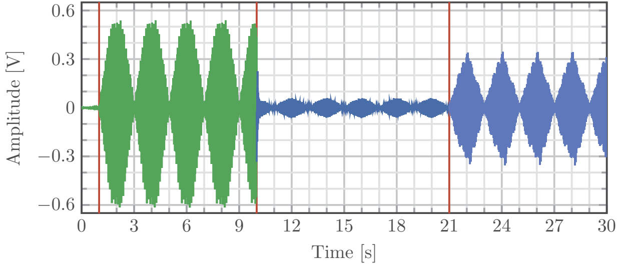
FIGURE 4.6. Acoustic interference attenuation using a robust controller.
