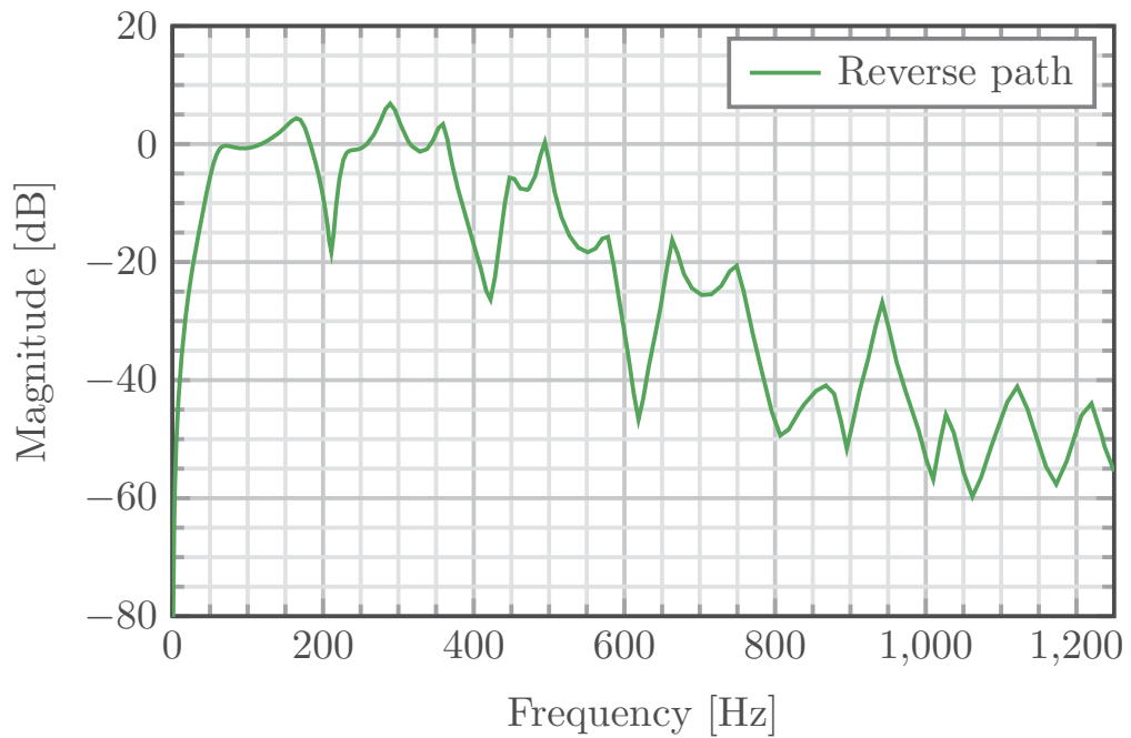
FIGURE 3.7. Identified reverse path for first test bench configuration.
