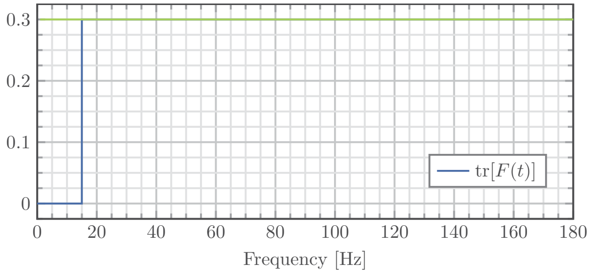
FIGURE 5.15. Evolution of adaptation matrix F 's trace for a constant trace profile of a FuSBA PAA. A value of \text{tr}[F]_{pp} = 0.010 was chosen, so \text{tr}[F(t)] = \text{tr}[F] = 0.3
