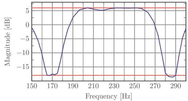
Fig. 6. Robust controller's output sensitivity function evolution—zoomed-in view.
