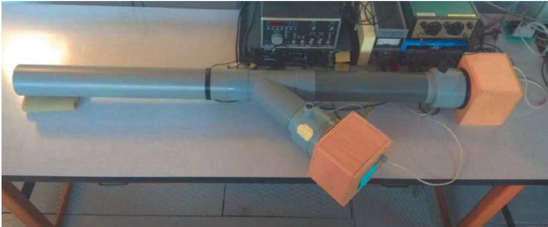
FIGURE 5.6. Photo of test bench's third configuration.
