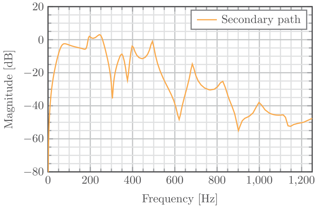
FIGURE 3.11. Identified secondary path for third test bench configuration.
