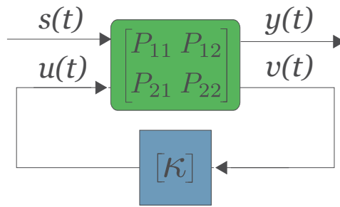
FIGURE 1.3. General representation of a 2 input - 2 output Active Noise Control / Active Vibration Control system.
