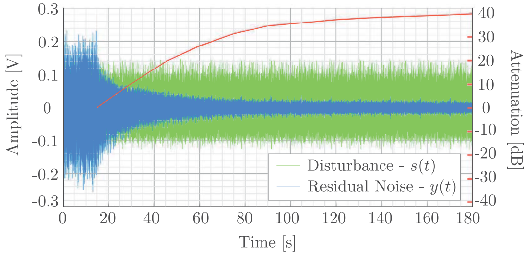
FIGURE 5.12. Performance of IIR compensator of order [15/15] with FuSBA PAA and constant trace profile ( \text{tr}[F]_{pp} = 0.010 ). Right side shows the level of attenuation achieved at a given point in time, with 39.6 dB achieved at 180 s. Compensation starts at 15 s.
