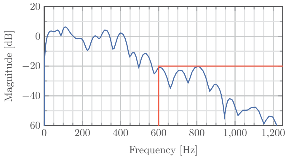
FIGURE 4.2. Input sensitivity function S_{up} of a fixed linear controller.
