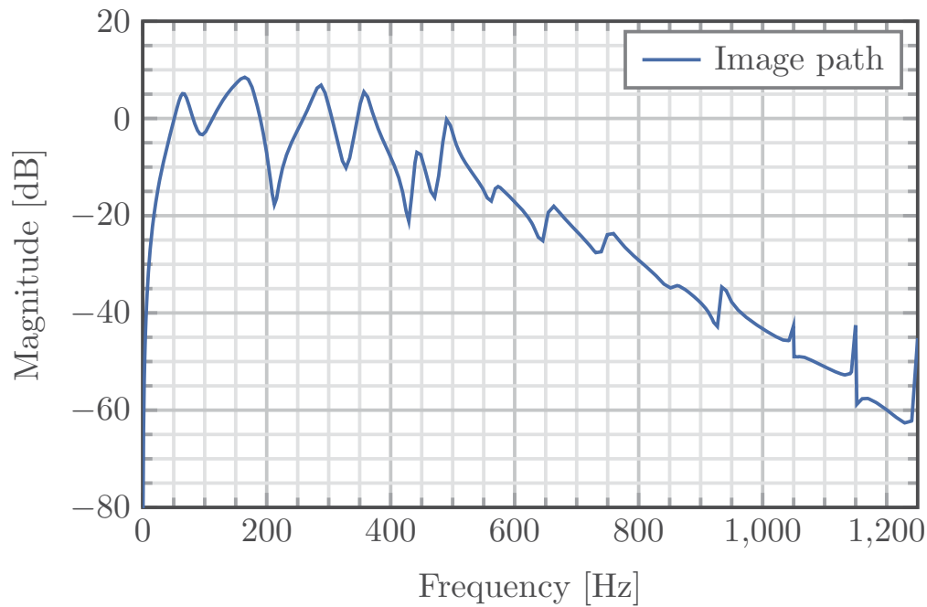
FIGURE 3.8. Identified image path for first test bench configuration.
