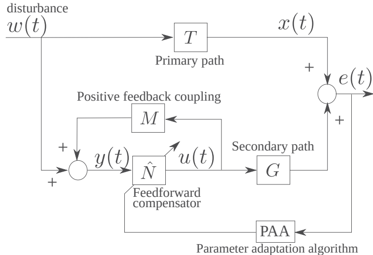
Figure 1: Adaptive active noise feedforward compensation.
