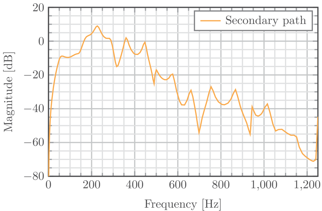
FIGURE 2.7. First test bench configuration's identified secondary path.
