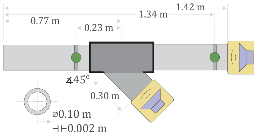
FIGURE 2.11. Third experimental test bench configuration.
