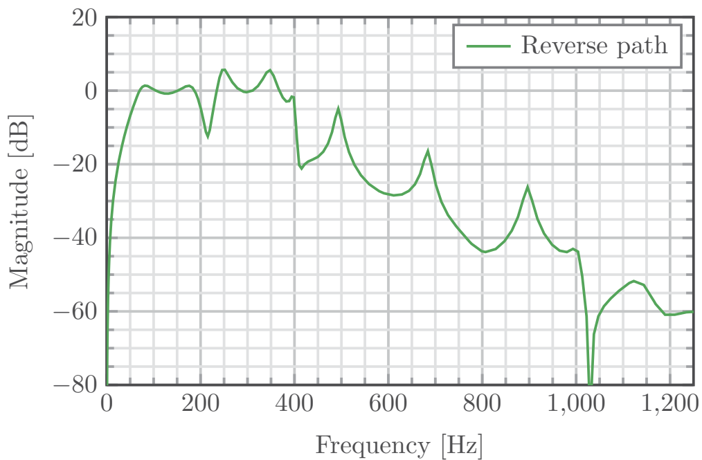
FIGURE 3.12. Identified reverse path for third test bench configuration.
