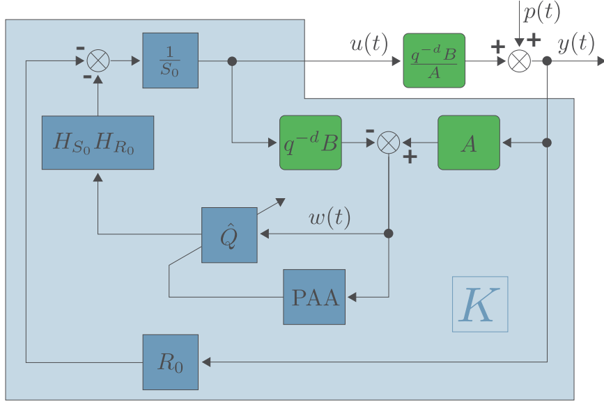
FIGURE 4.5. Adaptive Youla-Kučera parametrization scheme.
