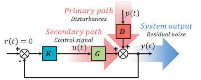
Fig. 3. Feedback regulation scheme.
