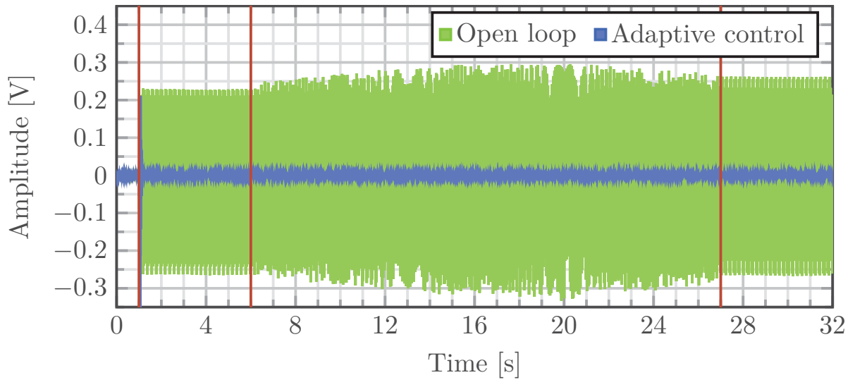
FIGURE 4.13. Residual noise in open loop vs closed loop using the adaptive controller with YK parametrization under the effect of tonal disturbances with variable frequencies.
