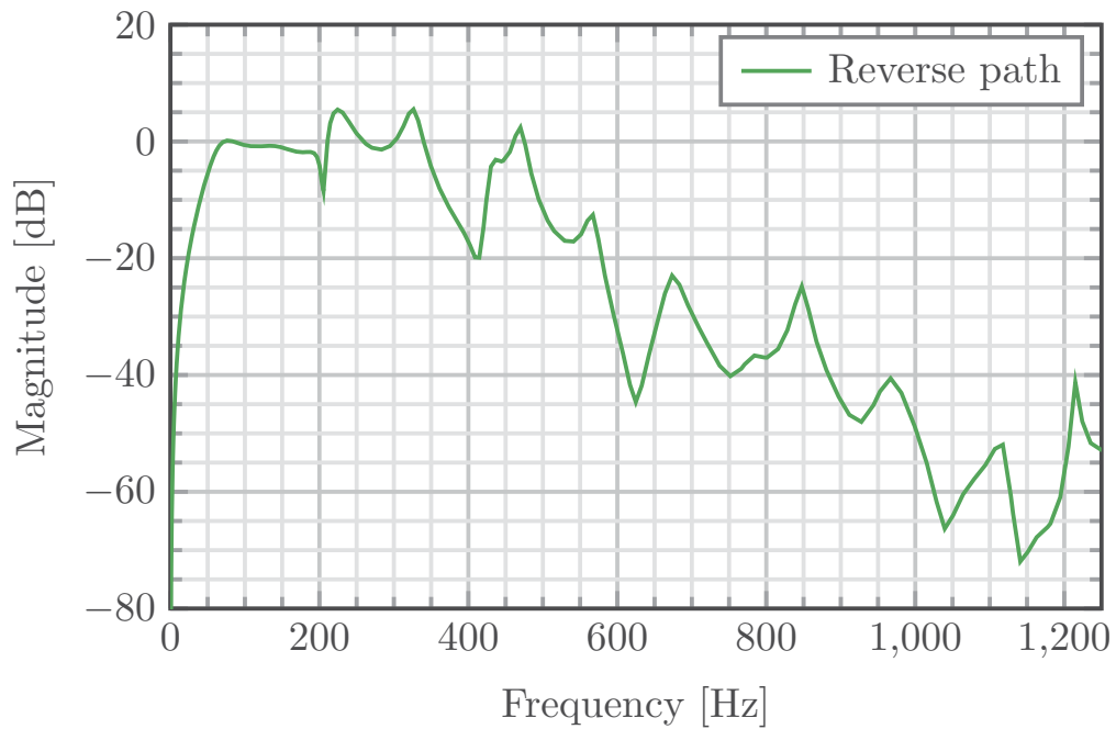
FIGURE 3.10. Identified reverse path for second test bench configuration.
