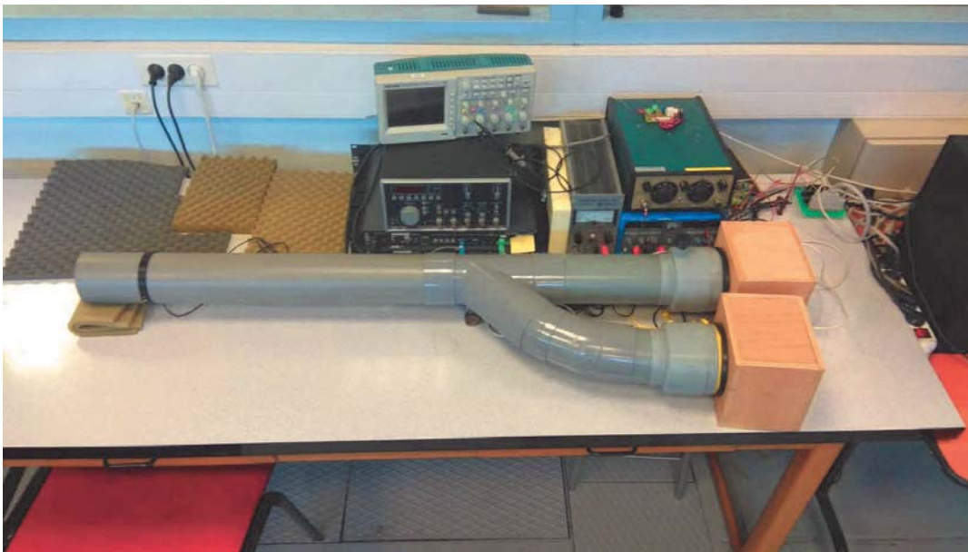
FIGURE 5.2. Photo of test bench's second configuration.
