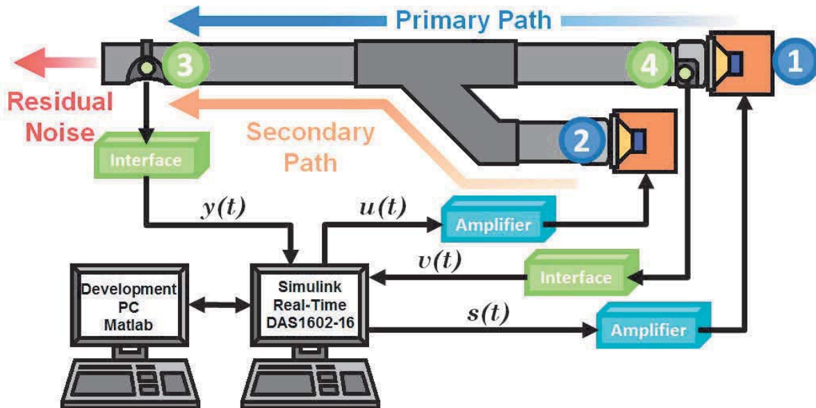
FIGURE 2.4. Schema of test bench's first configuration.
