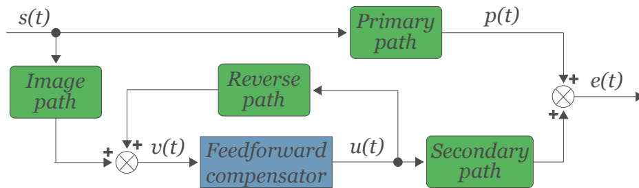
FIGURE 1.8. Feedforward control problem schema.
