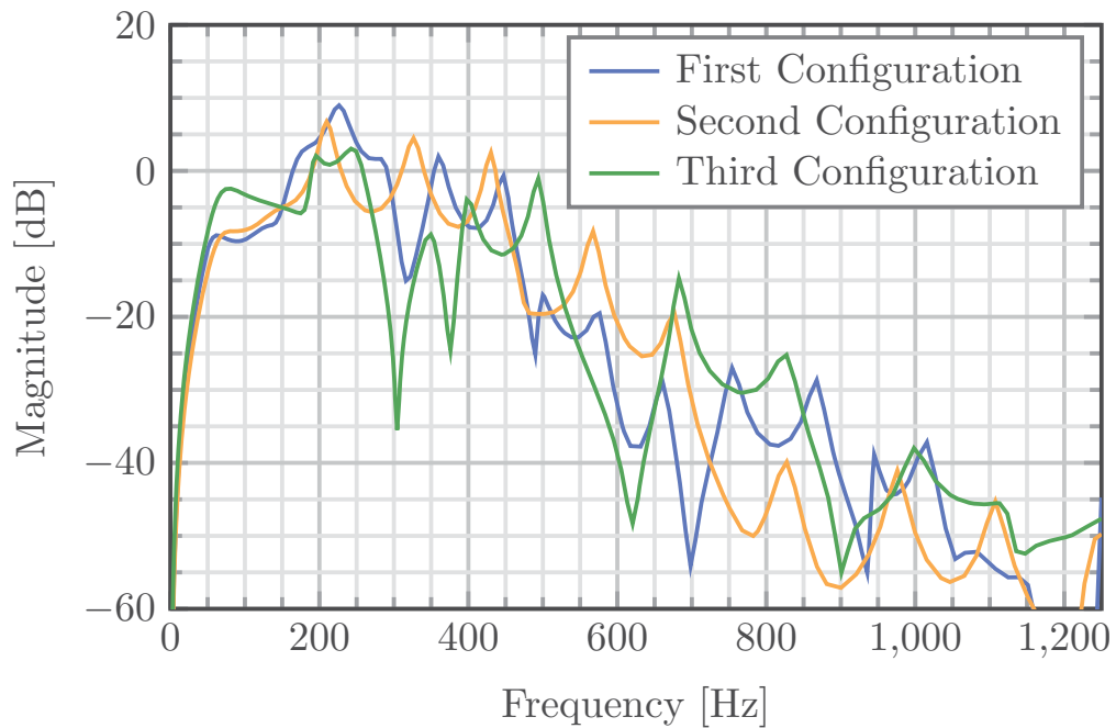
FIGURE 5.7. Identified secondary path for first, second and third test bench configurations.
