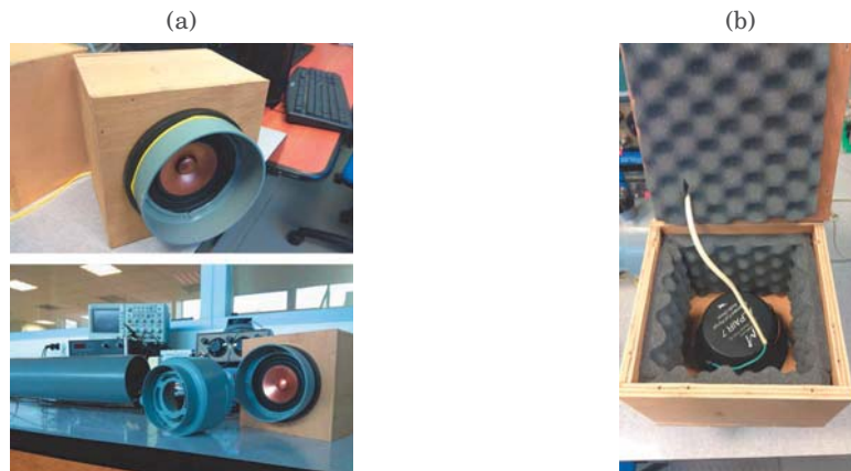
FIGURE 2.15. Anechoic boxes Set up.
