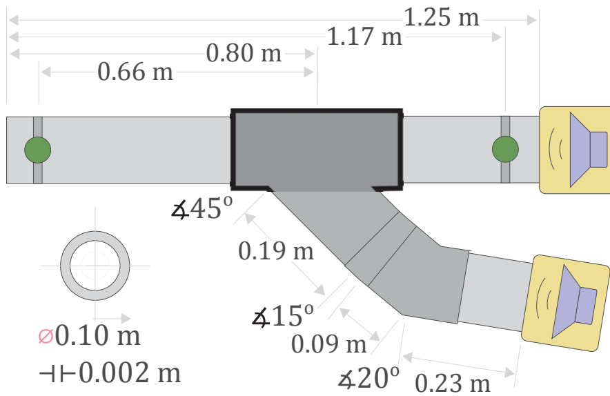
FIGURE 5.1. Second experimental test bench configuration.
