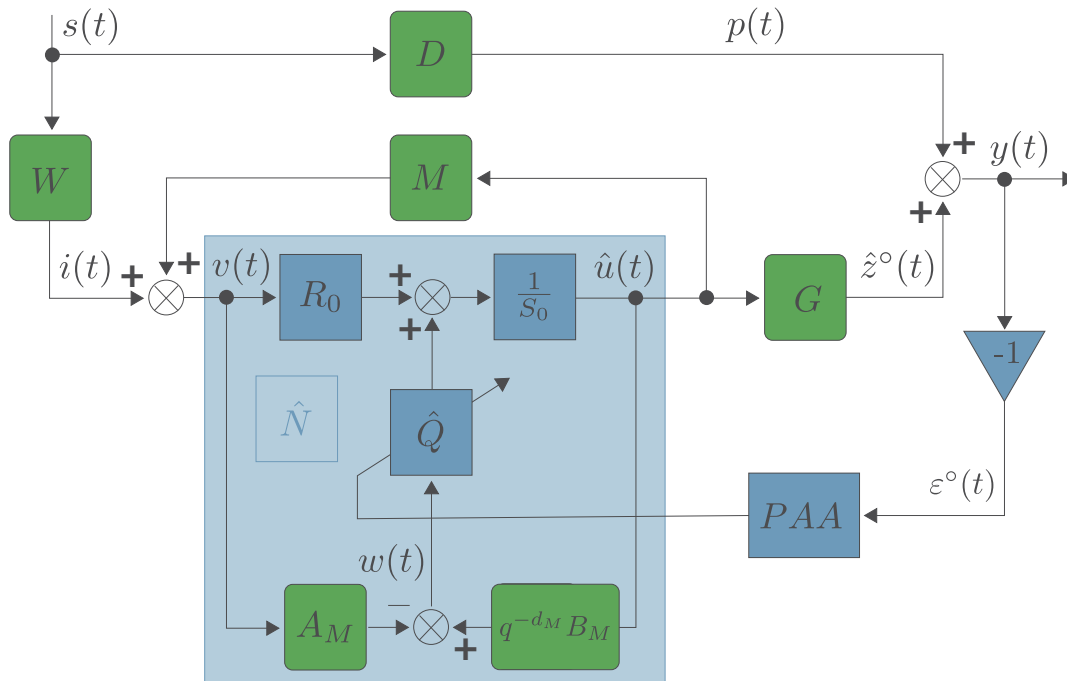
FIGURE 5.10. Feedforward control scheme using a Youla-Kučera parametrization with PAA.
