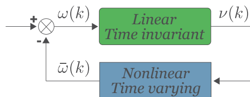
FIGURE 1.9. Standard representation of the analysis of adaptive systems using hyperstability theory.
