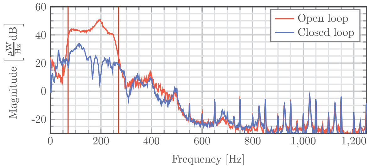
FIGURE 5.17. Comparison between measured noise's PSD of a disturbance with frequencies between 70 Hz and 270 Hz without compensation (Open loop), and measured residual noise of the system at 180 s, using a YK FuSBA PAA with a constant trace profile and \text{tr}[F]_{pp} = 0.10 (Closed loop).
