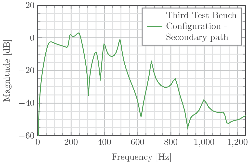
FIGURE 5.11. Identified secondary path for the third test bench configuration.
