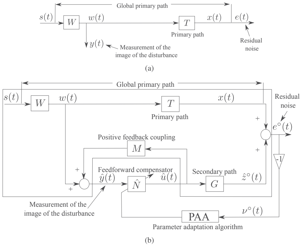
Figure 6: Feedforward ANC: in open-loop (a) and with adaptive feedforward compensator (b).
