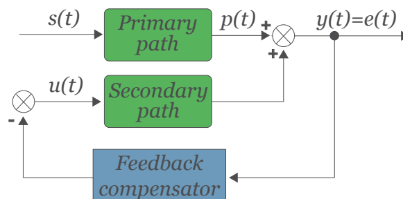
FIGURE 1.6. Feedback control problem scheme.
