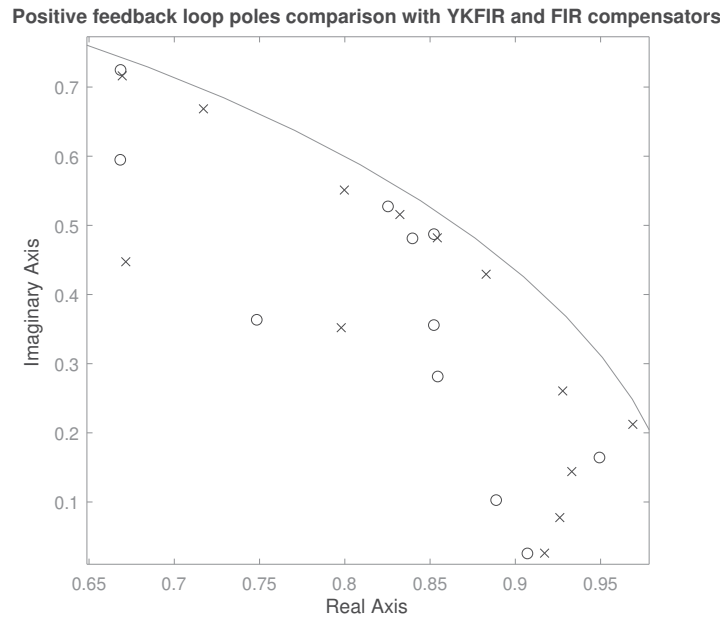
Figure 9: Comparison of the positive feedback loop poles for the YK FIR (o) and FIR (x) adaptive compensators (simulation).
