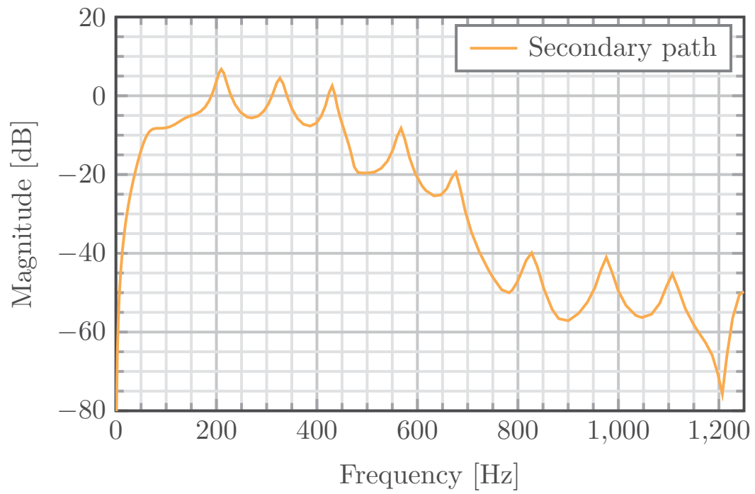
FIGURE 2.10. Second test bench configuration's identified secondary path.
