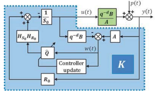
Fig. 7. Adaptive YK parameterization scheme.
