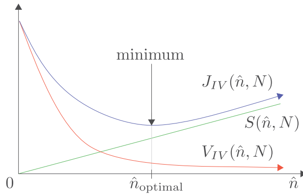
FIGURE 3.2. Evaluation of the penalized instrumental variable criterion for order estimation.
