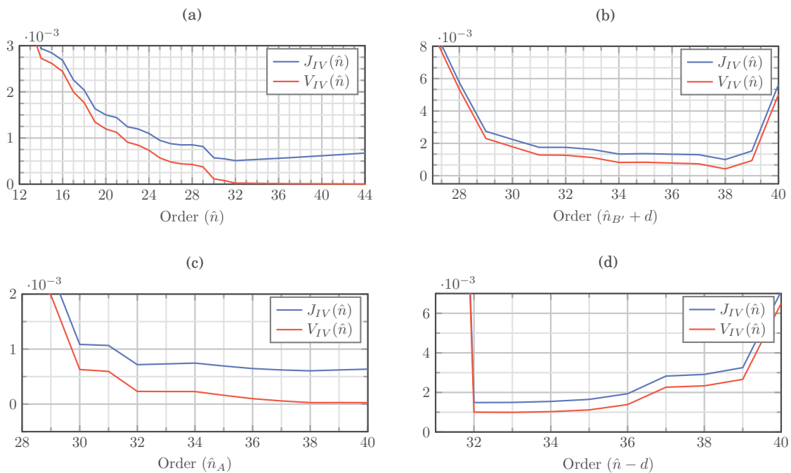
FIGURE 3.3. Order estimation using an Instrumental Variable and complexity penalty, with estimation for (a) \hat{n} , (b) \hat{n}_{B'} + \hat{d} , (c) \hat{n}_A , and (d) \hat{n} - \hat{d} .
