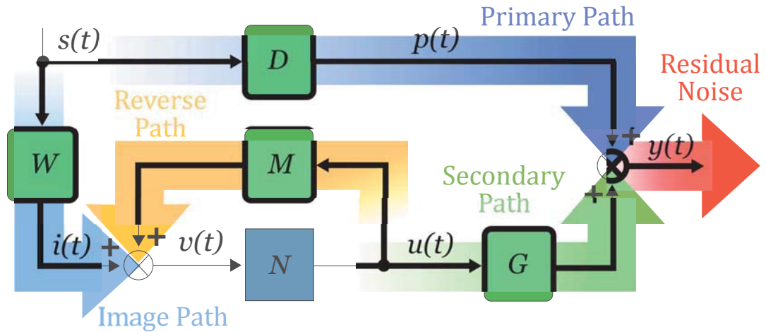
FIGURE 5.8. Feedforward control scheme.
