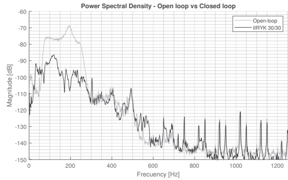
Fig. 14. PSD of the IIRYK 30/30 adaptive compensators using FUSBA matrix adaptation (70-270 Hz disturbance, 600 s experiments).
