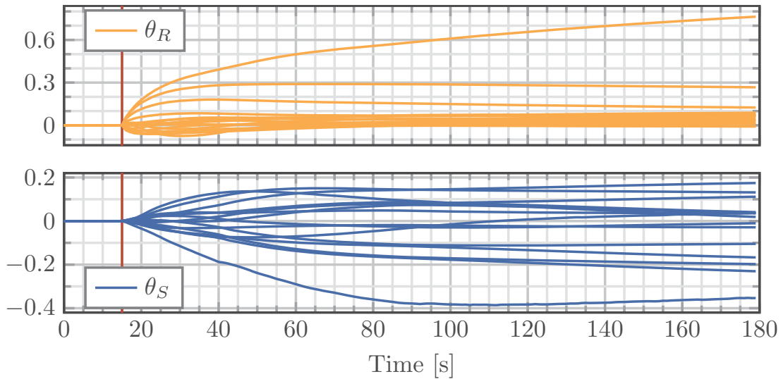
FIGURE 5.14. Filter N(q^{-1}) = \frac{R}{S} parameters evolution for a [15/15] standard IIR filter using FuSBA PAA with a constant trace profile. Compensation starts at 15 s.
