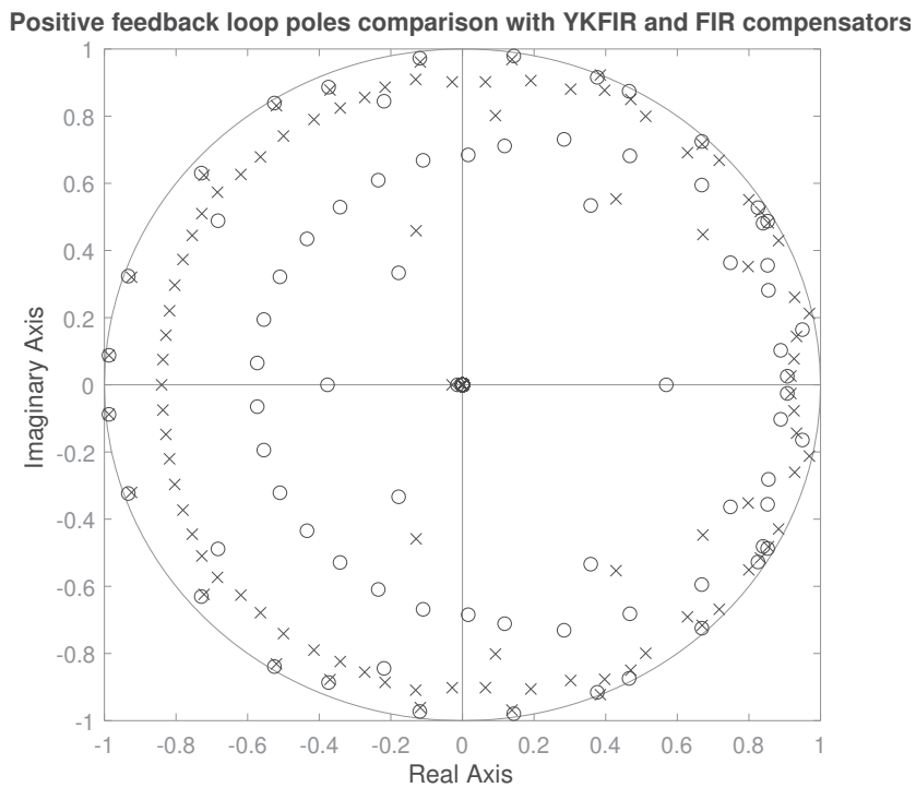
Figure 8: Comparison of the positive feedback loop poles for the YK FIR (o) and FIR (x) adaptive compensators (simulation).
