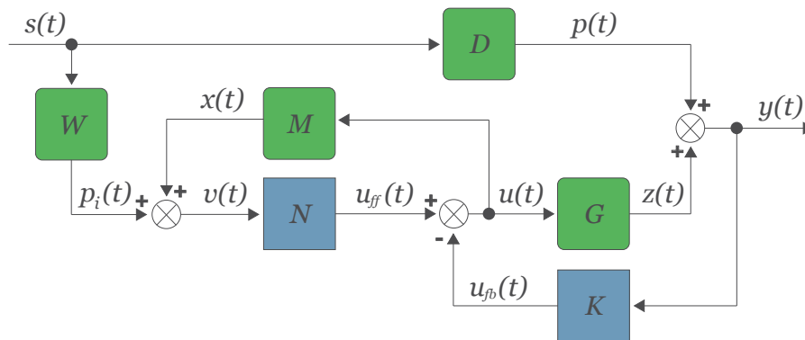
FIGURE 1.4. Block scheme of the combined feedback and feedforward control problem.
