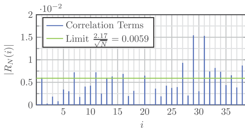
FIGURE 3.4. Whiteness test for identified secondary path.
