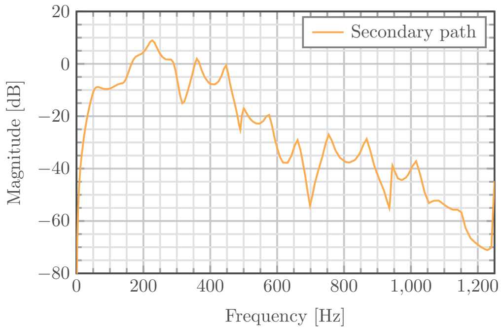
FIGURE 3.6. Identified secondary path for first test bench configuration.
