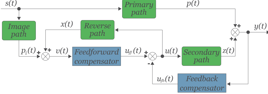
FIGURE 1.2. Block diagram representation of the combined feedback and feedforward control problem. In green we can identify the blocks corresponding to the system's plant, meanwhile in blue the corresponding feedback K and feedforward N compensators.
