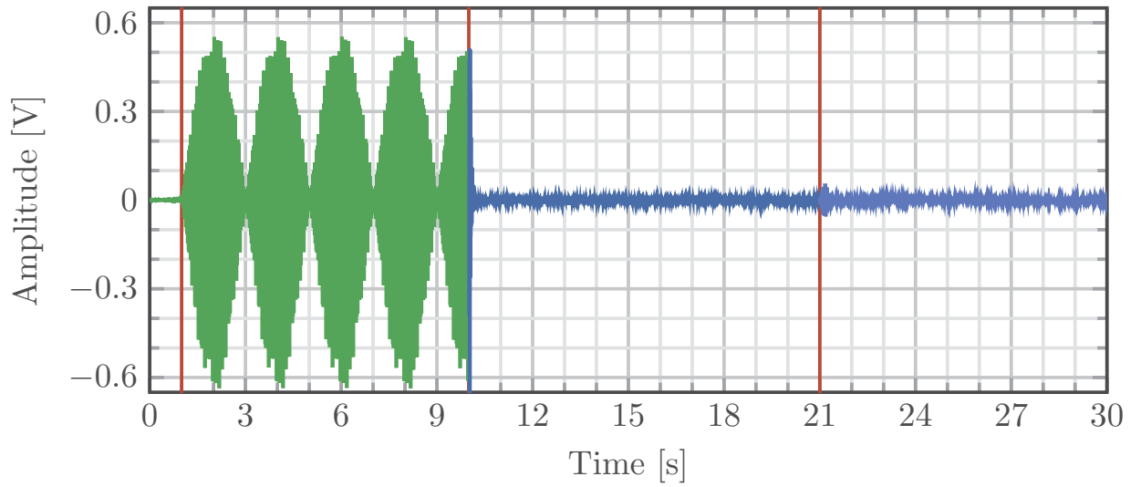
FIGURE 4.7. Acoustic interference attenuation using an adaptive controller with YK parametrization.
