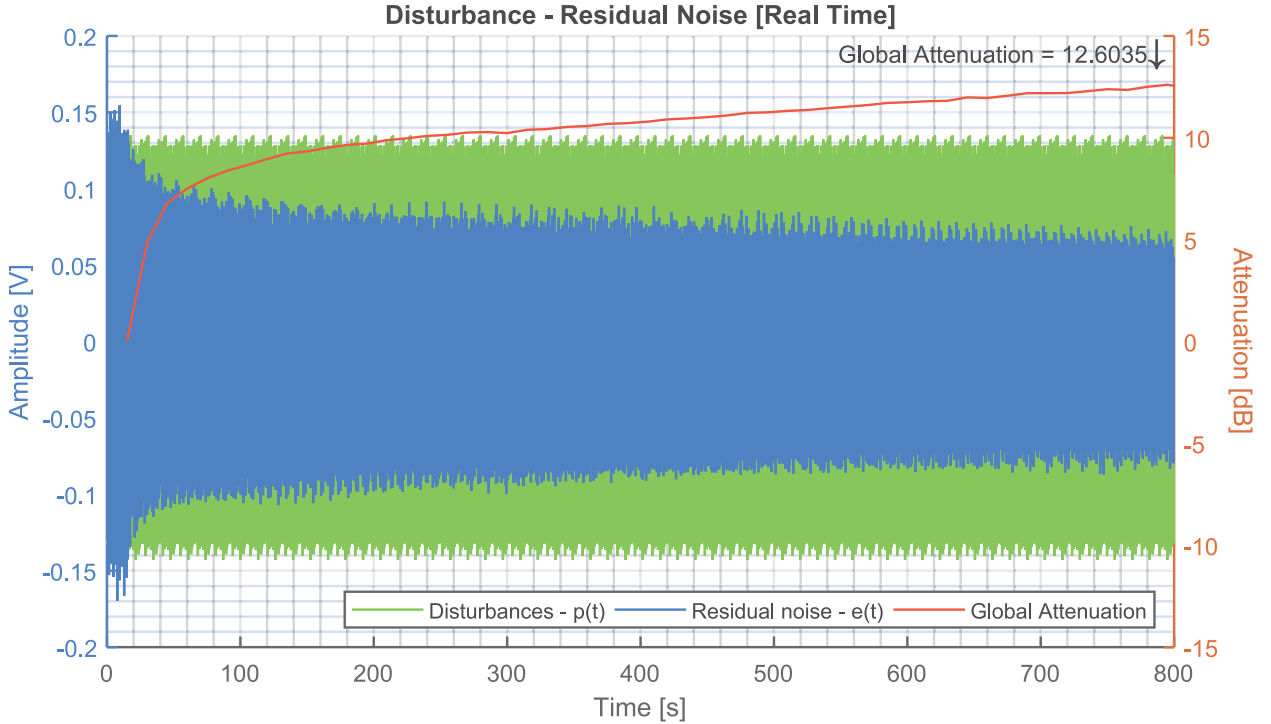
Figure 12: Performance of FUSBA FIR adaptive compensator (60 parameters, experimental).
