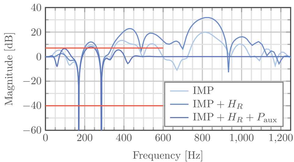
FIGURE 4.3. Evolution of the Output sensitivity function S_{yp} of a fixed linear controller.
