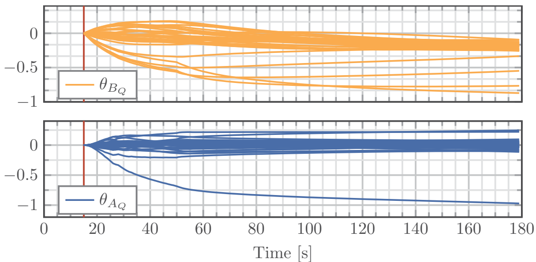
FIGURE 5.18. Filter Q(q^{-1}) = \frac{B_Q}{A_Q} parameters evolution for a [30/30] YK-IIR filter using FuSBA PAA with a constant trace profile. Compensation starts at 15 s.
