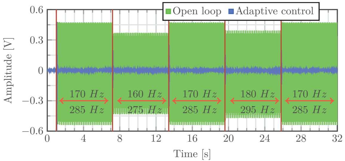
FIGURE 4.10. Step changes in frequencies using the adaptive controller with YK parametrization.
