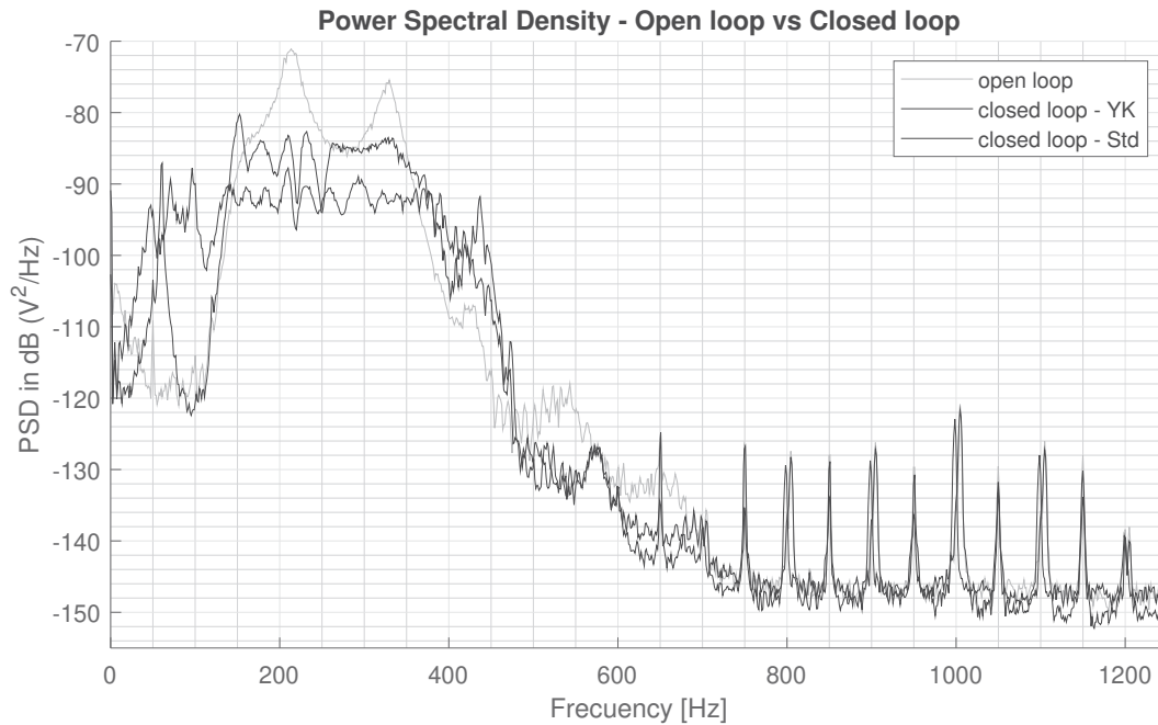
Figure 13: Power spectral density for FUSBA FIR and FUSBA YK FIR (60 parameters, experimental).
