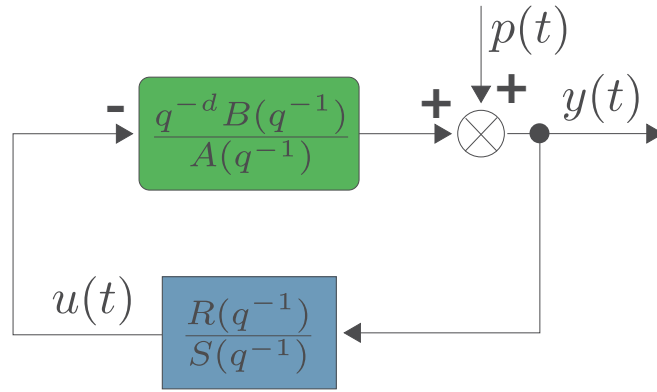
FIGURE 4.1. Feedback regulation scheme.
