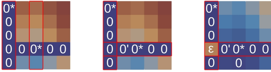
Figure 5.2 – Matrix reduction phase. Subtracting the minimum element from each of the n rows and columns might not be sufficient to make a set of n independent zeros appear. In the above example, initially detected independent zeros are first starred. All columns containing a 0^* are then covered (left). An uncovered zero which has a 0^* in its row is found and primed; its row is covered and the column of the 0^* is uncovered (center). At this point, all zeros are covered by construction. Let \epsilon be the smallest uncovered value. Add \epsilon to every covered row; subtract \epsilon from every uncovered column. This amounts to decreasing uncovered elements by \epsilon and increasing twice-covered elements by \epsilon . The sum of the elements of the matrix has been decreased and a new zero has appeared in an uncovered zone.
