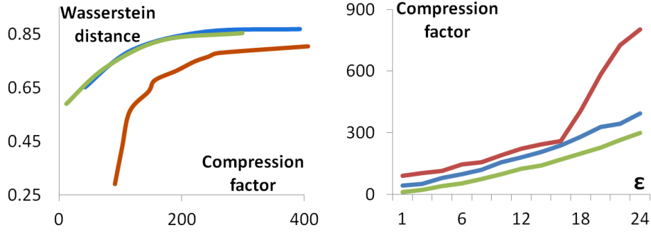
Figure 4.8 – Comparison to the SQ compressor [IKK12] (green: SQ-D, blue: SQ-R, red: our approach). Left: average normalized Wasserstein distance between the persistence diagrams of the input and decompressed data, for increasing compression rates. Right: average compression factors for increasing target persistence thresholds \epsilon .
