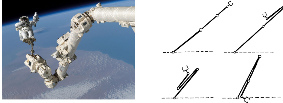
Figure 3.2 – A robotic arm (left, Canadarm2 [Nok07] - NASA 2005). Some degenerate configurations of a 3-arm (right, from [BHB84]), corresponding to critical points of the function giving the position of the end effector from the angles of joints.
