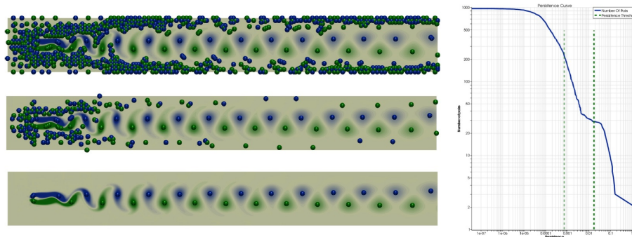
Figure 3.15 – Von Kármán Vortex street phenomenon, showing the turbulence of a fluid flow behind a solid obstacle [Tie16]. Extrema (spheres, blue: minima, green: maxima) of the the orthogonal component of the flow curl are shown (left). The persistence curve (right) shows populations of critical point pairs in the field; by selecting the most persistent ones (those on the right of vertical cuts of the curve), we can define a hierarchy of critical point sets (left, from top to bottom).
