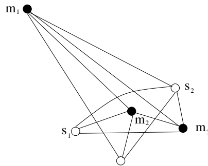
Figure 7.2: Edge Monitoring for K_6 - I .
