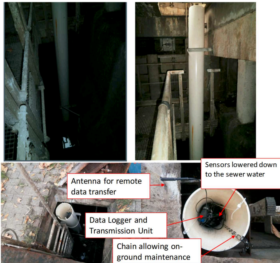
Figure 24. Location of sensors at Naujac (after Granger et al. , 2016).
