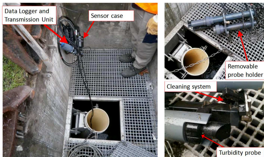
Figure 23. Installation of sensors and associated units at the CSO manhole at Peugue (after Granger et al. , 2016).
