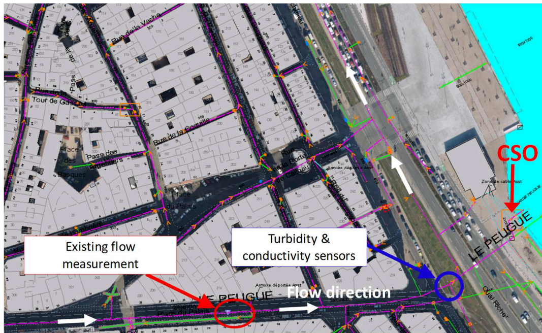
Figure 22. Location of sensors at Peugue (after Granger et al. , 2016).
