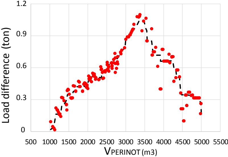
Figure 93. Impact of tank volume (Périnot tank, event 26 May 2016) on the difference in TSS load interception between QBR and HBR (black dotted line represents the moving median line with window width of ten values).
