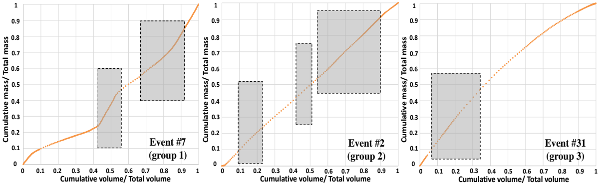
Figure 59. MV curves of the storm events #7 (left), #2 (middle), and #31 (right). Grey box indicates the filling periods of QBR.
