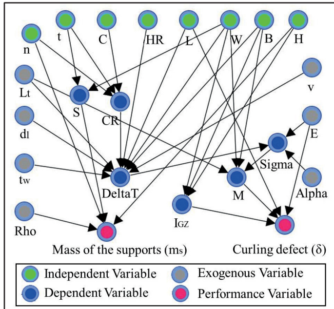
Figure 55. Causal graph for curling defect (represented in BayesiaLab)
