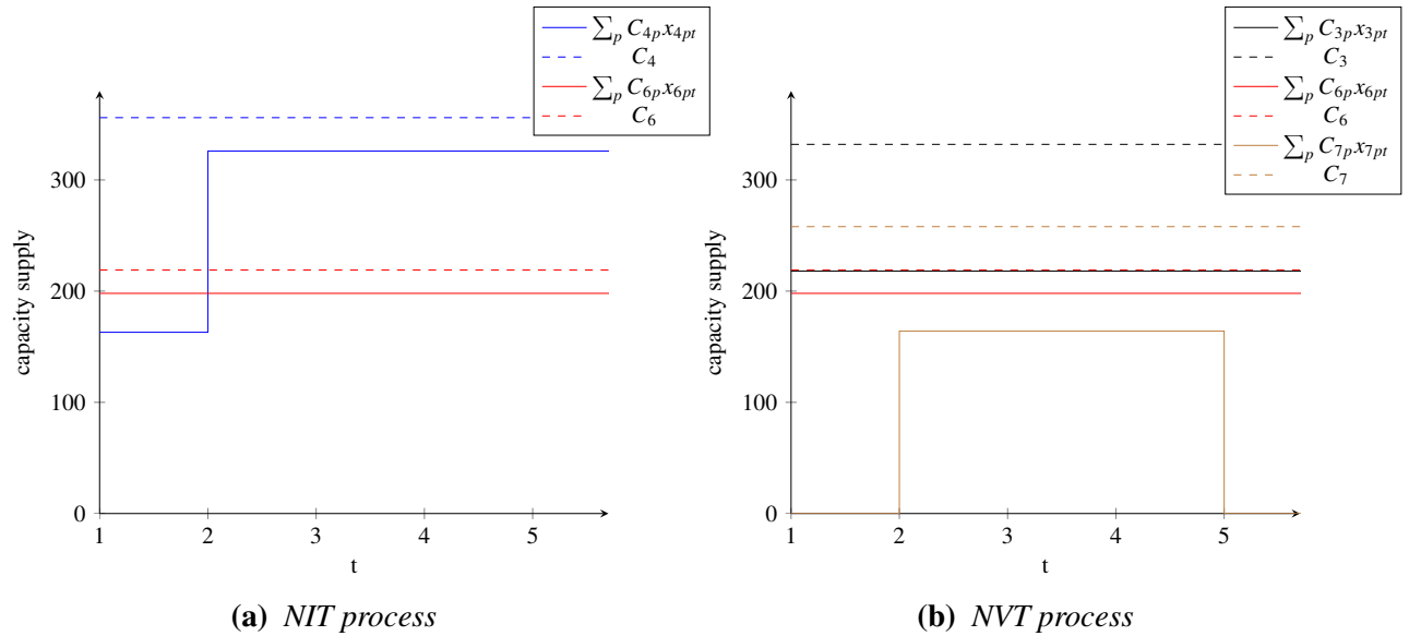
Figure 4.5: Capacity-allocation decisions from multi-period modeling approach versus the a priori capacity C_l for 5-4/8/20-25-(11,LT,TC,..)
