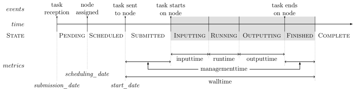
Figure 2.3: Tasks lifecycle
