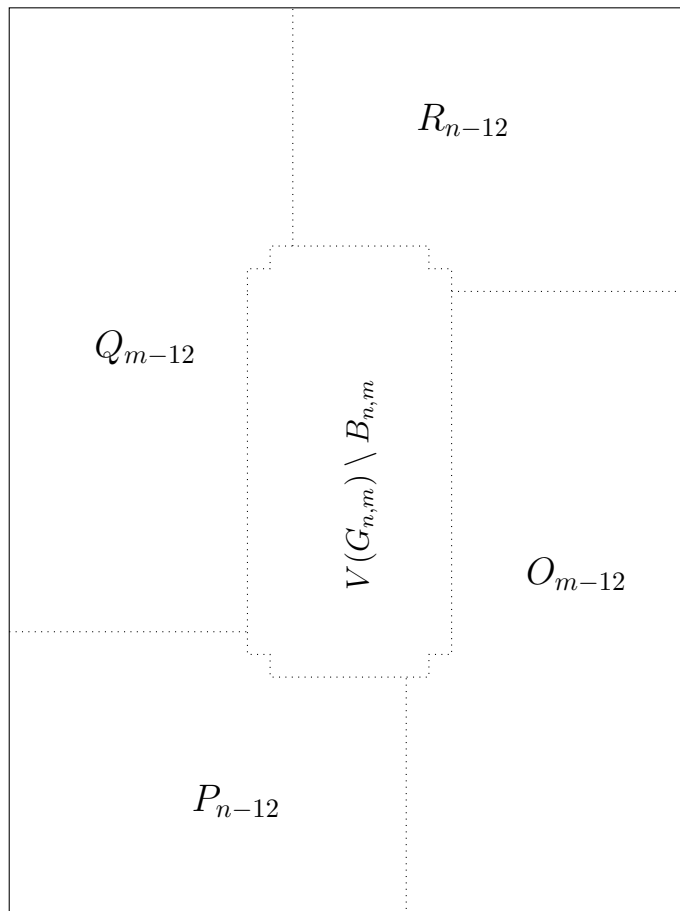
Figure 9.4 – The sets O_{m-12} , P_{n-12} , Q_{m-12} and R_{n-12} .
