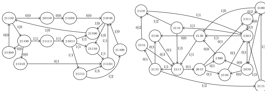
Figure 10.7 – \mathcal{T}_A , the union of s(\mathcal{T}_{10000}) (left) and s(\mathcal{T}_{1000}) (right).
