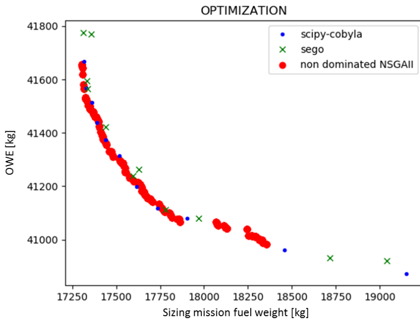
Figure 70: Pareto fronts obtained with the three optimization algorithm for Optimization 2
