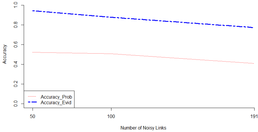
Figure 3.8: LFR: comparison of probabilistic and evidential accuracy: case of noisy links.
