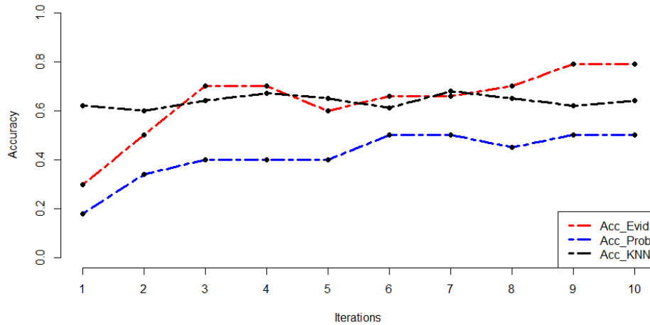
Figure 4.13: Accuracy Results: Case of PNCUPC .
