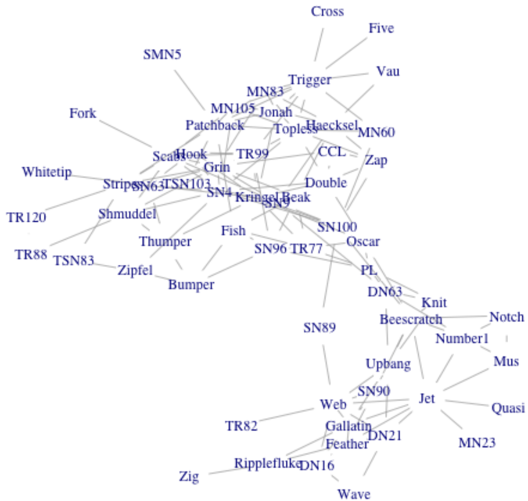
Figure 1.3: Dolphins Network.
