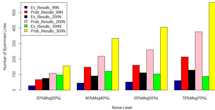
Figure 4.10: Spammed links after 10 iterations: case of noisy messages and links.
