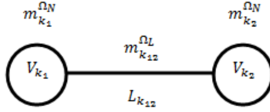
Figure 3.1: Triplet k .
