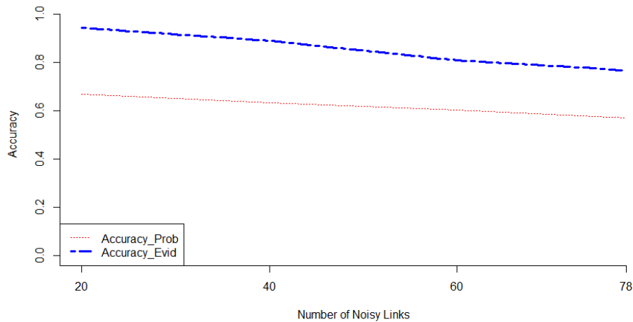
Figure 3.5: Karate Club: comparison of probabilistic and evidential accuracy: case of noisy links.
