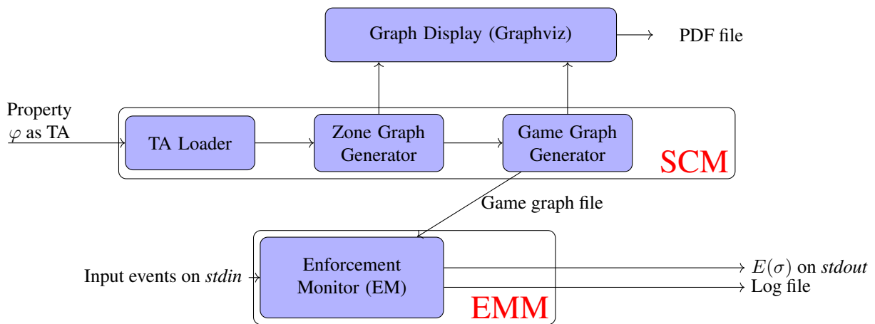
Figure 4.16 – Architecture globale de GREP
