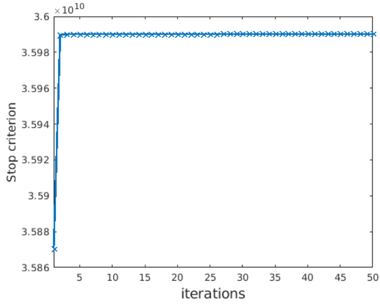
Figure 4.16: Convergence of JMAP for the joint reconstruction and segmentation of IQI volume from 300 projections
