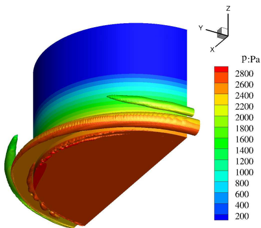
(a) foamStar 80x
