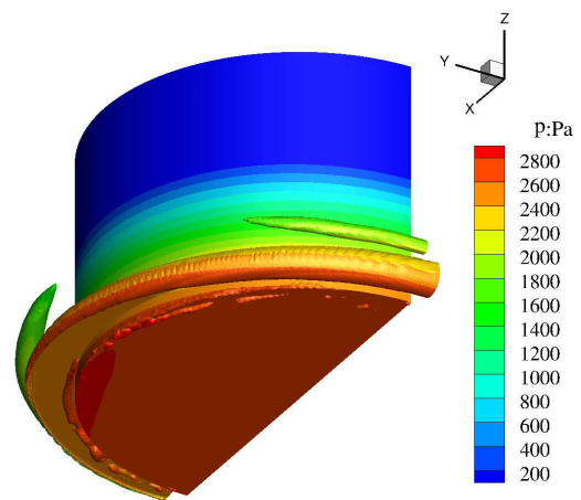
(b) foamStar-SWENSE 20x
