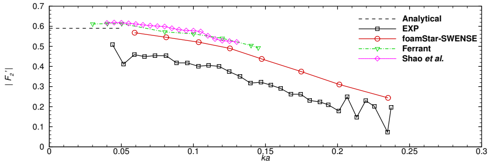
(c) Second harmonic amplitudes
