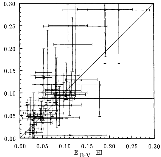
Fig. 5. Comparison between the total colour excesses E_{B-V}^{mod} computed from the extinction model at \tau = \tau_0 , and those read on maps of E_{B-V} built from HI distribution and deep galaxy counts from Burstein and Heiles. The ranges in galactic latitude are -45^\circ to -15^\circ and +15^\circ to +45^\circ .
