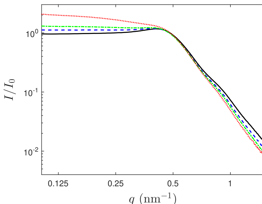
FIGURE 2.7: Intensity profiles for a sample dried at RH_c = 10\% with initial mass m_0 = 12.5 g. Measurements were taken 4 days (solid black line), 49 days (dashed blue line), 89 days (dash-dot green line) and 192 days (dotted red line) after the end of the drying. The effect of aging is visible as a increase of the scattered intensity at small q .
