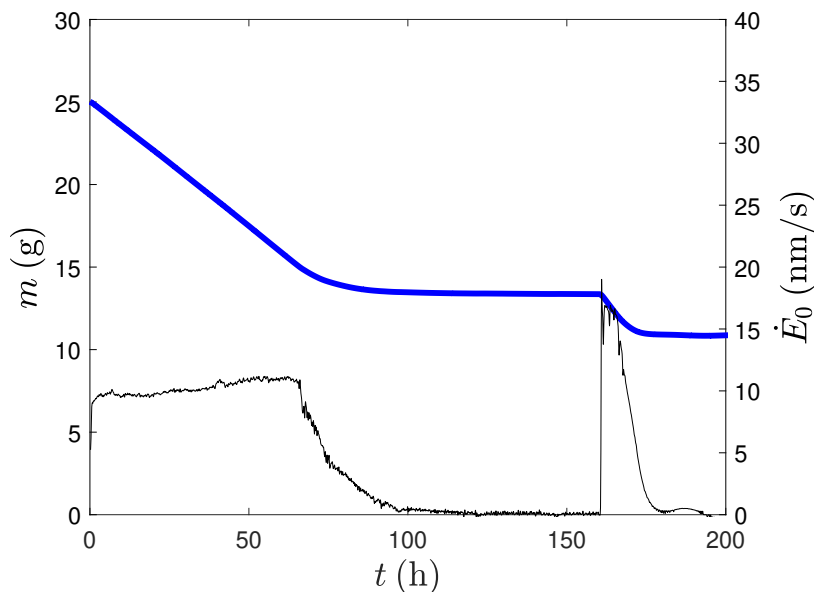
FIGURE 5.1: Drying experiment on a layer of HS-p suspension at \text{RH} = 80\% : mass m (thick blue line, left y-axis) and evaporation rate \dot{E}_0 (thin black line, right y-axis) as a function of time t .
