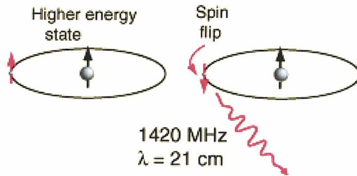
Figure 2.8: Hyperfine splitting of the hydrogen ground state
