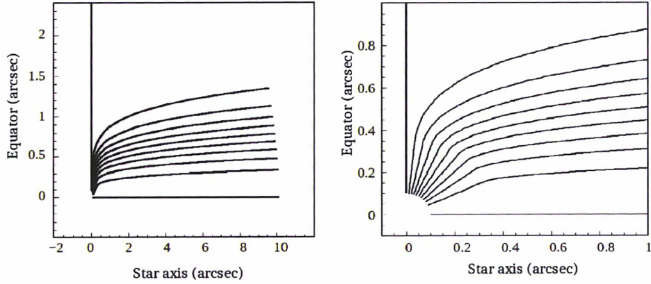
Figure 3.13: Meridian plane configuration of the molecular outflow for the model allowing for non-radial velocities. The curves are equally spaced in \gamma (steps of 0.1). The abscissa is the star axis, the ordinate on a radius along the equator, both in arcseconds. The right panel is a zoom of the left panel for r < 1'' .
