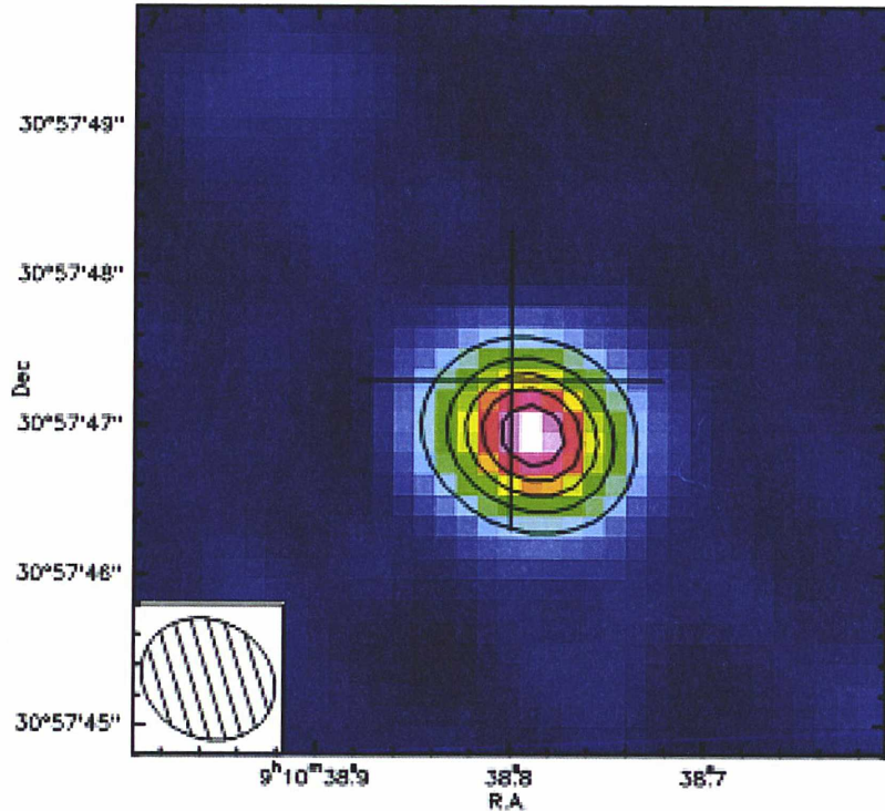
Figure 3.12: Continuum map at 115 GHz of RS Cnc (A+B configuration data obtained in 2011). The cross corresponds to the 2000.0 position of the star. The contour levels are separated by steps of 0.90 mJy/beam ( 20\sigma ).
