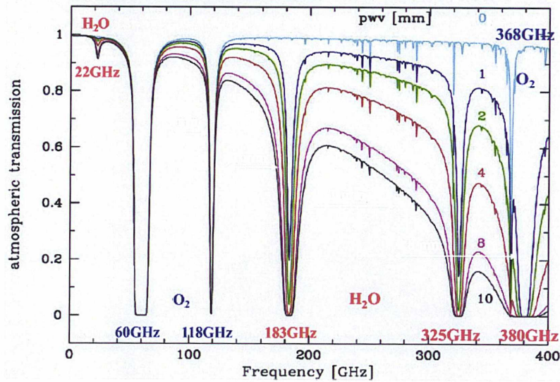
Figure 2.2: Dependence on frequency of the atmospheric transmission at PdBI (2550 m). The different transmission curves are calculated for the amounts of water vapour (in mm) given on the right.
