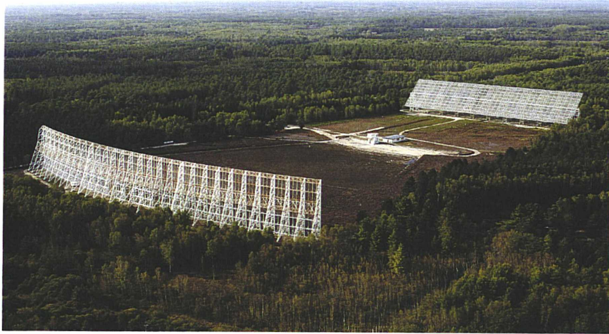
Figure 2.6: The Nançay (France) radio telescope. The tilting plane mirror in the background sends an image of the source to the fixed spherical mirror in the foreground. The mobile receiver system is visible between the two mirrors.
