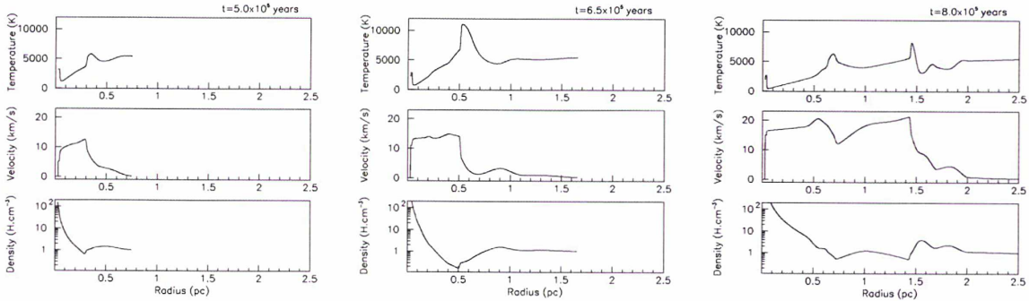
Figure 8. Density, velocity and temperature profiles for the Villaver et al. (2002) model (scenario 3) at three different epochs [ 5.0 \times 10^5 yr (left), 6.5 \times 10^5 yr (centre), 8.0 \times 10^5 yr (right)].
