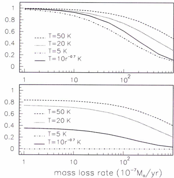
Figure 10. Ratio between the ‘estimated’ mass in atomic hydrogen and the real mass for the freely expanding wind case (scenario no. 1) with mass-loss rates ranging from 10^{-7} to 10^{-4} M_{\odot} \text{ yr}^{-1} (see Section 5.1) and different cases of temperature dependence (see text). Upper panel: no background. Lower panel: with a 5 K background.
