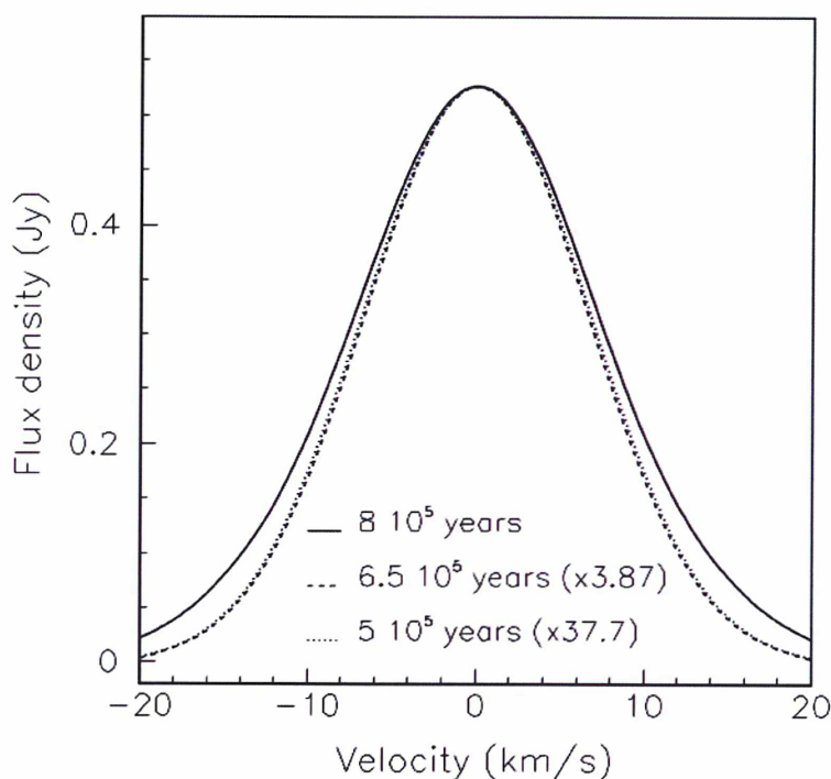
Figure 7.11: H I line profiles of a circumstellar shell model around a 1.5 M_{\odot} star during the evolution on the TP-AGB phase ( 5.0, 6.5, 8.0 \times 10^5 yr; Villaver et al. (2002), in the absence of background. The distance is set at 1000 pc. The first two profiles, scaled by up by factors of 37.7 and 3.87 respectively, in order to help the comparison, are virtually indistinguishable.
