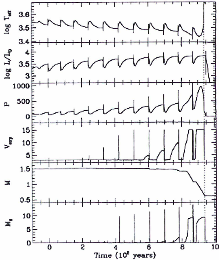
Figure 1.11: Time dependence (starting from the first TP) of various quantities during the TP-AGB phase of a star having a mass of 1.5 solar masses. The dotted line marks the end of the AGB phase. M_6 is the mass-loss rate in units of 10^{-6} solar masses per year (Vassiliadis & Wood 1993).
