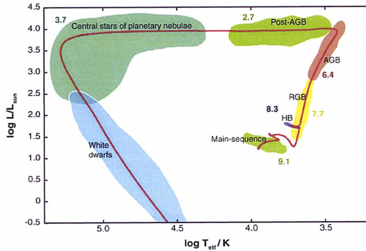
Figure 1.3: Evolution in the H-R diagram of a star having the metallicity of the Sun and twice its mass (Herwig 2005). The number labels for each evolutionary phase indicates the log of the approximate duration (in years).
