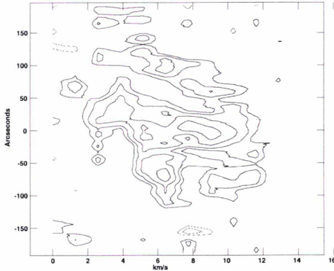
Fig. 15. H I position–velocity plot derived from naturally weighted data along PA = 10° and centered on the position of RS Cnc. Contour levels are (−5.6[absent], −4, −2.8, −2, 2...5.6) × 1.1 mJy beam −1 . The lowest contour level is \sim 2\sigma . The origin of the y -axis is the stellar position.
