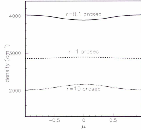
Fig. 6. Density profiles (in hydrogen atom number) in our preferred model as a function of \mu ( \equiv \sin \theta , \theta being the angle with respect to the equator) and for various distances from the central star. The profile for r = 1 \text{ arcsec} ( r = 0.1 \text{ arcsec} ) is scaled by a factor of 1/100 (1/10 000).
