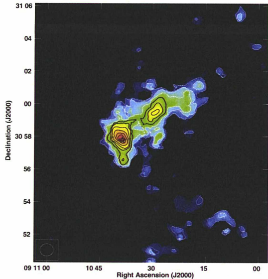
Fig. 13. H I total intensity map, derived from data with 6 k \lambda tapering (see Sect. 4.2). Contour levels are (1,2,3,\dots,9) \times 6.6 \text{ Jy beam}^{-1} \text{ m s}^{-1} . This image was derived by summing the emission over the velocity range from 2.6 \text{ km s}^{-1} to 11.6 \text{ km s}^{-1} ; to minimize the noise contribution to the map, data that did not exceed a 2\sigma threshold after smoothing the data spatially and spectrally by a factor of 3 were blanked. The star symbol marks the stellar position of RS Cnc.
