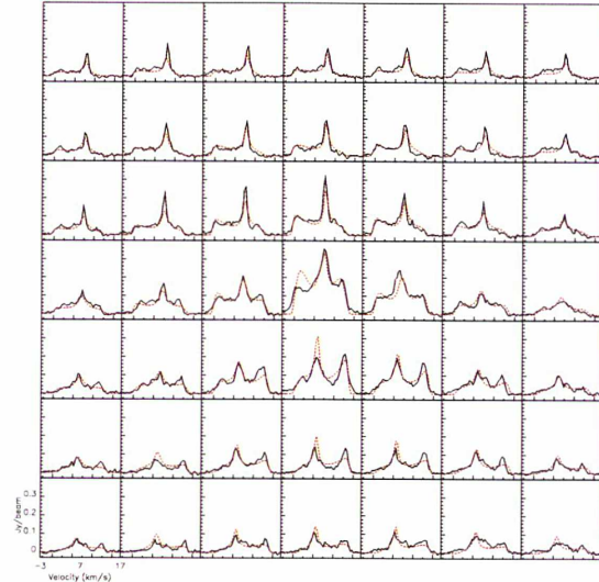
Fig. 10. Central part of the CO1–0 spectral map of RS Cnc together with the fits (dotted lines, in red in the electronic version) obtained in Sect. 3.2.
