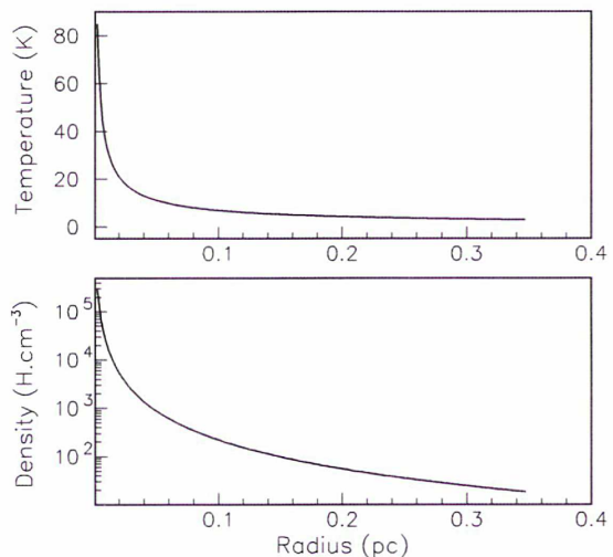
Figure 1. Density and temperature profiles for an outflow in uniform expansion (scenario 1, V_{\text{exp}} = 10 \text{ km s}^{-1} , \dot{M} = 10^{-5} M_{\odot} \text{ yr}^{-1} ).
