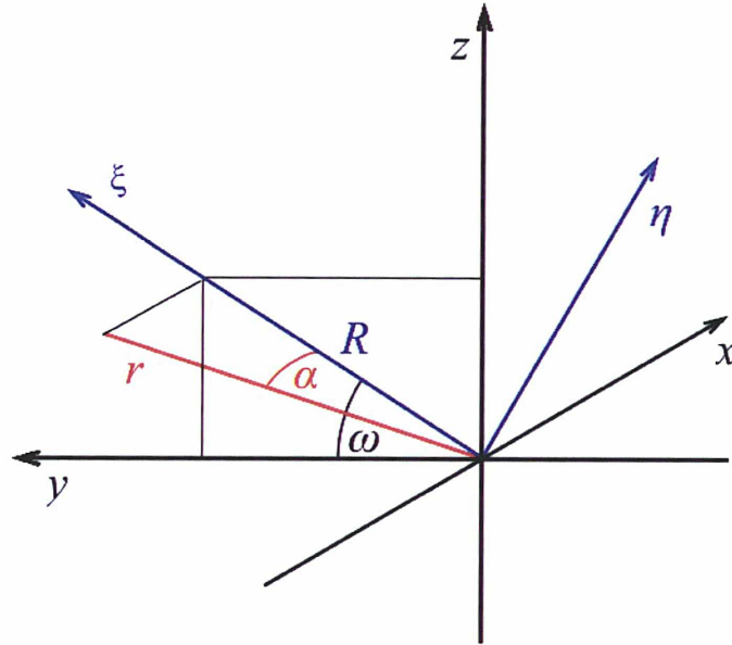
Figure 4.4: Definition of coordinates. The (\xi, \eta) coordinates are obtained from (y, z) coordinates by rotation of angle \omega in the sky plane about the x axis (line of sight and star axis, cf. Sect. 4.2). In the sky plane, y is towards East, and z towards North.
