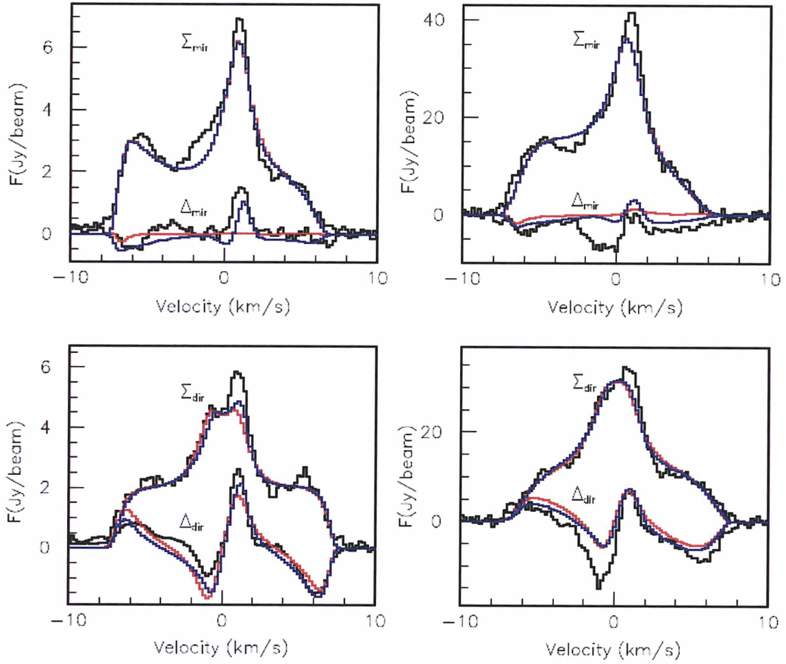
Figure 3.31: Velocity distributions of \Sigma_{dir} , \Delta_{dir} , \Sigma_{mir} , \Delta_{mir} , evaluated over the 24 pairs of diametrically opposite spectra of the CO(1-0) (left) and CO(2-1) (right) spectral maps. The upper panels are for mirror quantities and the lower panels for direct quantities. In each case, the data are shown in black, the best fit results of the standard model in red and of its modified asymmetric version in blue. The reference velocity is 7.25 \text{ km s}^{-1} , the CO(1-0) data of Libert et al. (2010b) and Hoai et al. (2014) having been corrected by +0.5 \text{ km s}^{-1} .
