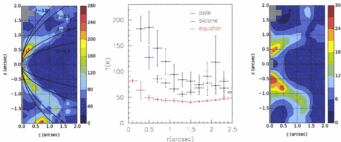
Figure 5.11: Left: Map of temperatures in the half-meridian plane of the star obtained from the effective densities using Relation 4. The parabolas are for \beta=0.3 , 0.8 , 2.5 and 3.5 and define the sectors illustrated in the central panel. Middle: r -distribution of the gas temperature averaged over the three angular sectors delineated in the left panel: the red points are for the equatorial region (inside the \beta = 0.3 parabola), the black points are on the bicone (between the \beta = 0.8 and \beta = 2.5 parabolas) and the blue points are for the polar region (outside the \beta = 3.5 parabola). Error bars show the dispersion within each r bin. Right: CO density (in molecules per \text{cm}^3 ) multiplied by r^2 (in \text{arcsec}^2 ).
