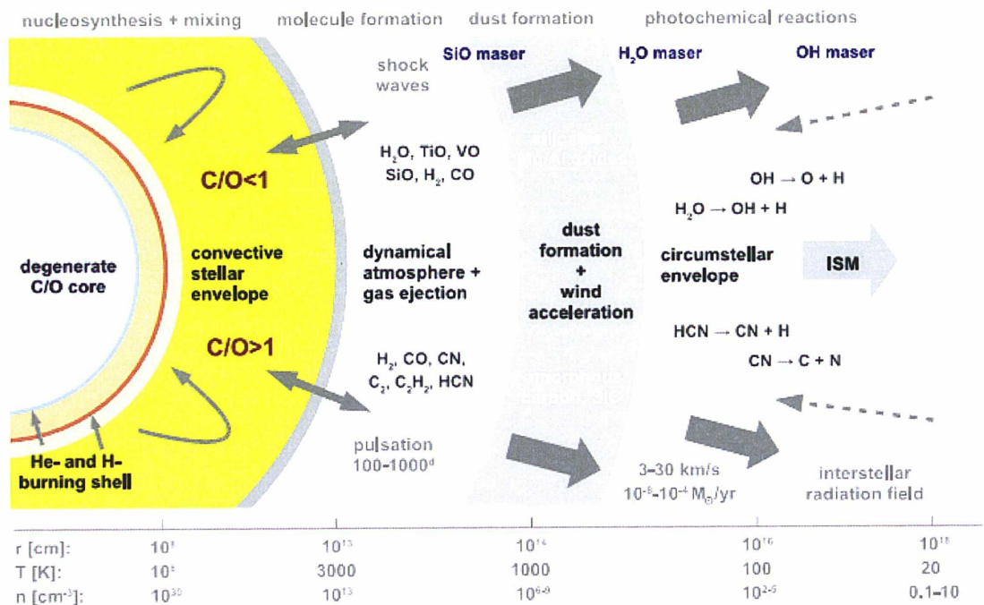
Figure 1.1: Sketch of the structure and environment of an AGB star (with the original idea from Le Bertre 1997).
