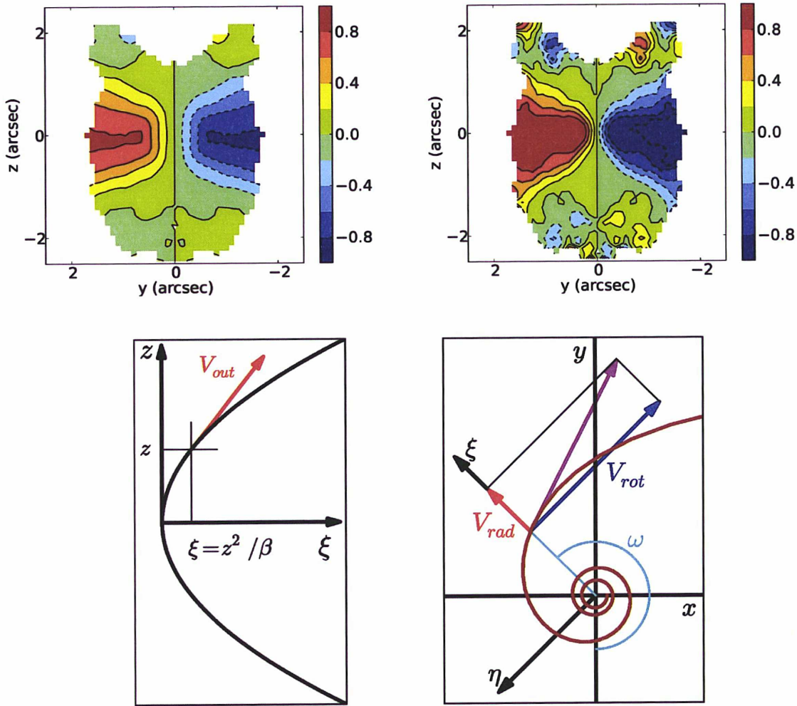
Figure 3: Red Rectangle. Upper panels: Sky maps of the east-west asymmetry of the Doppler velocity for CO(3-2) (left) and CO(6-5) (right). Lower panels: Gas velocity. Left: in the polar region (in the meridian plane of the star); Right: in the equatorial region (in the equatorial plane of the star).
