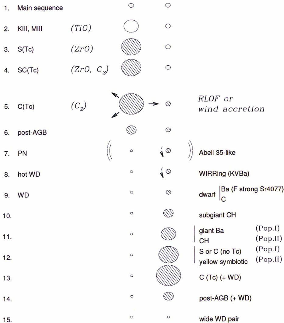
Figure 1.13: Schematic evolution of close binaries (Jorissen 2004).
