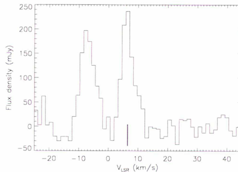
Fig. 14. Spatially integrated H I spectrum of RS Cnc derived from naturally weighted (J)VLA C+D configuration data. The vertical bar indicates the stellar systemic velocity derived from CO observations. The spectral feature centered near the stellar systemic velocity is circumstellar in origin, while the second peak near V_{\text{LSR}} = -7 \text{ km s}^{-1} results from interstellar contamination within the measurement aperture.
