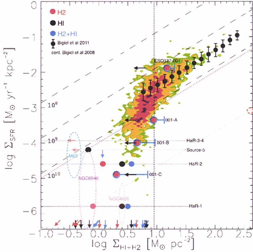
Fig. 4. K-S relation for sources in Table 4, with filled circles and arrows for values and upper limits respectively. Red markers consider only H_2 for \Sigma_{\text{gas}} , black ones only HI, and blue ones the sum of both. Figure adapted from Jáchym et al. (2014), where their sources ESO137-001, 001-A, 001-B and 001-C have been plotted in a similar way than ours: red circles for H_2 gas, black left arrows for HI upper limits, and blue "error bars" to account for both gas components. Colored contours account for the spiral galaxies from Bigiel et al. (2008) (green, orange, red and purple for 1, 2, 5 and 10 sampling points per 0.05 dex respectively). Black markers with error bars correspond to the running medians in \Sigma_{\text{SFR}} as a function of \sigma_{H_2} of 30 nearby galaxies from Bigiel et al. (2011). Shaded ovals represent the data from the outer parts of XUV disk galaxies: NGC4625 and NGC6946 from Watson et al. (2014) (priv. communication), and M63 (NGC5055) from Dessauges-Zavadsky et al. (2014), taking only H_2 into account in all of them. The dashed vertical line shows the 9 M_{\odot} \text{pc}^{-2} threshold at which the atomic gas saturates. Dashed inclined lines represent "isochrones" of constant star formation efficiencies, indicating the depletion times \tau_{\text{dep}} of 10^8 , 10^9 and 10^{10} years to consume all the gas. The dashed red isochrone marks a depletion time equal to the age of the universe, as one Hubble time (13.8 Gyr). A representative shift of the HaR-1 marker for \Sigma_{H_2} is drawn, to show the "effective" molecular gas density at which stars would formed in this region if we consider a beam correction factor of +2.68 in log space, to convert our 22" beam to a \sim 1'' beam as in the H_{\alpha} data.
