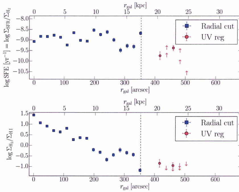
Figure 2.9: Radial profiles of the star formation efficiency (upper panel) and the H 2 -to-HI surface density ratio (bottom panel). The SFE is defined here as the star formation rate per unit of molecular gas. The blue squares correspond to the 17 pointings done to map CO along the M63 major axis (the radial cut) out to the isophotal radius, r_{25} (dashed line), and the red circles correspond to the 8 pointings with 24 \mu\text{m} emission detection done to map CO over the bright UV region at r_{\text{gal}} = 1.36 r_{25} . The double data points plotted for the UV region at each r_{\text{gal}} correspond to the parallel pointings used to map this region (see Table 2.2).
