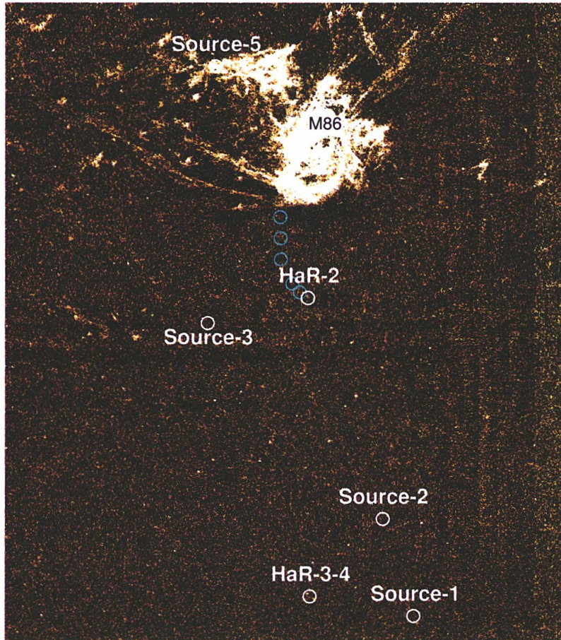
Figure 3.6: H\alpha + [NII] map of the Virgo cluster from Kenney et al. (2008) taken with the KPNO telescope. Our sources are marked in the same way as in Figure 3.2. Circles in this image are 22'' width, but the aperture photometry was done in a 1'' aperture, to be consistent with the H\alpha data from Yagi et al. (2013). This map was calibrated with Yagi's data and used to calculate the L_\alpha of Source-5, as well as the upper limits for Source-1, Source-2, Source-3, HaR-2-1, HaR-2-2, HaR-2-3 and HaR-2-4 from the map's noise level.
