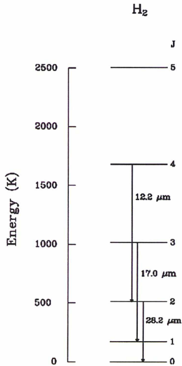
Figure 1.1: \text{H}_2 energy levels diagram
