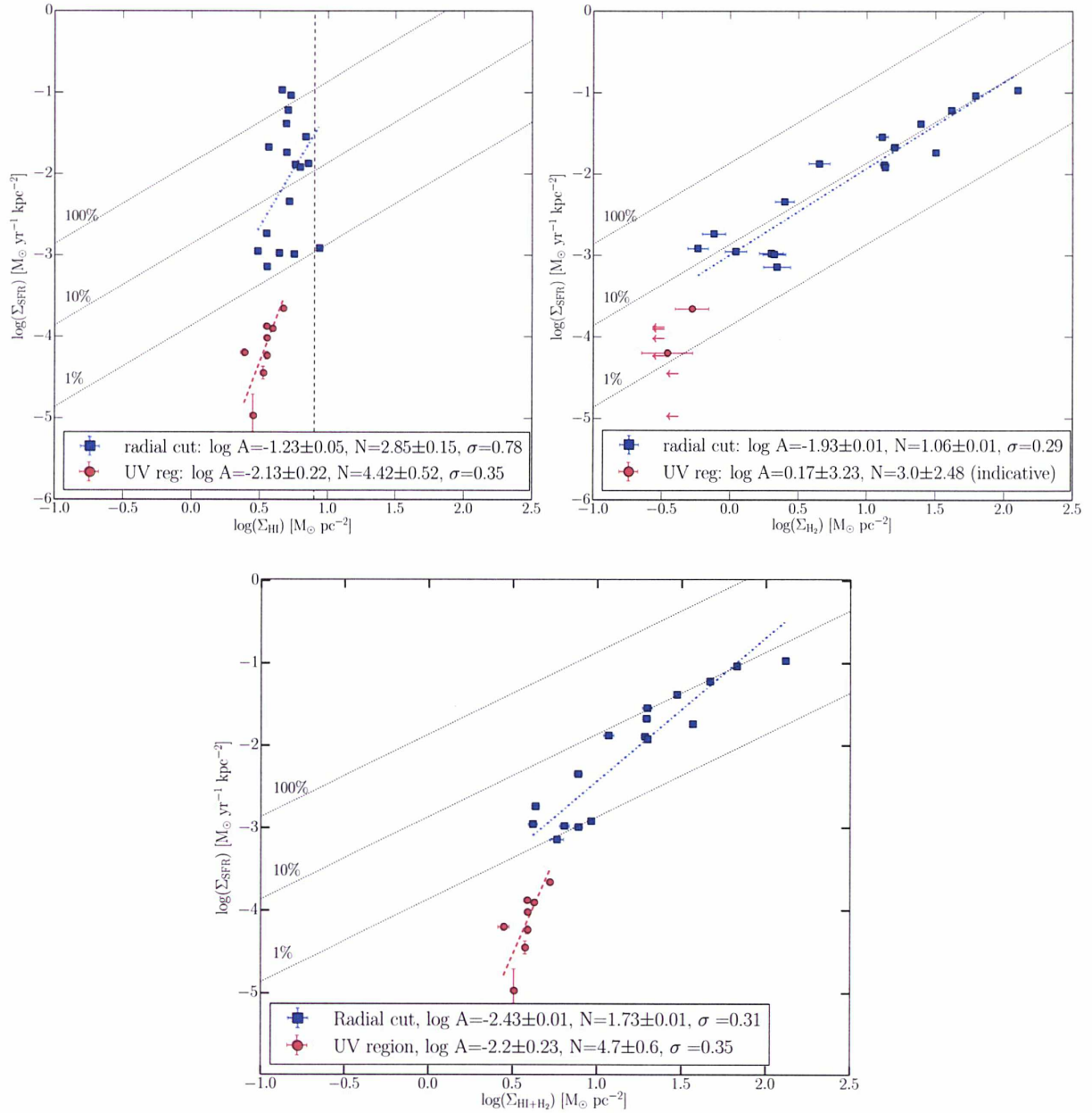
Fig. 7. Kennicutt-Schmidt relations that relate the SFR surface density to the gas surface density plotted for \Sigma_{\text{H I}} (top-left panel), \Sigma_{\text{H}_2} (top-right panel), and \Sigma_{\text{H I}+\text{H}_2} (bottom panel). The blue squares correspond to the 17 pointings used to map CO along the M63 major axis (the radial cut) out to the isophotal radius, r_{25} , and the red circles correspond to the 8 pointings with 24 \mu\text{m} emission detection used to map CO over the bright UV region at r_{\text{gal}} = 1.36 r_{25} . The K-S relation is best parametrized by a power law of the form \Sigma_{\text{SFR}} = A(\Sigma_{\text{gas}})^N , which in log space translates into a linear relation. The best-fitting bisector linear K-S relations are derived separately for the radial cut (blue dashed-dotted lines) and for the UV region (red dashed lines). The corresponding coefficients \log A and slopes N can be found in the labels of each panel. The black dotted lines represent “isochrones” of constant star formation efficiencies, indicating the level of \Sigma_{\text{SFR}} needed to consume 100%, 10%, and 1% of the total amount of gas within 10^8 years. The vertical dashed line in the top-left panel corresponds to the \Sigma_{\text{H I}} \sim 9 \text{ M}_{\odot} \text{ pc}^{-2} threshold at which the atomic gas saturates (Bigiel et al. 2008).
