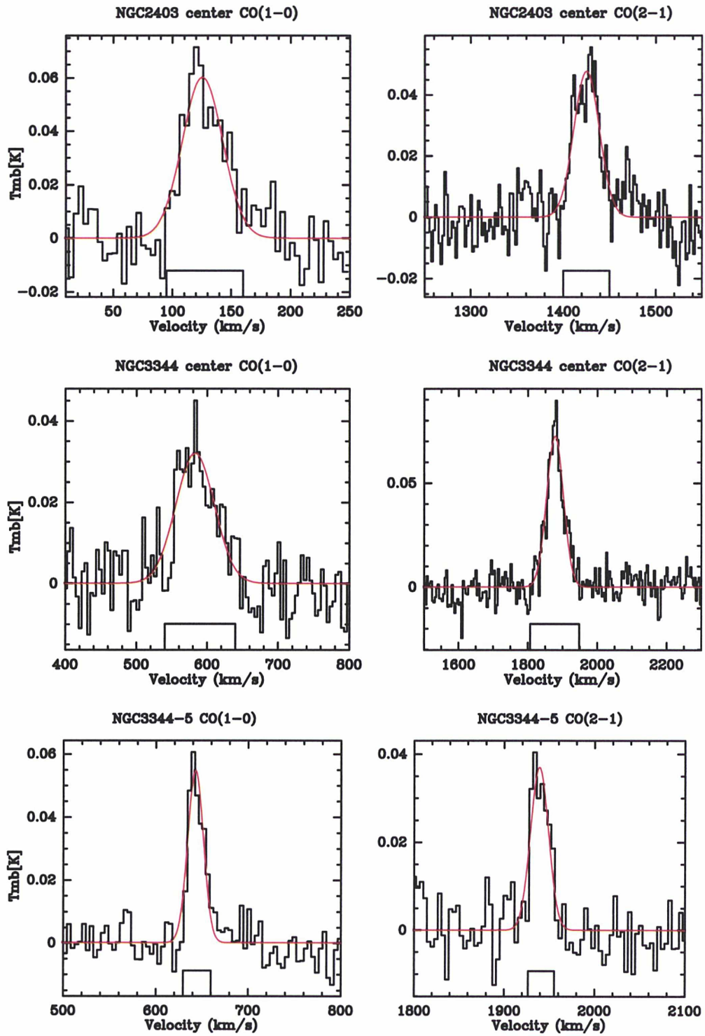
Figure 2.14: Spectra results for XUV observations 2013.
