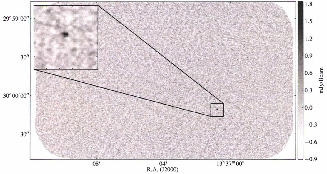
Figure 2.21: Continuum map of M83 with a weak detection on a point source ( <2\text{mJy} ). The rms of the map is 0.19 mJy.
