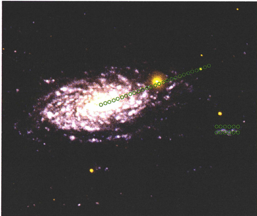
Figure 2.2: Positions of observing pointings to map the radial axis of M63, as well as its bright UV region, overlaid in the same NUV-FUV composite image of Figure 2.18. Mapping CO through individual beam pointings, has proven to be a very efficient technique to obtain deep observations of specific, not extended areas of a galaxy. To better visualize the spatial resolution of our data, pointings circles have been drawn with a 11'' width, same as the CO(2-1) FWHM.
