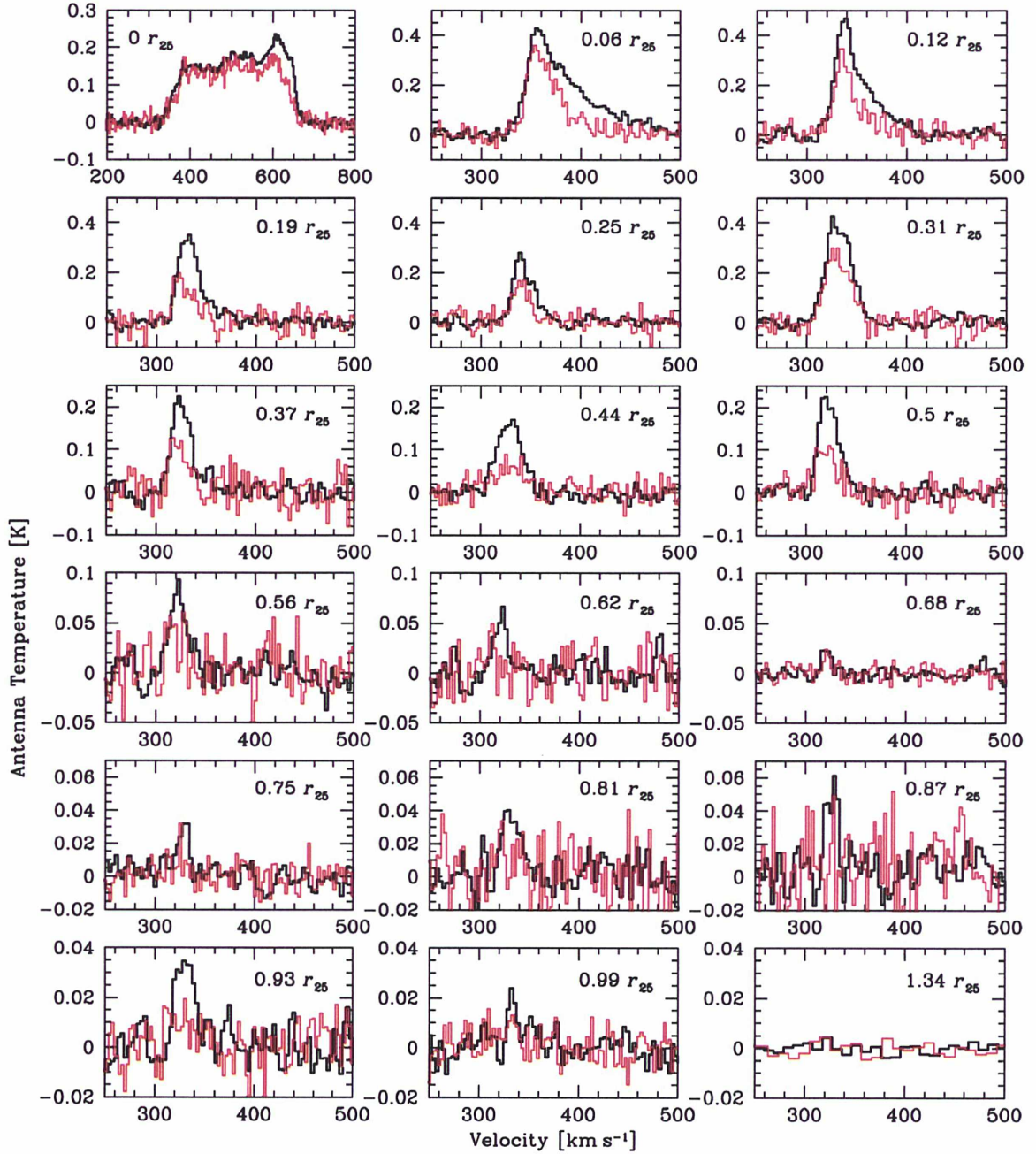
Fig. 2. Mosaic of CO spectra obtained when mapping the M63 disk along its major axis from the center of the galaxy out to the isophotal radius, r_{25} . The CO(2–1) spectra (red thin line) are overplotted on the CO(1–0) spectra (black thick line). While CO(1–0) is clearly detected up to the optical radius, CO(2–1) appears to be confined to r_{\text{gal}} \lesssim 0.68 r_{25} . The bottom right hand panel shows the CO(1–0) and CO(2–1) spectra obtained when summing all scans at the ten outermost pointings from r_{\text{gal}} = 1.06 r_{25} to 1.6 r_{25} and smoothed to a resolution of 9.7 \text{ km s}^{-1} and 10.4 \text{ km s}^{-1} , respectively. No CO emission is detected at these outermost pointings.
