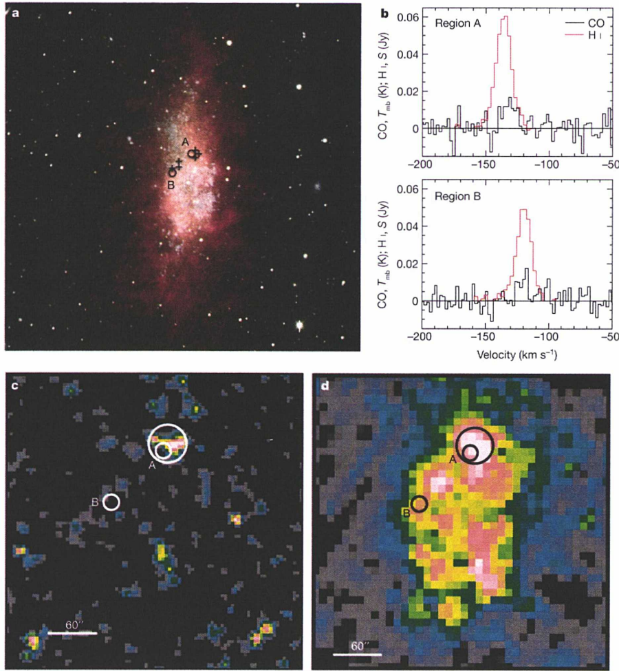
Figure 1 | Observations of the galaxy WLM. WLM is a small, gas-rich galaxy 985 \pm 33 kpc from the Milky Way 1 . It contains 1.6 \times 10^7 M_{\odot} of stars 28 , compared with (6.4 \pm 0.6) \times 10^{10} M_{\odot} in the Milky Way 29 , and it forms new stars at a rate 23 of 0.006 M_{\odot} \text{ yr}^{-1} , which is 12 times higher per unit stellar mass than the Milky Way 30 . a , Colour composite image: red, H I; green, V band; blue, GALEX far-ultraviolet. For H I the aperture was 7.6'' and the resolution was 2.6 \text{ km s}^{-1} , and for CO(3–2) the aperture was 18'' (circles) and the resolution was 0.11 \text{ km s}^{-1} , although the CO(3–2) spectra shown in the figure were smoothed to a resolution of 2.2 \text{ km s}^{-1} . The CO detections are labelled; their exposure times were 218 min (region A) and 248 min (region B). Other regions searched with exposure times shorter by factors of \sim 2 to \sim 6 are indicated by plus signs; the presence of comparable CO mass in some of these other regions cannot be ruled out. b , Spectra of the two detections: velocities are relative to the local standard of rest; CO labels main-beam brightness temperature, T_{\text{mb}} , in kelvin; H I labels flux in Jy. c , False-colour image of the 870\text{-}\mu\text{m} observations made with LABOCA on APEX. d , False-colour Spitzer 160\text{-}\mu\text{m} image obtained from Spitzer archives. In c and d , the images show the same field of view and the small circles ( 22'' diameter, the resolution of LABOCA) show where CO was detected. The large circle is 45'' in diameter and surrounds a large H I and FIR cloud (region A1) where the dust temperature was measured.
