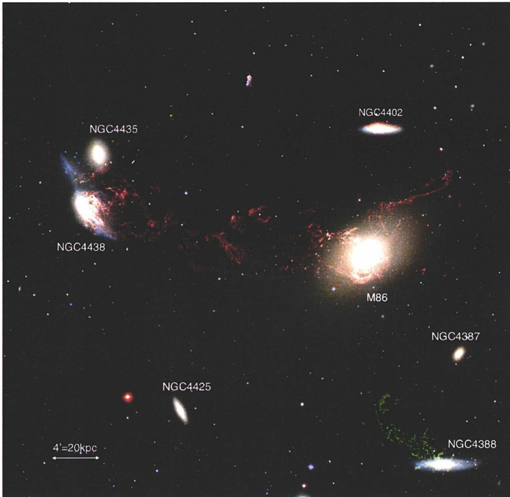
Figure 3.1: H \alpha + NII image of the Virgo cluster from Kenney et al. (2008). In red: low velocity emission <500 km/s. In green: high velocity emission >2000 km/s.
