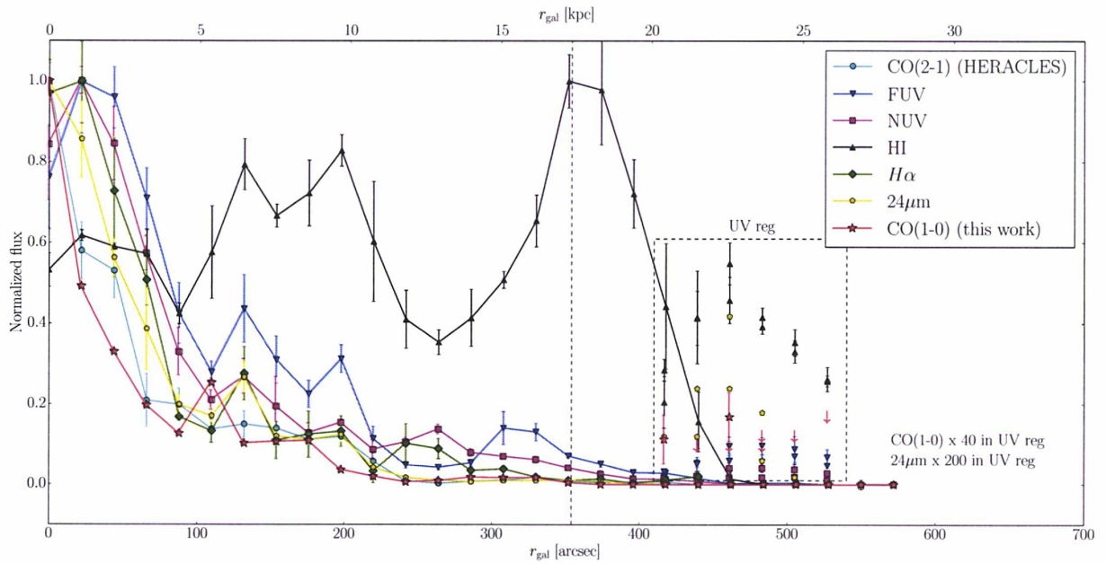
Fig. 5. Radial profiles of FUV, NUV, H\alpha , 24 \mu\text{m} , different star formation tracers, and HI taken from the literature (see Table 3), as measured along the major axis of the M 63 disk, which we compare to our CO(1–0) radial profile (red stars) and to the CO(2–1) radial profile from the HERACLES survey (Leroy et al. 2009). The measured fluxes are plotted in a normalized flux scale in order to allow relative comparisons. All the star formation tracers nicely follow the spiral arm structure at r_{\text{gal}} \approx 130, 200 , and probably 260'' . We observe a severe drop with the galactocentric radius for all star formation tracers, as well as for CO, such that close to the r_{25} limit (dashed line) and beyond all tracers and CO are practically absent with the exception of UV and HI. The CO emission is again detected in the external bright UV region. The measurements obtained in this UV region are shown in the dashed box at the correct galactocentric radii. The CO(1–0) and 24 \mu\text{m} fluxes are multiplied by a factor of 40 and 200, respectively, to make them visible. The double data points plotted at each r_{\text{gal}} correspond to the parallel pointings used to map the UV region (see Table 2). This external UV region has relatively high FUV and NUV emissions and is dominated by HI.
