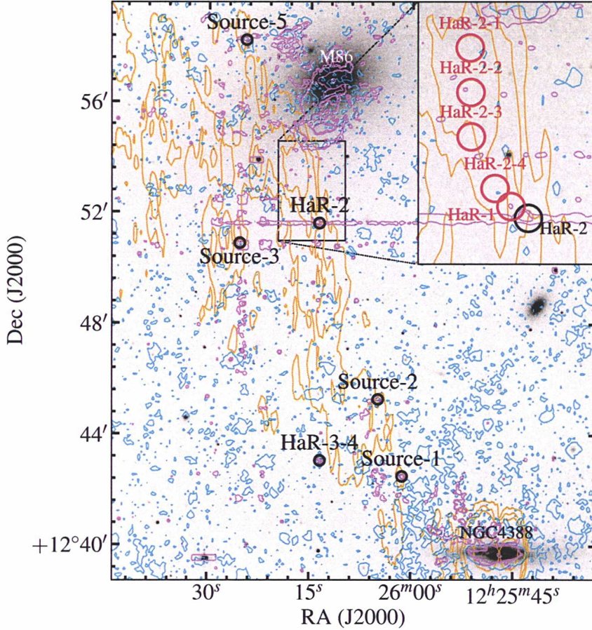
Fig. 1. Targets observed in the Virgo Cluster. Orange: HI contours levels at 1, 5, 10 and 50 \times 10^{19} \text{cm}^{-2} from Oosterloo & van Gorkom (2005). Purple: H \alpha contours levels at 5, 11 and 50 e^-/\text{sec} (Kenney et al. 2008). Cyan: 250\mu\text{m} contour levels at 0.01 and 0.1 Jy/beam (Davies et al. 2012). In zoomed regions: targets selected close to HaR-2 for run 075-14 (red circles). Circles enclosing targets are 22'' width, as the CO(1–0) HPBW.
