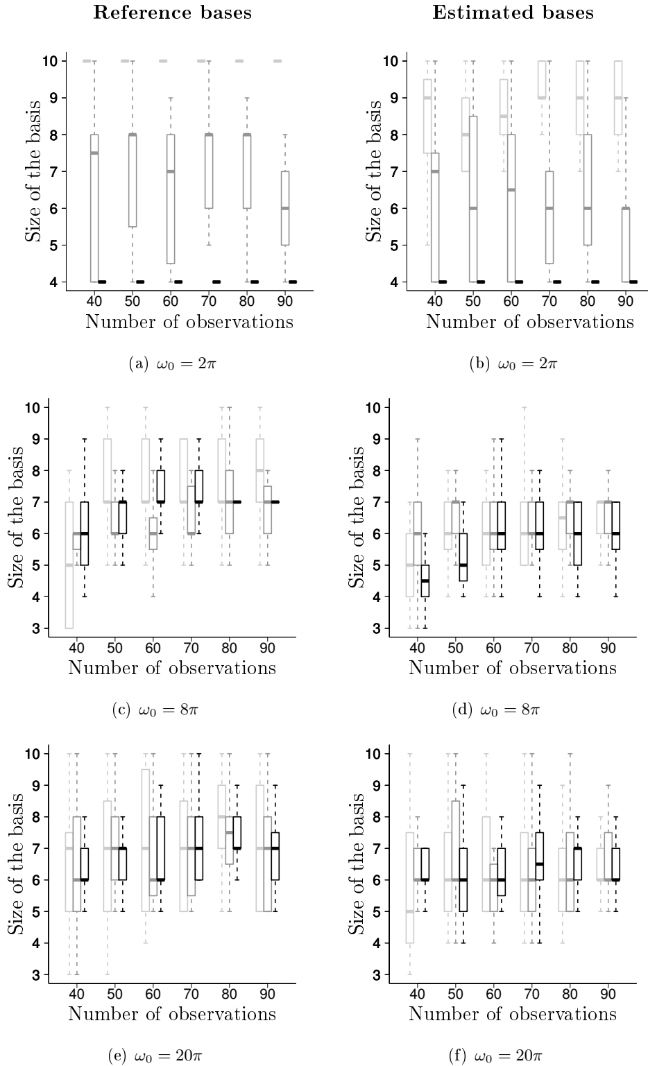
Figure 5.6: First numerical example: Sizes of the projection bases estimated with the Leave One Out criterion of Eq. (5.3.23). The observations are independently drawn according to \mu_{X_1} \times \mu_{X_2} and the designs are of increasing size. Three types of projection functions r_m are considered. The first one is based on Principal Components Analysis (light grey), the second one is based on PLS regression (mid-grey) and the third one is based on the projection of Proposition 5.2.1 with a linear model of the form L(\mathbf{a}^*)\mathbf{y}_1 where \mathbf{a}^* is given by Eqs. (5.5.5) and (5.5.8) (black). The study has been restricted to 1 \leq m \leq 10 . The reference bases are computed from a set of 1000 observations of the functional input and output of the second code. The estimated bases are estimated from the observations of the designs.
