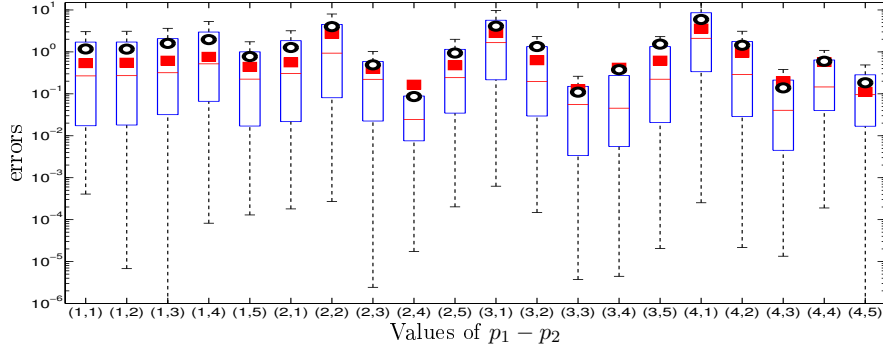
(a) Case 1: \hat{\epsilon}_{\text{LOO}}
