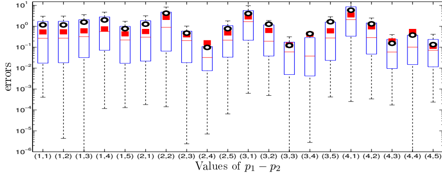
(b) Case 2: \tilde{\epsilon}_{\text{LOO}}
