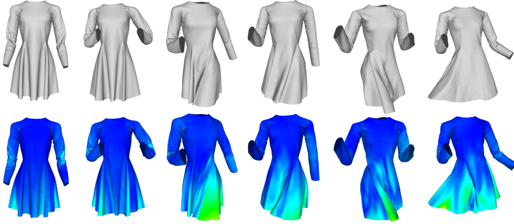
Figure 5.7 – Comparison to ground truth. First row: our predicted clothing deformation. Second row: ground truth colored with per-vertex error. Blue = 0cm, red = 10cm.
