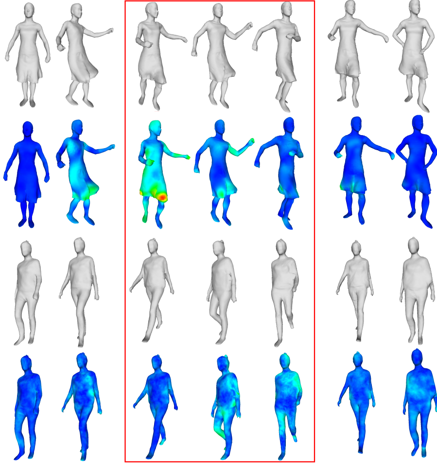
Figure 5.4 – Example frames from two sequences showing the reconstruction based on trained neural network. The first and the third row show the reconstruction and the second and the forth show the corresponding vertex error on ground truth meshes. The three columns in the red box are predictions from testing frames; others are from training frames. Dark blue = 0 millimeters, bright red \geq 5 millimeters.
