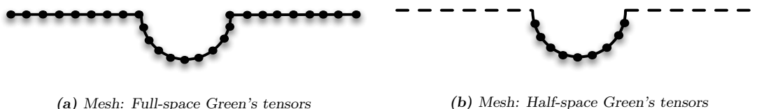
(a) Mesh: Full-space Green's tensors
