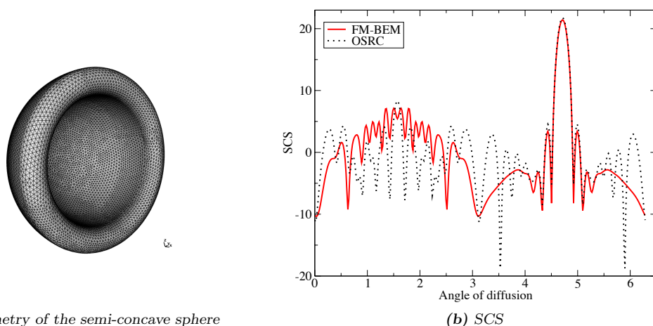
Figure 3.3: Diffraction of incident plane P-waves by a semi concave sphere ( \kappa_s = 8\pi ).
