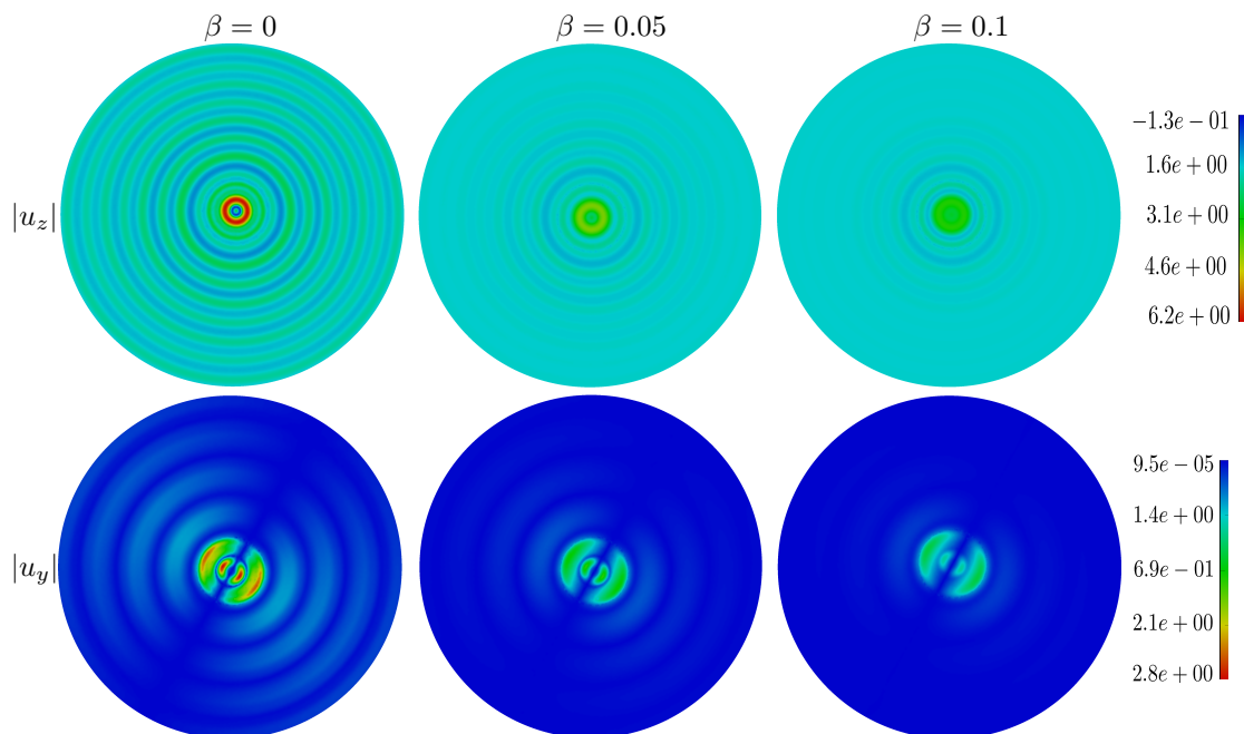
Figure 1.6: Vertically incident P-wave in a viscoelastic half-space containing a semi-spherical soft basin: contour maps of |u_z| and |u_y| at \kappa_P^{(1)} R/\pi = 2 for three levels of damping in both media ( \beta_1 = \beta_2 = \beta ): \beta = 0 (purely elastic case), \beta = 0.05 and \beta = 0.1 ; from [9].
