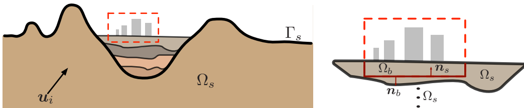
Figure 1.11: FEM-BEM coupling: notations.
