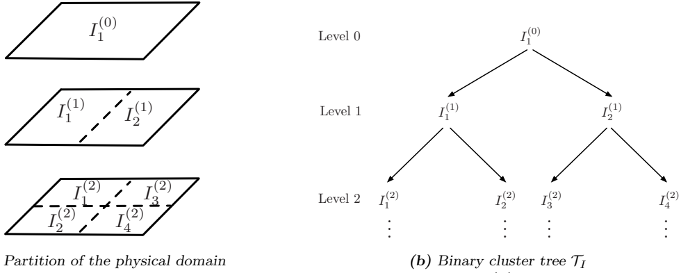
Figure 4.3: Illustration of the clustering of the degrees of freedom: (a) partition of the degrees of freedom in the domain and (b) corresponding binary tree.
