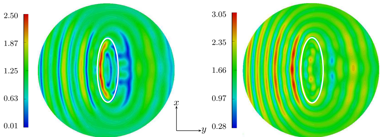
Figure 1.3: Diffraction of an oblique incident plane P-wave by a semi-ellipsoidal canyon: horizontal (left) and vertical (right) computed displacement on canyon surface and meshed part of free surface (normalized frequency \kappa_s a/\pi = 2 ); from [14]. The white ellipse depicts the canyon edge.
