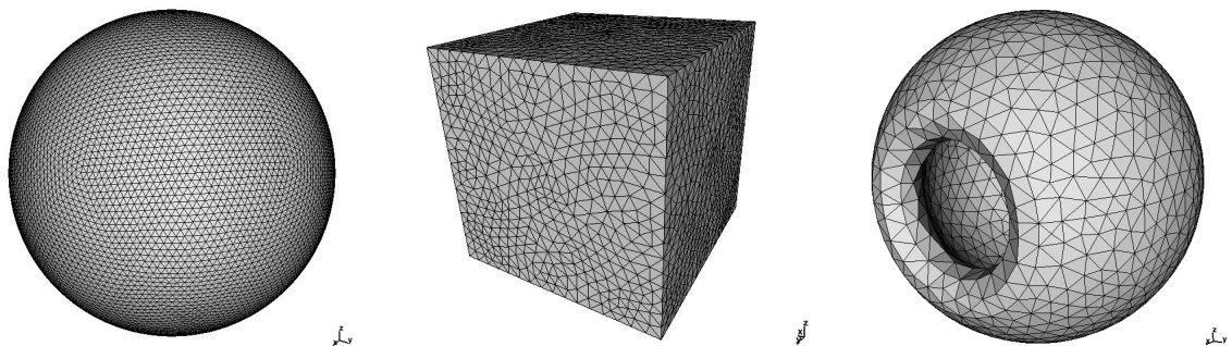
Figure 3.4: Illustration of the geometries considered: a unit sphere, a cube and a sphere with cavity.
