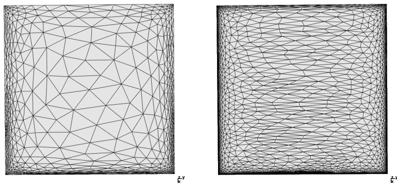
Figure 5.2: Screen case: final adapted meshes for \kappa = 5 (left) and \kappa = 20 (right).
