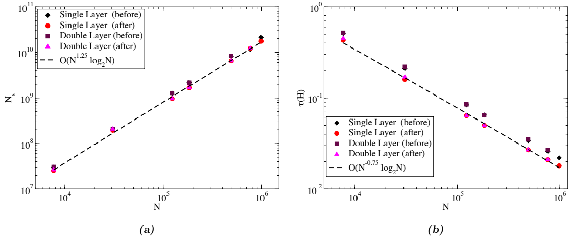
Figure 4.8: Observed and estimated (a) memory requirements N_s and (b) compression rate \tau(\mathcal{H}) with respect to the number of degrees of freedom N for a fixed density of points per S -wavelength for the single and double layer-operators and \varepsilon_{ACA} = 10^{-4} .
