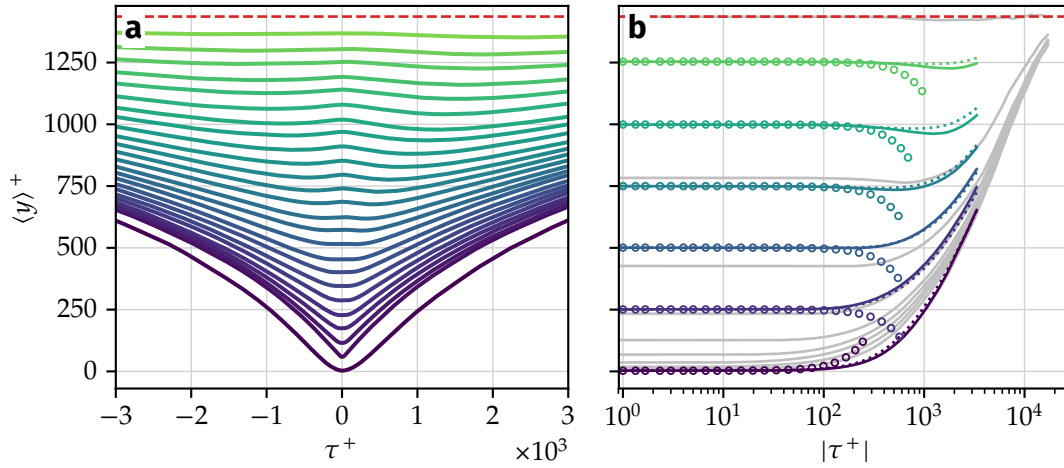
Figure 4.1. Mean wall-normal tracer displacement in the channel. (a) Average wall-normal particle position \langle y \rangle(y_0, \tau) for particles initially located at varying wall distances y_0 . The red dashed line represents the channel centre. (b) Detail on particle sets initially located at y_0^+ = 3, 250, 500, 750, 1000 and 1250 (from bottom to top). Time lag \tau is represented in logarithmic scale. Dotted lines represent backward displacement ( \tau < 0 ). Circles represent the short-time estimation \langle y \rangle \approx y_0 + \bar{a}_y(y_0)\tau^2/2 [eq. (4.2)]. Grey lines represent forward statistics obtained from the long-extent particle dataset DS2 described in chapter 5.
