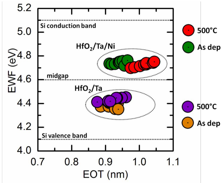
Fig.VI-9- EWF versus EOT for HfO_2/Ta and HfO_2/Ta/Ni capacitors before and after 500°C annealing.
