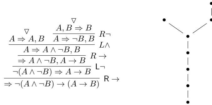
Figure 2.2: Derivation tree
