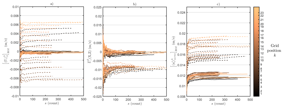
Figure 3.15 – Graph of convergence of statistical quantities. s is the size of sample used for statistical analysis. a) Convergence of the phase average velocity value averaged over the whole ROI. b) Statistical convergence of the same quantity at a given probing location (X,Z) of the ROI (here X=0, Z=50 mm). c) Convergence of the phase rms averaged over the ROI. Full lines are for horizontal velocity components and dashed lines for vertical velocity components.
