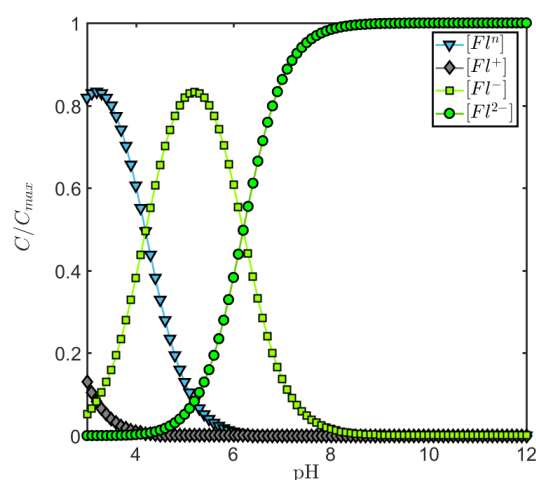
Figure 2.9 – Bjerrum plots of fluorescein sodium system
