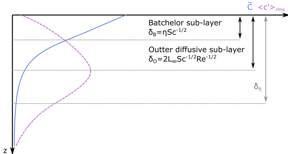
Figure 4.3 – Sketch of the characteristic scalar sub layers of near surface turbulence adapted from Brumley and Jirka (1987), and shape of the profiles of mean concentration (blue full line) and concentration variance (purple dashed line) obtained numerically by Magnaudet and Calmet (2006) and experimentally by Janzen et al. (2010) among others.
