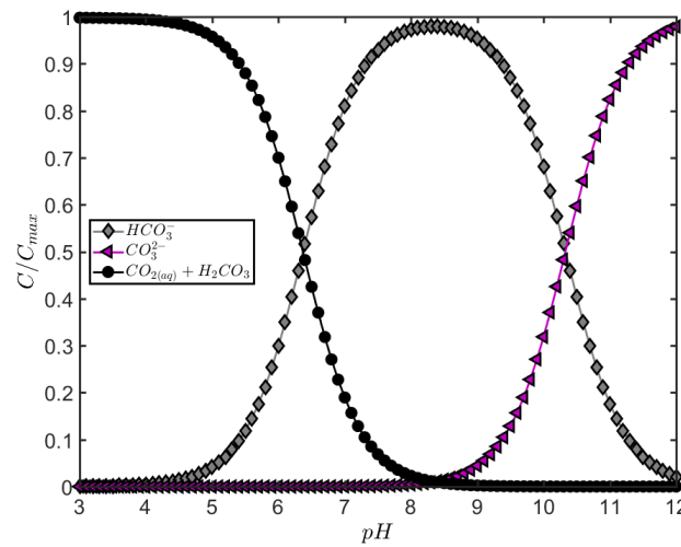
Figure 2.5 – Bjerrum plot of carbonate species into water
