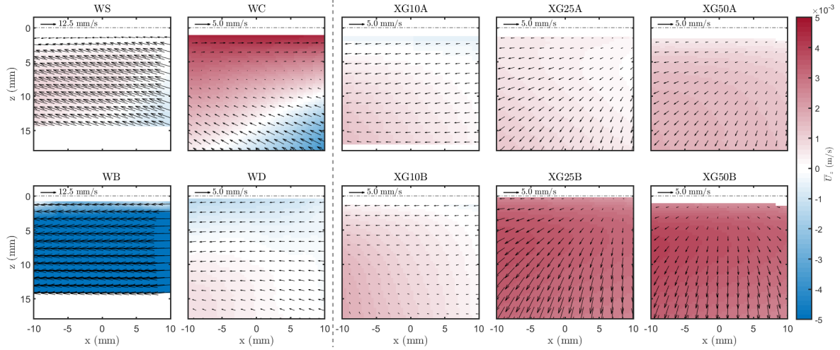
Figure 4.11 – Mean flow under the gas-liquid interface for water (runs WS, WB, WC and WD) and DPS at different concentrations (XG10A, XG10B, XG25A, XG25B, XG50A and XG50B). Vectors show the two in-plane components of the velocity field, and colorbar the out-of-plane velocity component. For clarity, only one every four vector is represented and XG100A run not shown.
