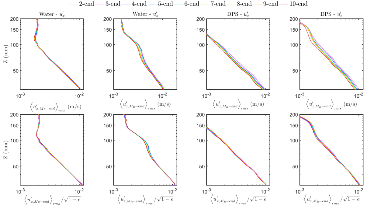
Figure C.9 – Reconstructed rms profiles \langle u'_{x, M_R+1-end} \rangle_{rms} and \langle u'_{z, M_R+1-end} \rangle_{rms} for water and DPS after removal of the first M_R modes, M_R = 1 to M_R = 9 .
