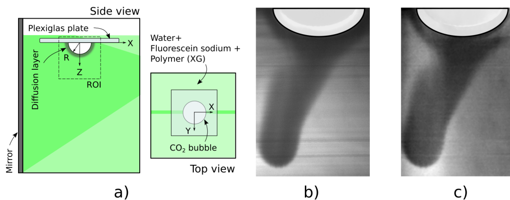
Figure 2.29 – Diphasic test case for I_{\text{pH}}^r – PLIF, a): Sketch of the bubble dissolution condition. b) and c): Fluoresced light intensity (band 1) and intensity ratio around the \text{CO}_2 bubble dissolving XG solution
