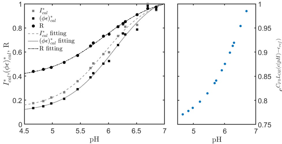
Figure G.1 – Calibration curves for single color methods S and Sa, and for the ratiometric method R. Markers are points measured from calibration images for respectively I_{cal}^* , (\phi\epsilon)_{cal}^* and R. Dashed and dotted lines are hyperbolic tangent fittings later used to turn measured fields into pH fields. The exponential corrective factor e^{C_{F0}L_{OR}(\epsilon(pH)-\epsilon_{ref})} is plotted versus pH in subfigure b.
