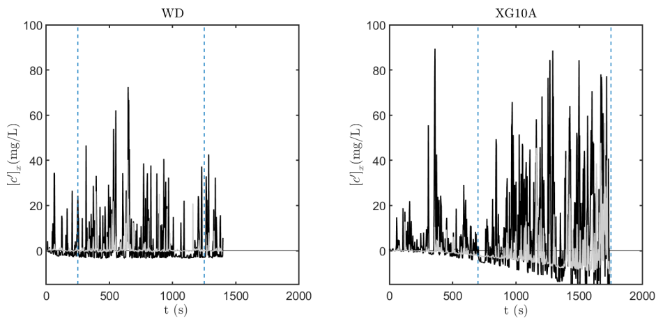
Figure 4.28 – Time series of x averaged concentration fluctuations for water and 10 ppm DPS at two different depths (dark lines for z=0.6 mm, gray lines for z=5.5 mm). Vertical dashed lines denote the time interval over which concentration statistics (rms, PDFs, correlations) are evaluated.
