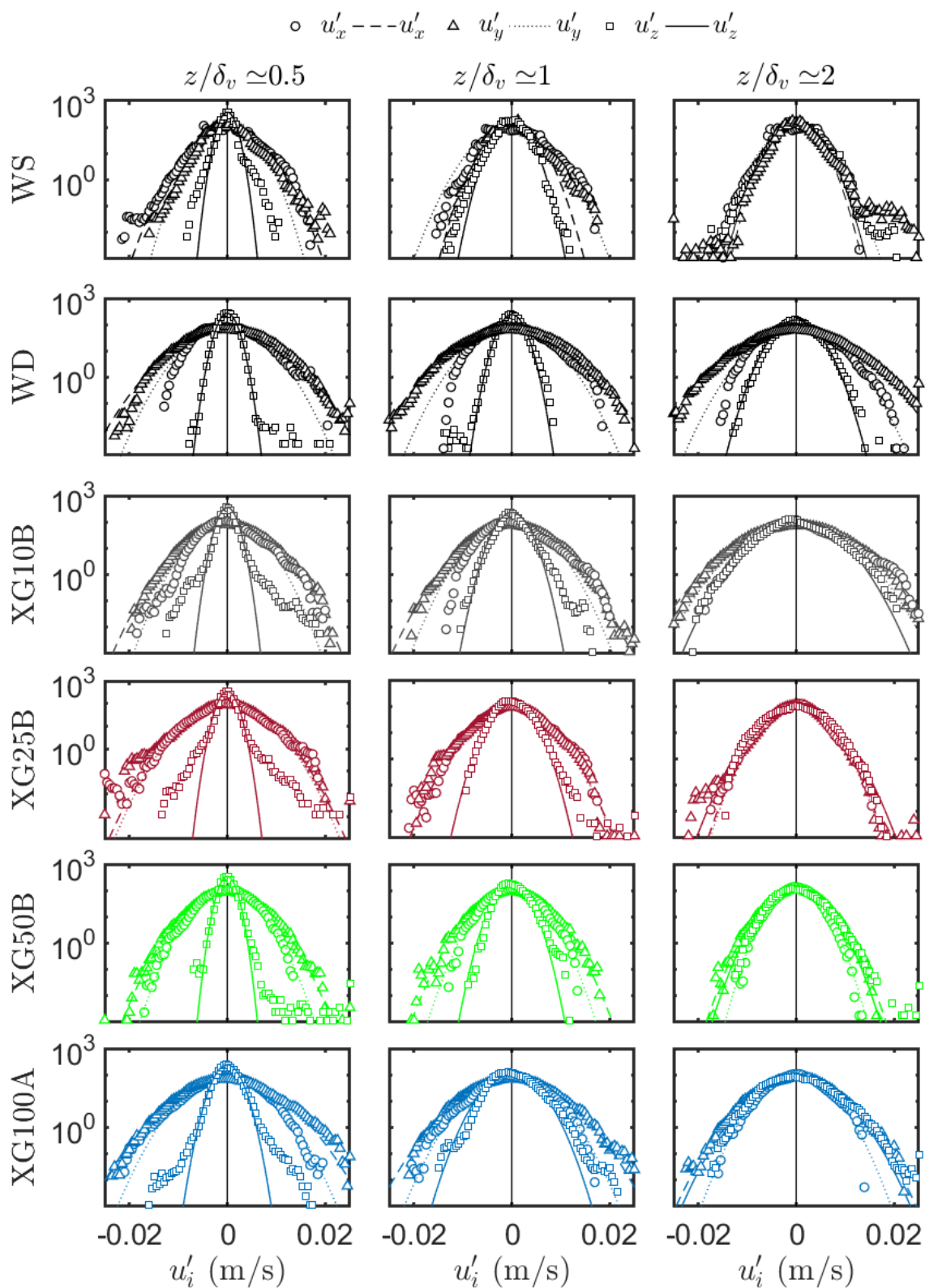
Figure 4.19 – PDF of velocity fluctuations for water and DPS at three relative depths. Results are presented for the runs WD, WS, XG10B, XG25B, XG50B and XG100A, at depths z/\delta_v \approx [0.5, 1, 2] . PDF values are shown in log scale. Lines are Gaussian fittings or the data points (markers).
