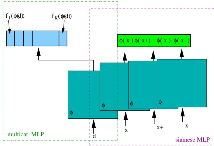
Figure 6.1: Neural Network Structure
