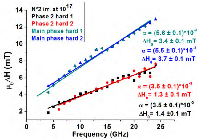
Figure 5.26: Comparison between the two phases in hard axis 1 and 2 for sample N o 2 irradiated at 10^{17} ions/cm 2 as the damping factor \alpha and extrinsic linewidth \Delta H_0 is lower for the second phase than the main phase.
