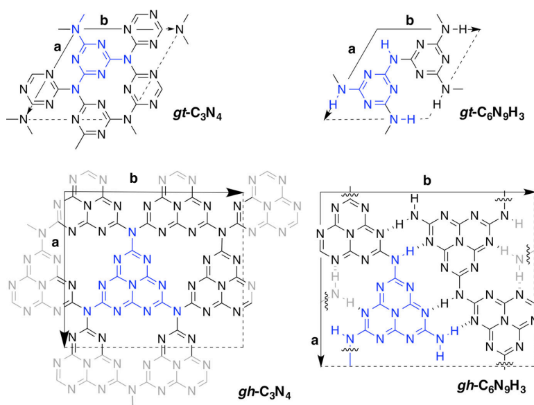
Figure 20. Structures of fully polymerized g\text{-C}_3\text{N}_4 ( gt\text{-} for triazine based and gh\text{-} for heptazine based systems) along with examples of partially polymerized ones. Adapted with permission from “Melissen, S.T.A.G.; Le Bahers, T.; Steinmann, S.N.; Sautet, P. J. Phys. Chem. C 2015, 119, 25188” Copyright (2018) American Chemical Society
