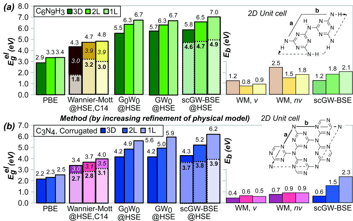
Figure 23 Summary of the results presented in this section. Electronic band gaps for (a) gt-C 6 N 9 H 3 , (b) corrugated gt-C 3 N 4 are reported. The Wannier–Mott analysis using the CRYSTAL14 code is depicted in an alternative color scheme. The optical band gaps E_g^{opt,nv} are depicted semi-transparently. The E_b -corrected band gaps are provided in italics for completion. The WM and scGW-BSE exciton binding energies E_b are provided to the right of the band gaps, with v and nv denoting vibrationally and not vibrationally corrected, respectively. The 2D unit cells for the studied structures are given with lattice vectors a and b.
