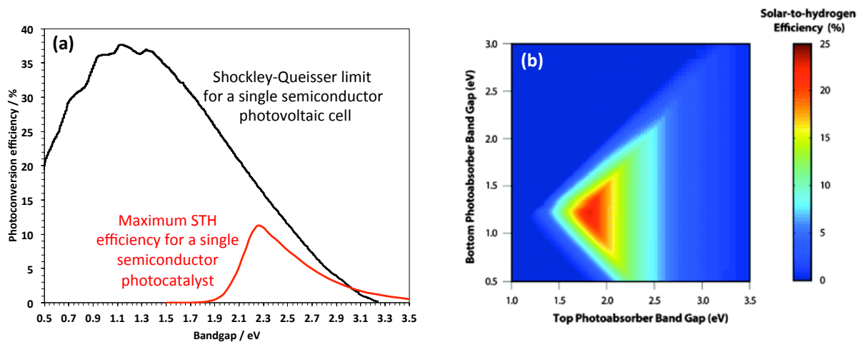
Figure 10. (a) Comparison between the Shockley-Queisser limit of a photovoltaic cell and the Solar-to-Hydrogen (STH) efficiency of a photocatalysts as a function of the bandgap of the semiconductor. (b) STH efficiency of two-junction photocatalysts as a function of the bandgaps of the two semiconductors. From Ref 37
