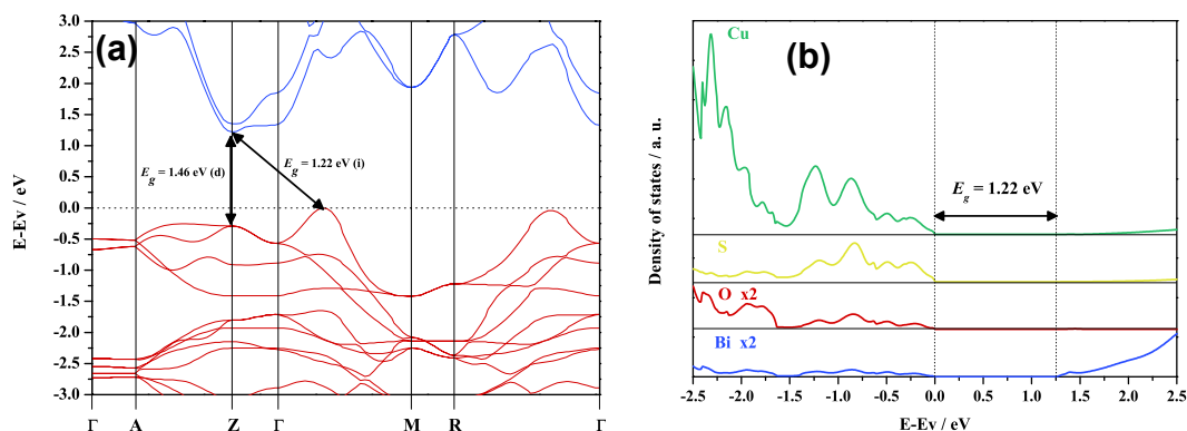
Figure 16. (a) band structure of BiCuOS. (b) Density of states of BiCuOS. Adapted with permission from “Le Bahers, T.; Haller, S.; Le Mercier, T.; Barboux, P. J. Phys. Chem. C 2015, 119 , 17585” Copyright (2018) American Chemical Society
