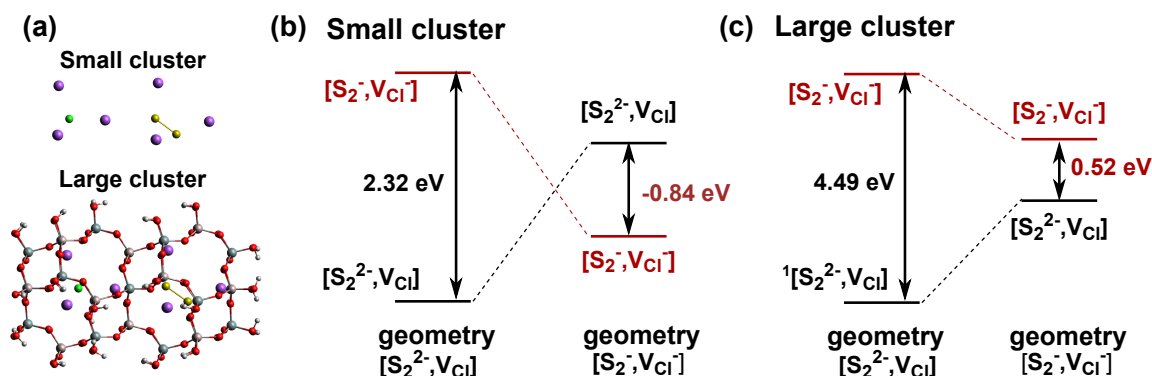
Figure 34: (a) Structure of the small and large clusters. The S 2 2- ion is in yellow and the Cl vacancy is in green (b) and (c) SAC-CI transition energies computed for the two clusters for two geometries.
