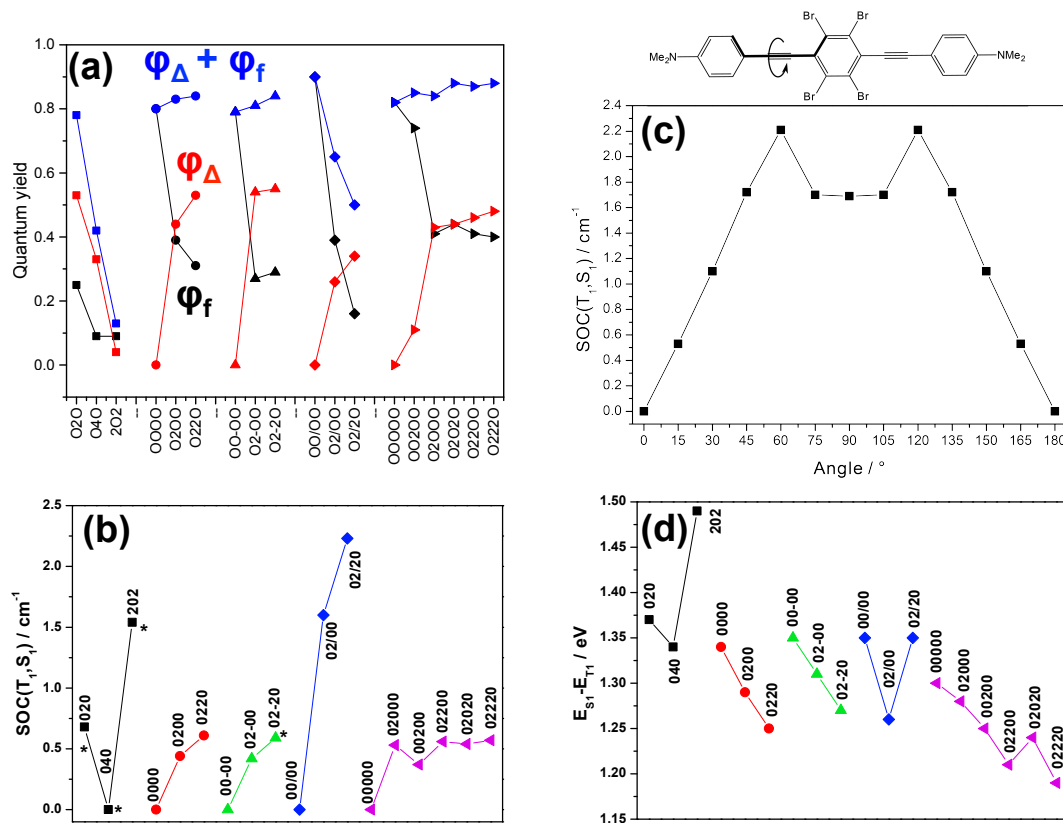
Figure 30. (a) \phi_{\Delta} (red curve), \phi_f (black curve) and \phi_{\text{eff}} (blue curve) (b) Computed SOC between the T 1 and S 1 states (c) Computed SOC between the T 1 and S 1 states for 040 as a function of a dihedral angle corresponding to the rotation between two phenyls. (d) Computed energy (in eV) difference between T 1 and S 1 at the S 1 stable geometry.
