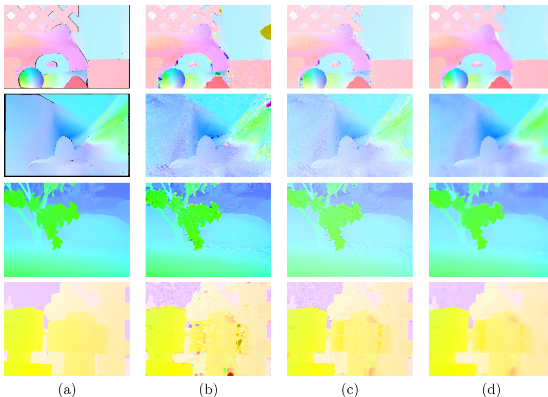
FIGURE 2.13: Flow color map according to Middlebury code : a) Ground truth, b) KLT, c) ours before propagation at the last iteration, d) ours after propagation on 4 sequences : RubberWhale, Dimetrodon, Grove2 and Urban3 from top to bottom respectively.
