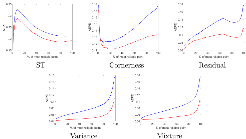
FIGURE 2.12: Comparison of the reliability measures for five criteria using the seeds selection based on grid strategy at 1st pyramidal level and 12th warp iteration (ST, corner, residues, variance and mixture) on Rubberwhale sequence. The blue curve and red curve represent the reliability measure before and after the propagation respectively.
