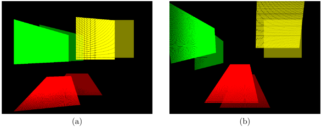
FIGURE 3.17: The 3 simulated planes with the camera movement T = [-0.5, 0.1, 0.5]^T and \Omega_Y = -\pi/20 (a), \Omega_X = -\pi/20 (b) : ex-horizontal (red), ex-lateral(green) and frontal (yellow). The brighter color show the projection of the planes after movement.
