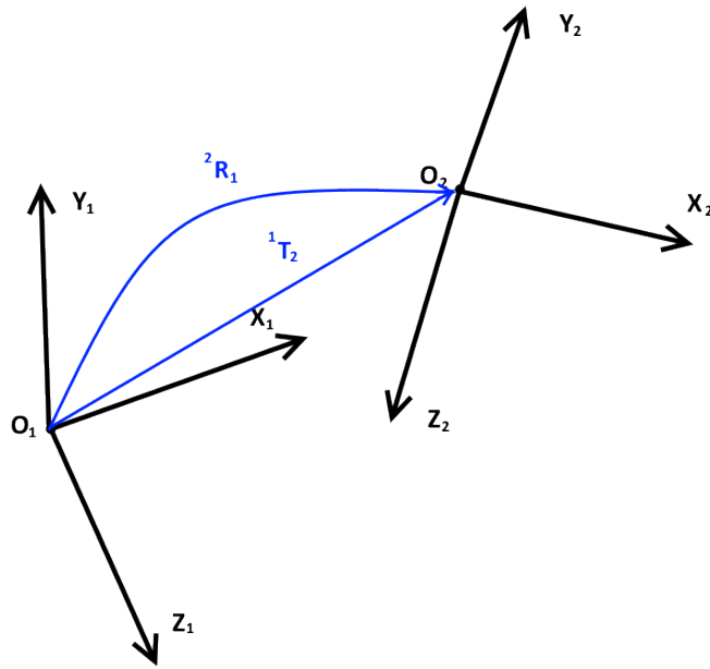
FIGURE 4.9: Illustration of two camera coordinates systems.
