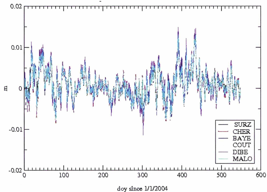
Fig. 2-21 : Non-tidal loading displacements from MOG2D model at GPS stations between 47°-50°N on the shelf of Brittany. (J. Marty personal communication)
