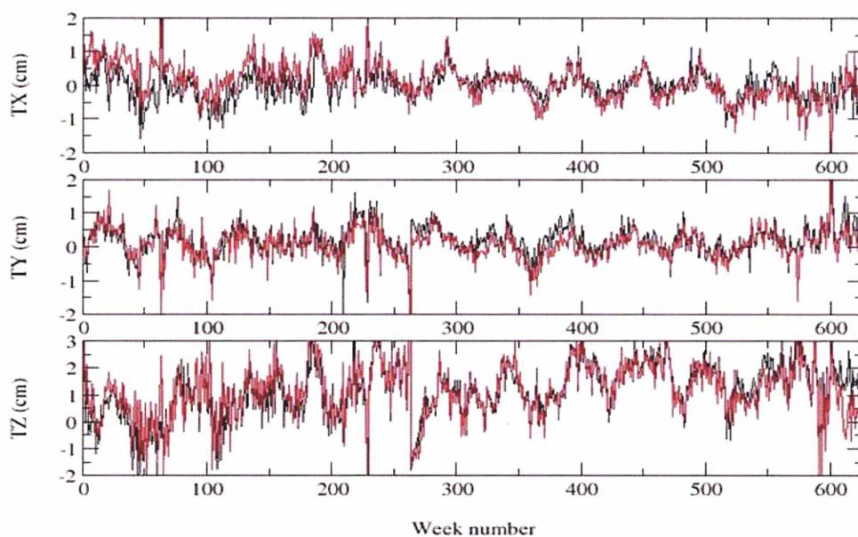
Fig. 2-2 : 12 years of weekly geocenter time-series wrt ITRF2000 from SLR (Coulot et al. 2005)
