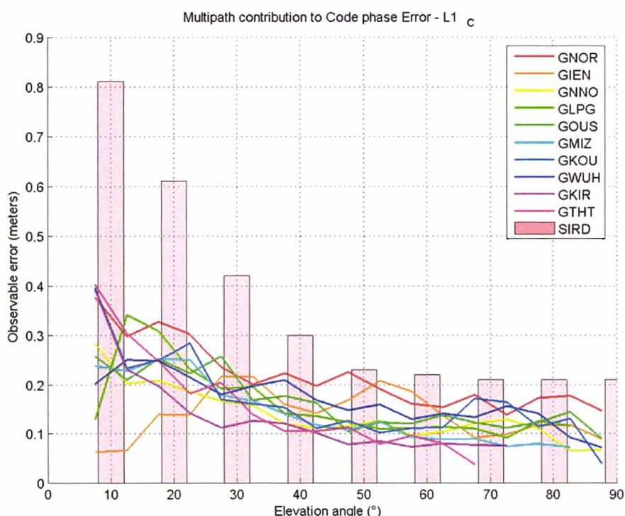
Fig. 1-11 : Code multipath estimation on static environment in GIOVE's infrastructure. SIRD is the required performance for Galileo as it is described in the SIS-ICD ( Navaro-Reyes 2007 )
