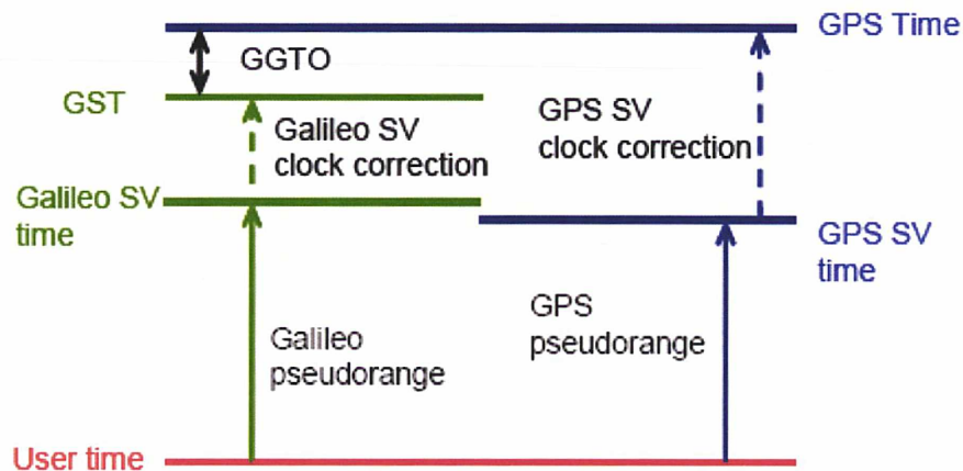
Fig. 1-7 : GPS time versus GST and the GGTO bias in the navigation solution. (Source DLR)
