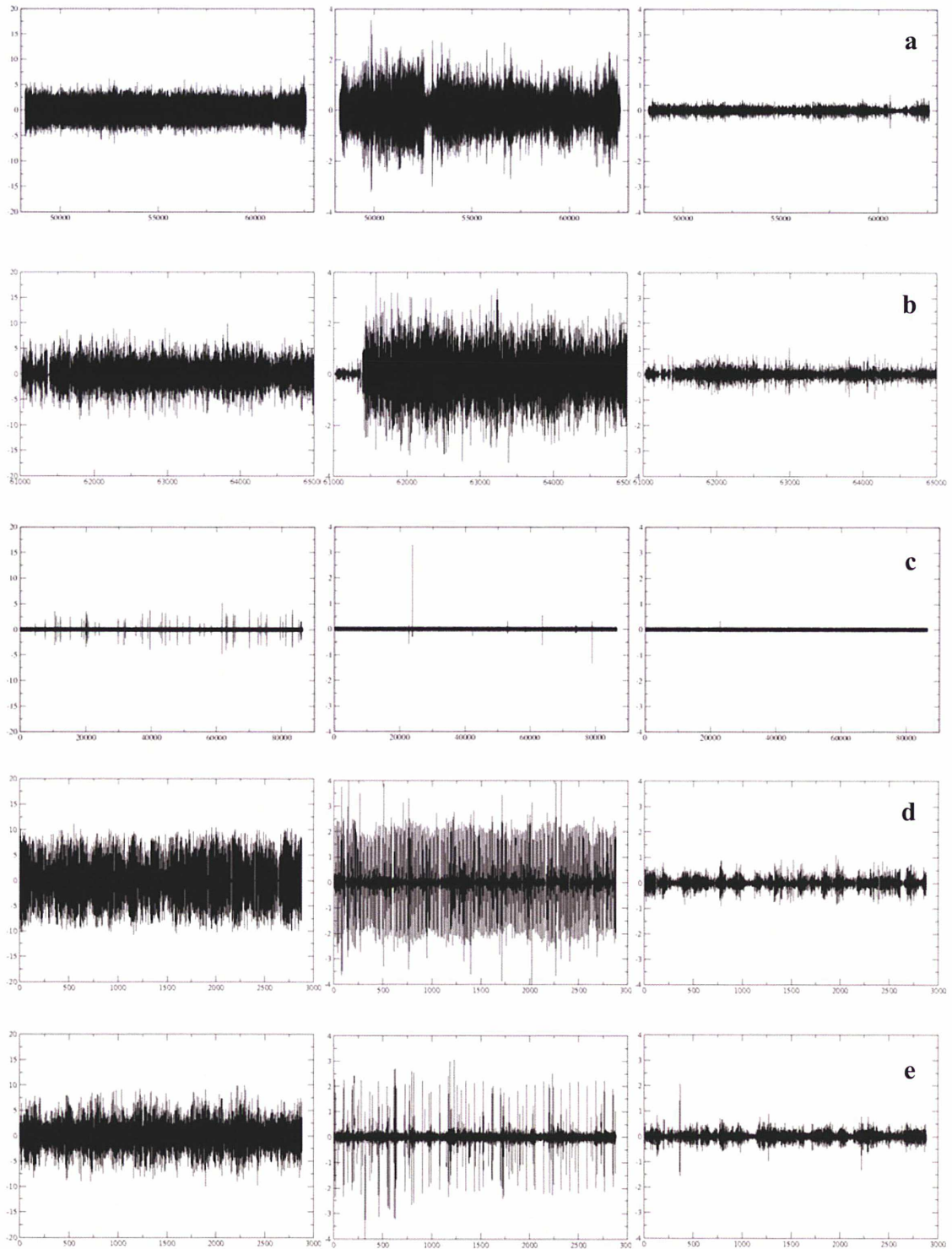
Fig. 2-17 : (a) BOHI, (b) BS07, (c) PALM, (d) BRST, (e) ZIMM, (Left column) Melbourne-Wübbena : L_{WM} , (Center column) Iono-free : L_3 , (Right column) Geometry free L_{10n} . Y-units are in meters and X-axis units are in epochs of 30s or 1s.
