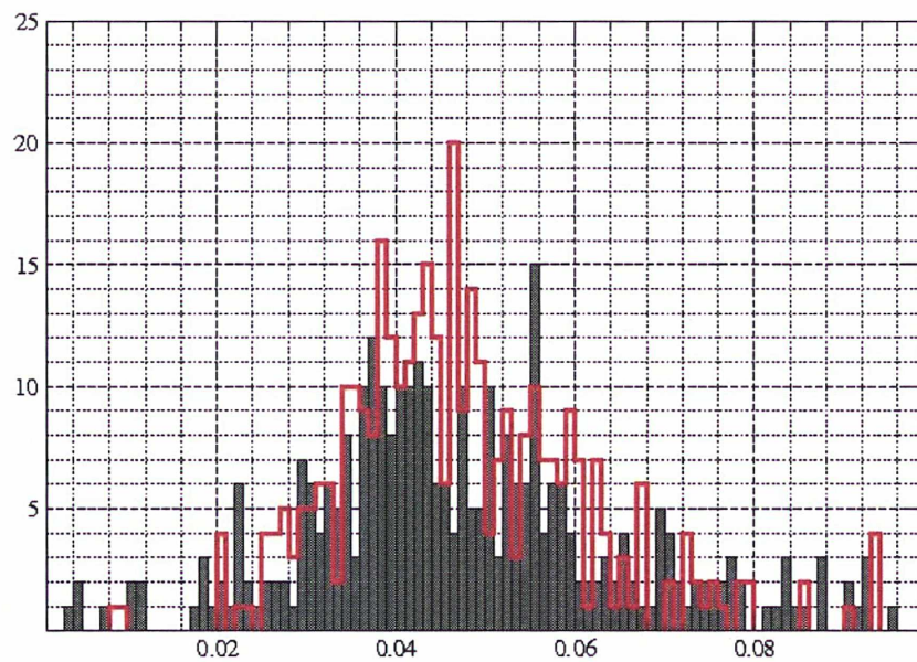
Fig. 3-15 : The mean RMS of range residuals (standard deviation) (m) per SLR stations for PRN 05/06 wrt IGS (in red) and GINS (in black) microwave orbits in year 2005.
