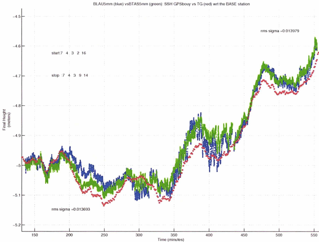
Fig. 5-17 : The two GPS-buoy SSH (3 s) time-series ( in blue and in green) against the collocated TG SSH (1 min) time-series (in red) at Spring Bay, Tasmania.
