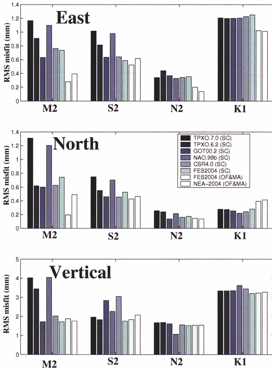
Fig. 4-8 : Misfits of GPS OTL estimates compared to: (SC) Olf/olmpp OTL modelling for: TPXO.7.0, TPXO.6.2, GOT00.2, NAO99.b, CSR4.0, FES2004; (OF&MA) GéochargeV3.0 OTL modelling for: FES2004, NEA-2004. MALO station is excluded. The misfit bars start respectively from left (black) to right (white).
