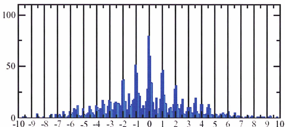
Fig. 2-10 : Distribution of the wide-lane ambiguities N_{WL} (in cycles) (source Noveltis)
