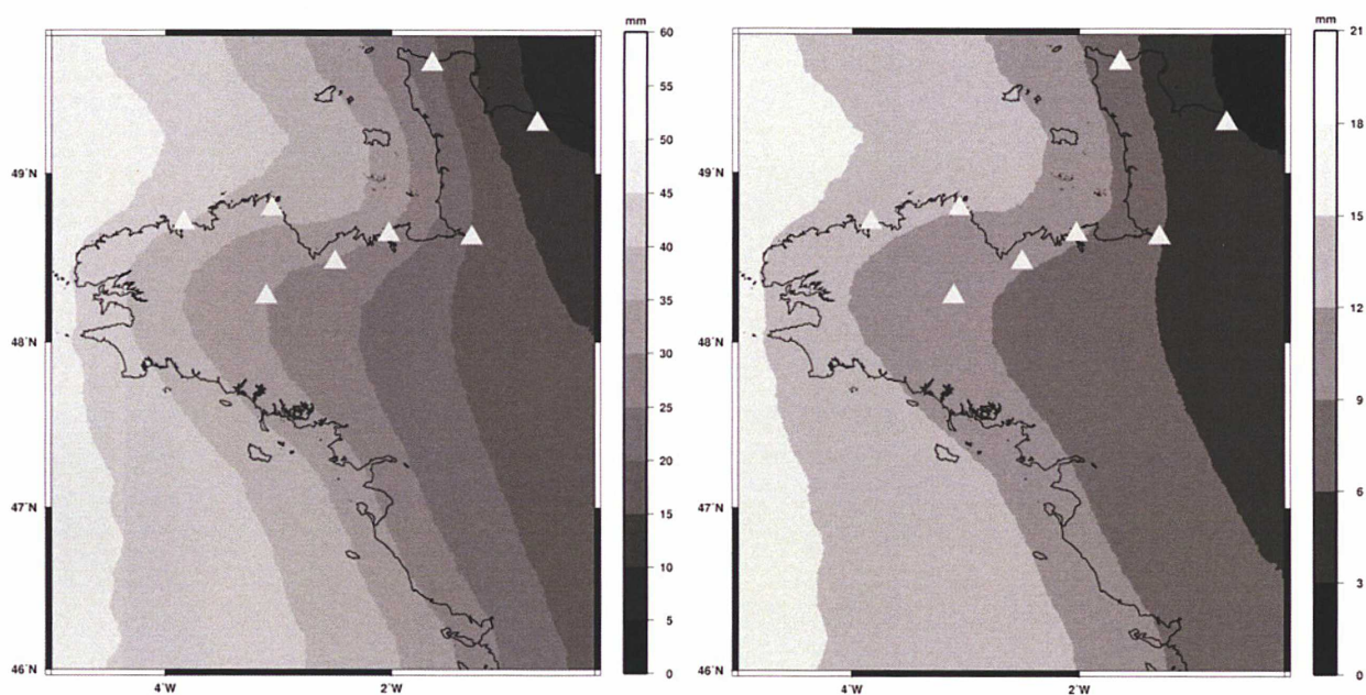
Fig. 4-3 : Amplitudes of the M_2 (left) and S_2 (right) vertical OTL displacement wave over the Brittany shelf and the campaign GPS stations (predictions are from the FES2004 tide model)
