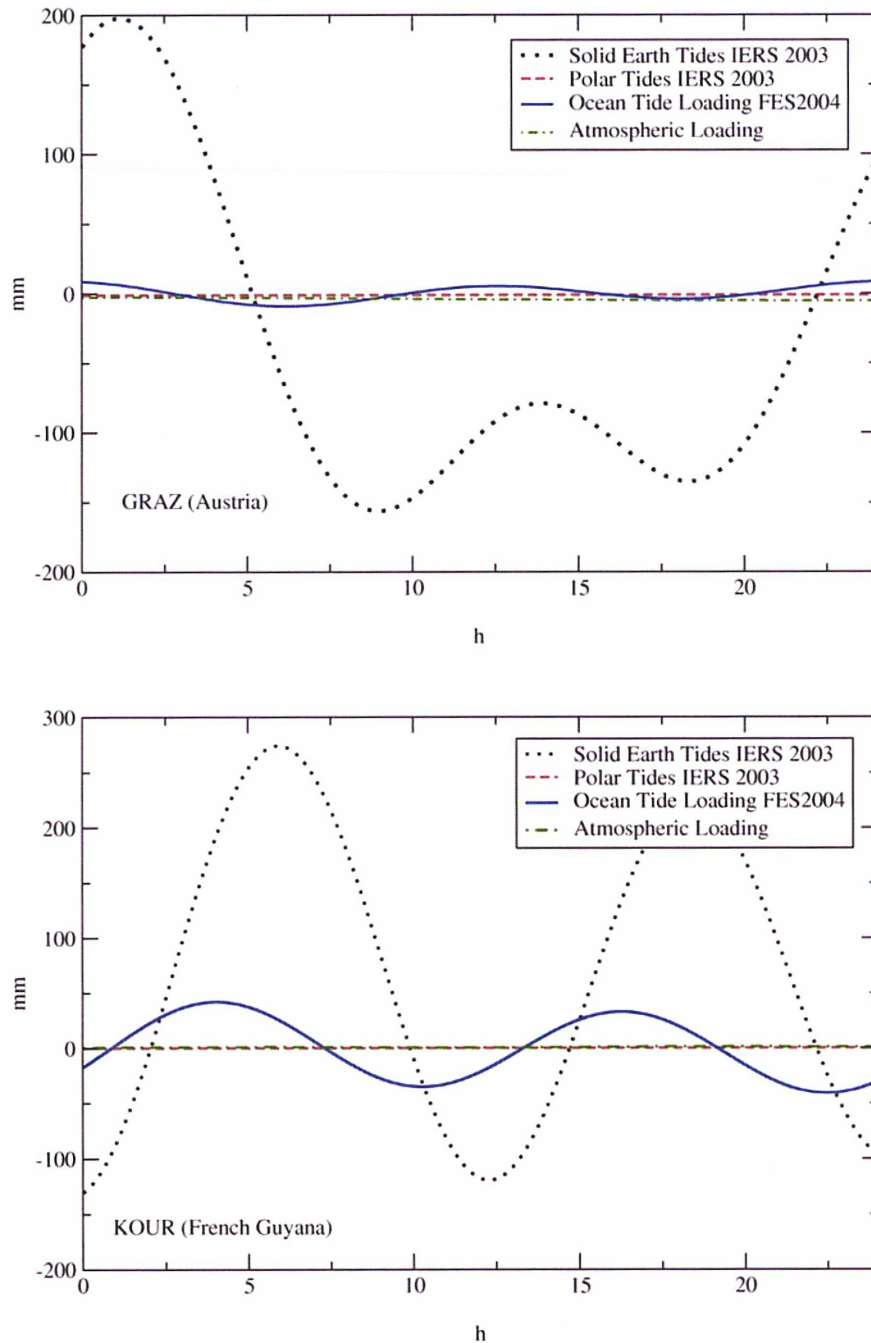
Fig. 2-22 : Ocean loading, atmospheric loading (ECMWF), Polar tides and solid Earth tides displacements in mm over GRAZ (47.061°N and 15.4934°E, Austria) and KOUR (5.2521°N and 307.1940°E, French Guyana) GPS stations over doy 03 2006.
