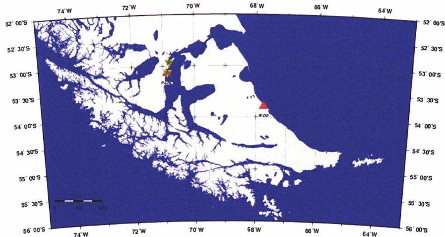
Fig. 5-7 : The GPS network of the 1 st and 2 nd calibration periods. In red are the two reference stations and in yellow the campaign stations.
