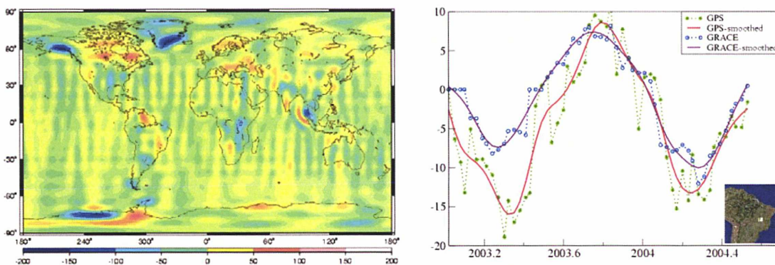
Fig. 2-23 : (Left) Equivalent water height (mm/10-day) trend over 2002-2006 from the GRACE 10-day GRGS gravity field and (right) hydrological loading displacements from GRACE and GPS in BRAZ (station) situated at the Amazonian basin (the satellite image is from google map)
