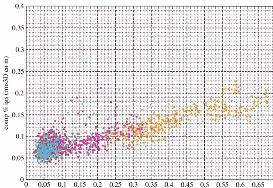
Fig. 3-9 : Internal vs external 3D-RMS misfits for GINS GPS orbits with the Rock T20 and T30 SRP models in four different parameterisations. Units are in meters.
