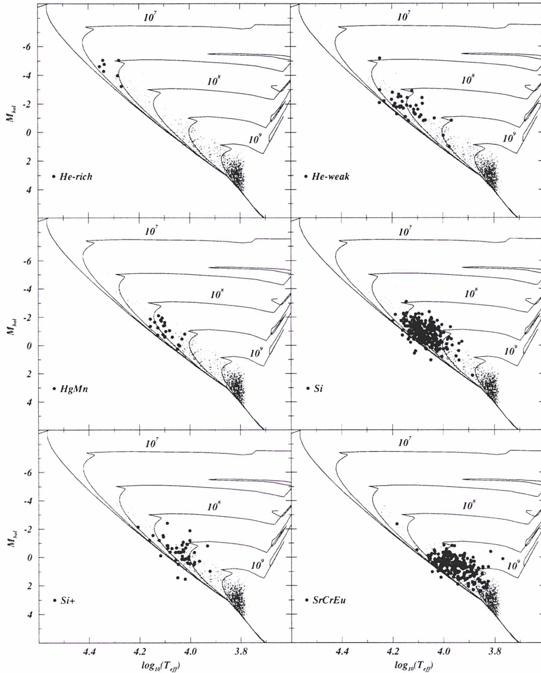
Fig. 2. Distribution in the [\log_{10} T_{eff}, M_{bol}] plane of the stars in the main groups (circles). The results for non-peculiar stars from Gómez et al. (1997a) are indicated (dots)
