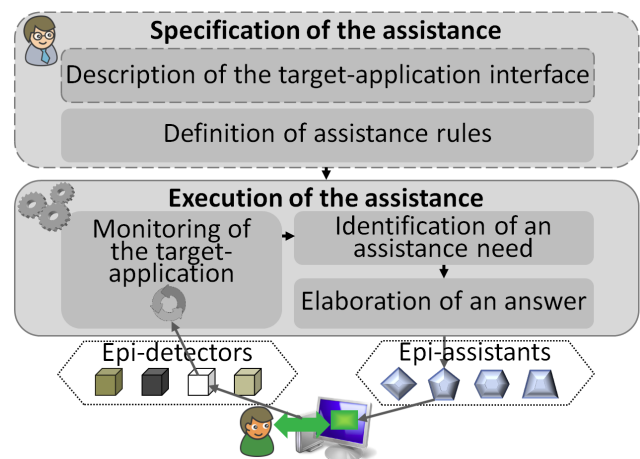
Fig. 3.4 The generic architecture implemented in SEPIA (Ginon et al. 2014)
