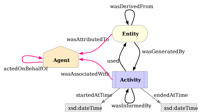
Fig. 4.3 PROV Core Structure (Lebo, Satya Sahoo, and McGuinness 2013)
