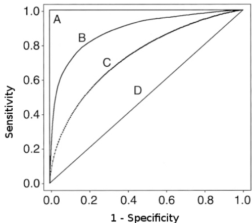
(a) Examples of ROC curves. Each point on the curve corresponds to a pair (sensitivity, 1-specificity). The curves A and D showcase the best and the worst possible performance, respectively. The CAD system corresponding to the curve B outperforms that of C.
