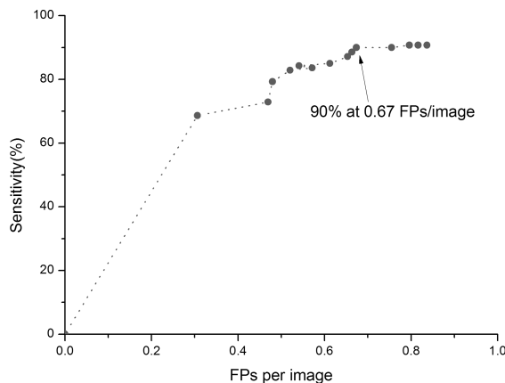
(b) An example of fROC curve. Each point on the curve corresponds to a pair (sensitivity, average number of false positive detections per image).
