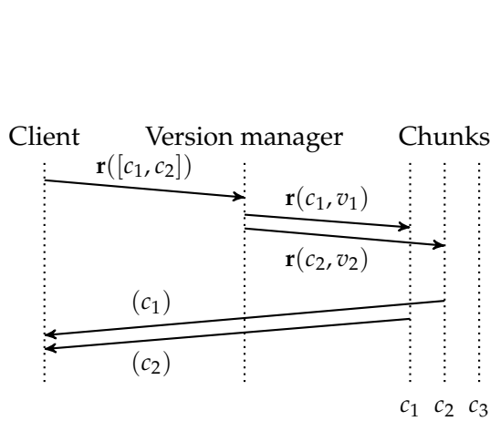
Figure 9.4 – Tír read protocol for a read spanning multiple chunks. The client sends a read query for chunks c_1 and c_2 to the version manager, which relays the query to the servers holding the chunks with the correct version information.
