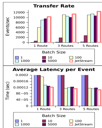
Figure 6.7 – The performance (transfer rate - top and average latency per event - bottom) of individual event streaming, static batches and JetStream for events of size 800 bytes. The performance of individual event streaming (i.e., batch of size 1) are from 40 to 150 times worse than JetStream.
