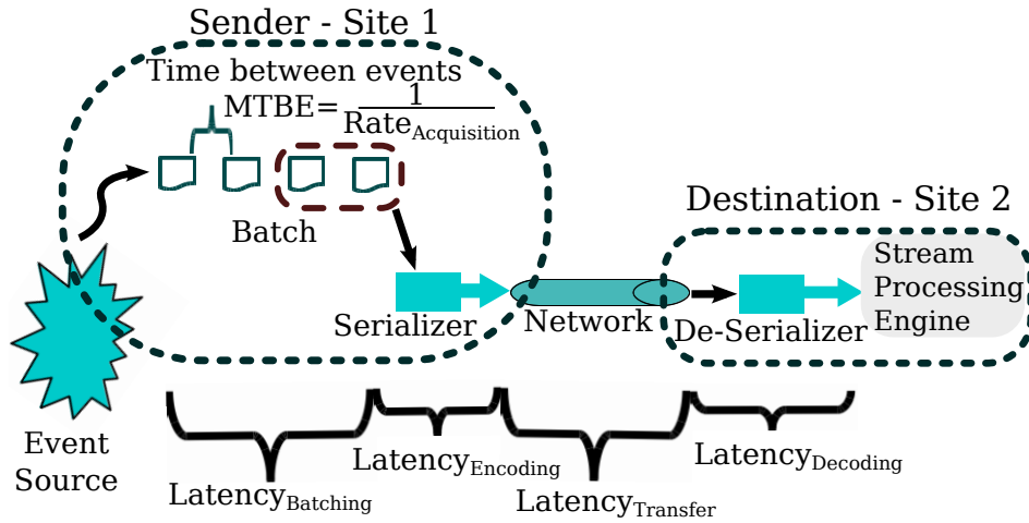
Figure 6.2 – Breaking down the latency to deliver an event from source to stream processing engine across cloud nodes.
