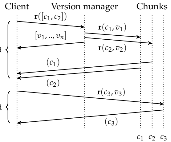
Figure 9.5 – Tír read protocol inside a transaction. The client sends a read query for chunks c_1 and c_2 to the version manager, which relays the query to the servers holding the chunks with the correct version information, and responds to the client with a snapshot of the latest chunk versions. Subsequent read on c_3 is addressed directly to the server holding the chunk data.
