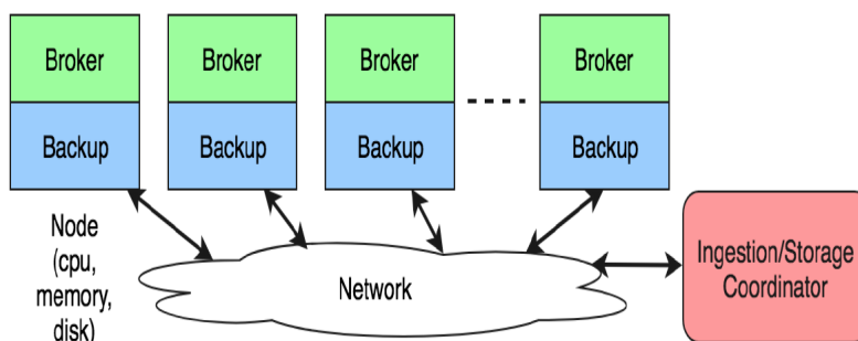
Figure 8.6 – KerA architecture: the Coordinator manages storage nodes on which live Brokers and Backups. Clients mainly interact with Brokers while Backups are simply used for storing stream’s replicas.
