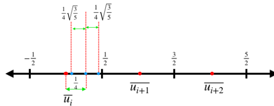
Figure 2.20: Right stencil for interpolation to quadrature point 1.
