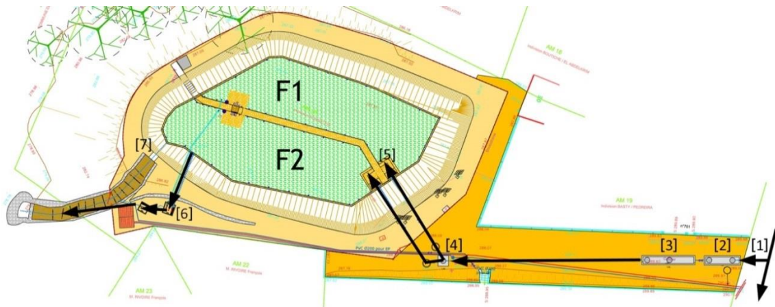
Fig. 7: The routing of flows towards, into and from the filter at Marcy l'Etoile. Point [1] marks the CSO structure and the green rectangles the two filters with the wall between them.
