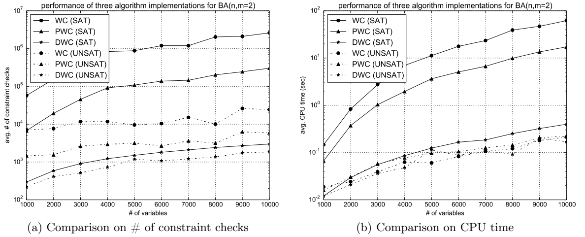
Figure 5.11: Performance comparison for random scale-free RCC-8 networks
