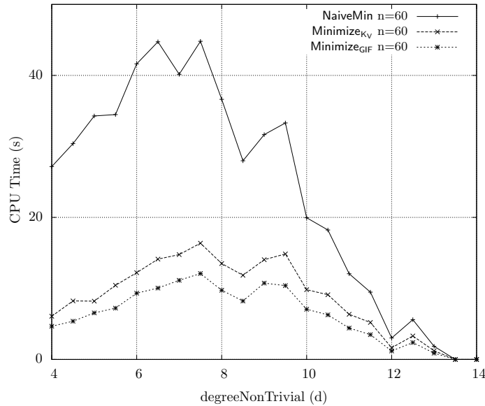
Figure 5.19: CPU time for instances of RCC-8 not forced to be consistent
