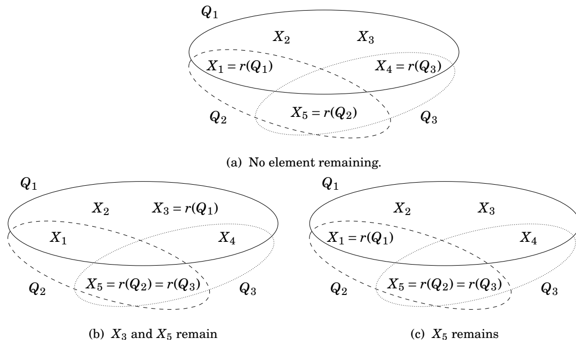
Figure 5.1: Orbits in the generalized orbit \{X_1, X_2, X_3, X_4, X_5\} with various choices of representatives
