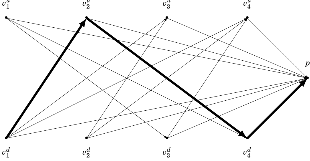
Figure 1.2: A solution to formulation ( F^n -Flow) with n = 1 and T = 4
