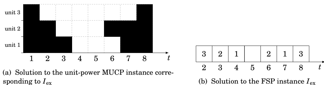
Figure 2.1: Instance I_{\text{ex}} of the FSP: |J| = 3 , p = [3, 3, 6] and \Delta = 7
