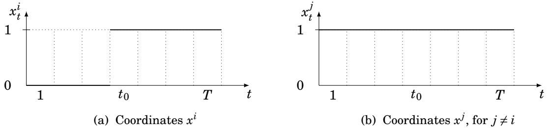
Figure 3.1: Coordinates x of vector \chi_{i,t_0}^u
