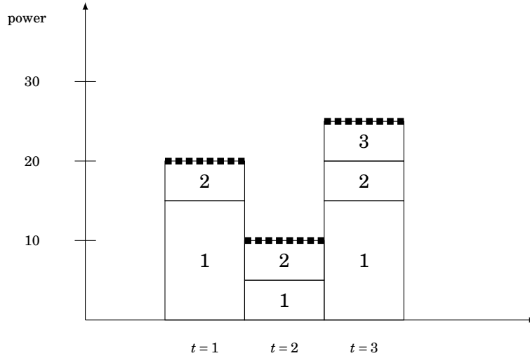
Figure 1.1: Demand values and production plan relative to Example 1.1
