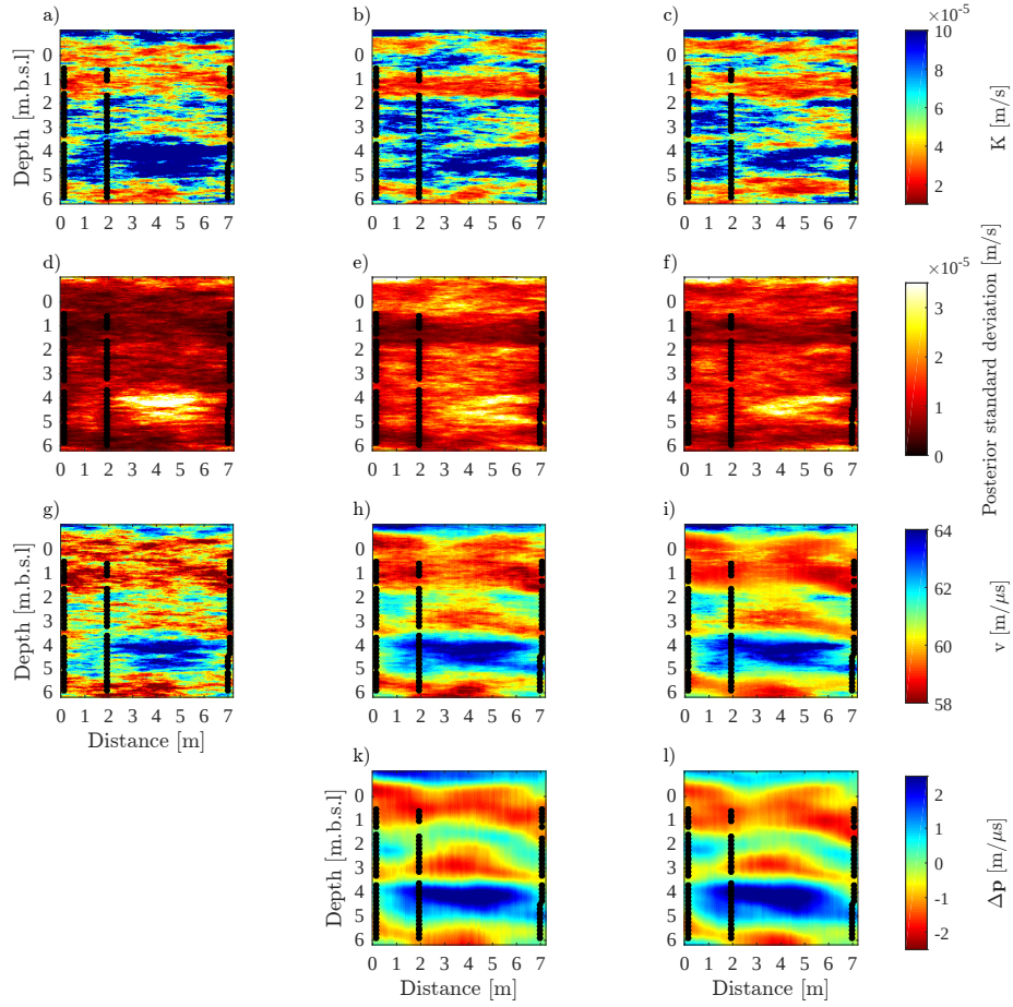
Figure 3.10 – Mean of the posterior hydraulic conductivity, K , realizations obtained using a (a) perfect linear, (b) scattered linear and (c) scattered quadratic petrophysical relationship with the corresponding (d)-(f) standard deviation of the posterior hydraulic conductivity estimates, respectively. Mean of the posterior GPR velocity realizations obtained using (g) perfect linear, (h) scattered linear and (i) scattered quadratic petrophysical relationships. Mean of the posterior petrophysical prediction uncertainty estimates for the (k) linear and (l) quadratic petrophysical relationship. The different measurement depths of the flowmeter data (black points) are indicated for boreholes S14 (on the left), T2 (in the middle) and M3 (on the right). The posterior distributions are computed from MCMC simulation with the DREAM (ZS) algorithm using 8 chains with 2.5 \cdot 10^5 iterations.
