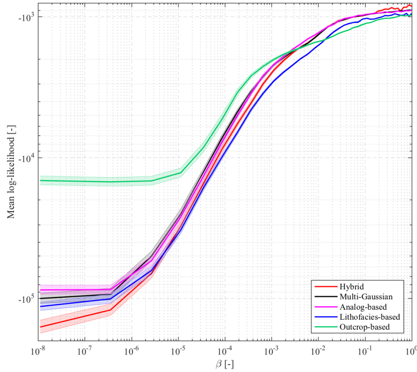
Figure 4.7 – Mean (line) of the natural logarithm of the likelihood functions, \ell , computed for each \beta value and the 95% confidence interval of the \ell -estimates (shaded areas). Note that the x - and y -axes are in \log_{10} scale.
