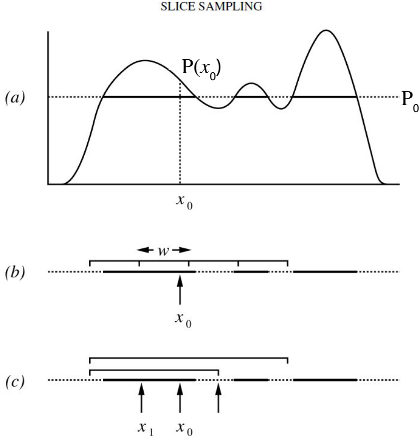
Figure A.2 – Illustration of slice sampling. a) Sample a P_0 slice (probability level) uniformly between 0 and P(x_0) and draw a horizontal line across the curve at this P_0 position. b) An interval of width w is randomly positioned around x_0 , and then expanded in steps until both ends are outside the slice. Then, sample uniformly a point x_1 in w until a point within the slice is found. Points picked outside the slice are used to shrink the interval by replacing one of the interval ends with this point. Repeat the process using the new x_1 value. (Figure modified from Neal (2003))
