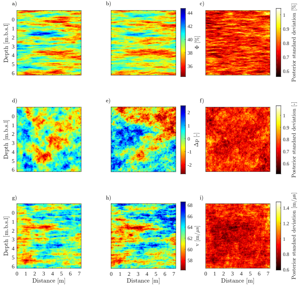
Figure 3.7 – (a) The "true" subsurface porosity model used in our synthetic example; (b) mean porosity field of the posterior distribution derived from MCMC simulation and the corresponding (c) standard deviations. (d) The "true" petrophysical prediction uncertainty model; (e) mean petrophysical prediction uncertainty field of the posterior distribution derived from MCMC simulation and the corresponding (f) standard deviations. (g) The "true" GPR velocity model; (h) mean velocity field of the posterior distribution derived from MCMC simulation and the corresponding (i) standard deviations. The mean fields are obtained from MCMC simulation with the DREAM (ZS) algorithm using 8 chains with 2.5 \cdot 10^5 iterations.
