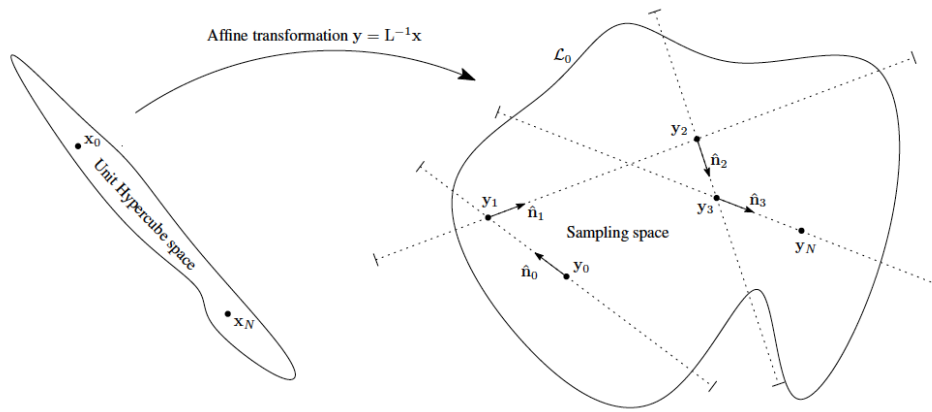
Figure A.1 – Slice sampling in d dimensions. The unit hypercube is whitened by linearly transforming a degenerate contour into one with dimensions \sim \mathcal{O}(1) in all directions. (Figure from Handley et al. (2015a))
