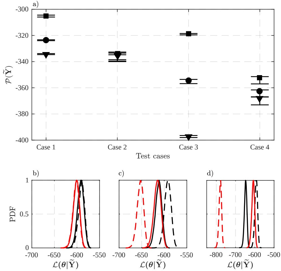
Figure 3.5 – (a) Mean values of the evidence in \log_{10} space, \mathcal{P}(\tilde{\mathbf{Y}}) , and corresponding uncertainty (error bars) derived from the Gaussian mixture importance sampling method for the multi-Gaussian conceptual models with horizontal anisotropy (squares), isotropy (circles) and vertical anisotropy (triangles). Posterior distribution of the log-likelihood, \mathcal{L}(\theta|\tilde{\mathbf{Y}}) , for the multi-Gaussian model with (b) horizontal anisotropy, (c) isotropy and (d) vertical anisotropy in Case 1 (black solid line), Case 2 (black dotted line), Case 3 (red dotted line) and Case 4 (red solid line).
