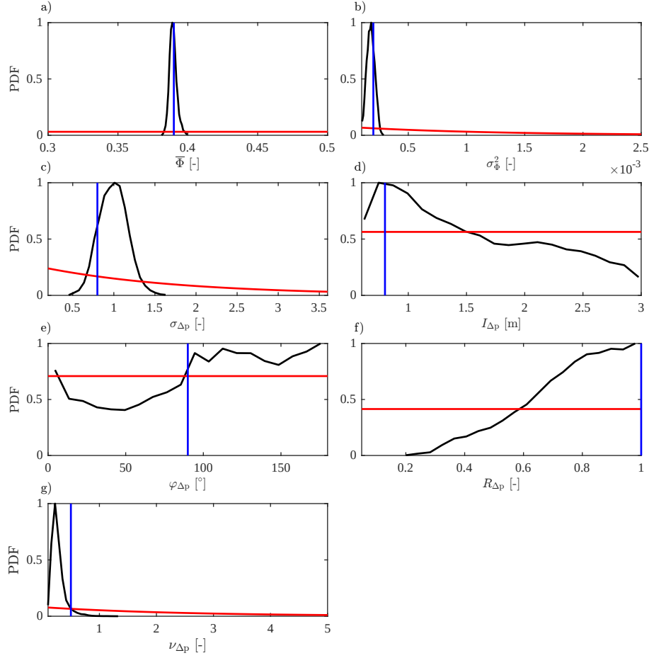
Figure 3.6 – Posterior distributions (black lines) derived from MCMC simulation with the DREAM (ZS) algorithm using 8 chains with 2.5 \cdot 10^5 iterations of the (a) inferred mean, \bar{\Phi} , and (b) variance, \sigma_{\Phi}^2 , of the porosity field and of the geostatistical parameters of the petrophysical prediction uncertainty field: (c) standard deviation, \sigma_{\Delta p} , (d) integral scale along the major axis of anisotropy, I_{\Delta p} , (e) anisotropy angle, \varphi_{\Delta p} , (f) ratio of the integral scales along the minor and major axis of anisotropy, R_{\Delta p} , and (g) shape parameter of the Matérn variogram, \nu_{\Delta p} . The red and blue lines depict the corresponding prior distributions and values of the reference field, respectively. The densities in each plot are normalized.
