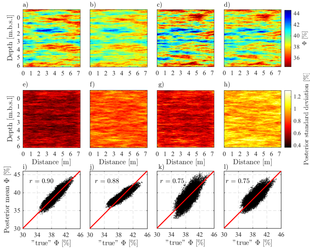
Figure 3.4 – (a-d) Mean porosity fields of the posterior distribution derived from MCMC simulation with the DREAM (ZS) algorithm using 8 chains with 2.5 \cdot 10^5 iterations for Cases 1-4, respectively. The corresponding posterior standard deviations of the porosity estimates for the four different cases are shown in (e-h), respectively. From (j) to (l), scatter plots of the "true" porosity values versus the mean posterior porosity estimates obtained in the four cases. In each plot, from (j) to (l), the Pearson correlation coefficients, r , are reported and the red lines depict the theoretical 1:1 trend line (i.e., Pearson correlation coefficient equal to 1).
