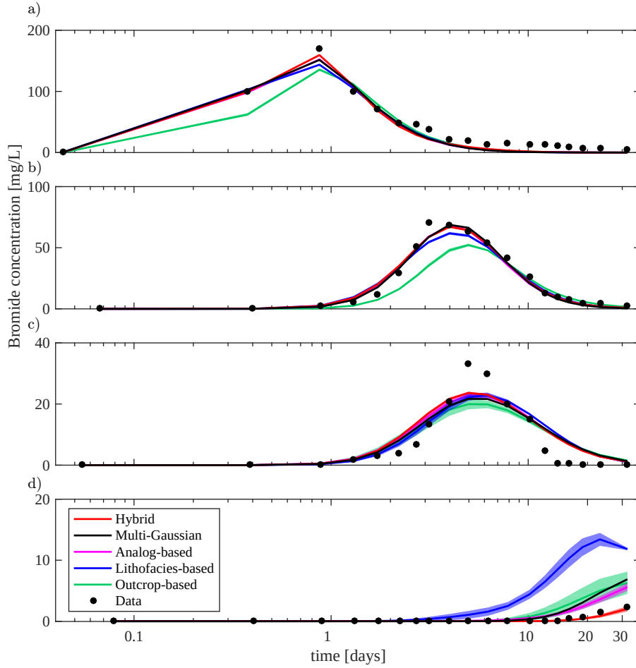
Figure 4.5 – Simulated (solid lines) and measured (black dots) bromide breakthrough curves from the MADE-5 experiment in the two monitoring wells MLS-1 and MLS-2 at a depth of 7 m (a-b) and 11 m (c-d), respectively. The simulated breakthrough curves are summarised by the mean of the posterior realisations (solid lines) and their 95% confidence intervals (shaded areas).
