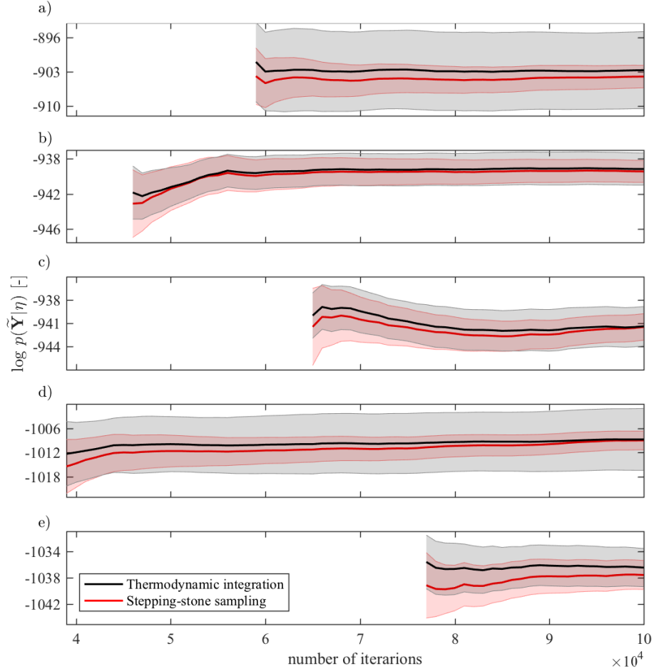
Figure 4.6 – Natural logarithm of the evidence estimates, \log p(\tilde{\mathbf{Y}}|\eta) , as a function of the number of MCMC iterations. Evidences are computed with the stepping-stone sampling method (red line) and the thermodynamic integration method based on the corrected trapezoidal rule (black line) for the (a) hybrid, (b) multi-Gaussian, (c) analog-based, (d) lithofacies-based and (e) outcrop-based model at the MADE site. The evidence computation starts after a different number of MCMC iterations because each of the conceptual models has a specific burn-in period. The shaded areas represent the 95% confidence interval of the evidence estimates (pink for stepping-stone sampling and grey for thermodynamic integration).
