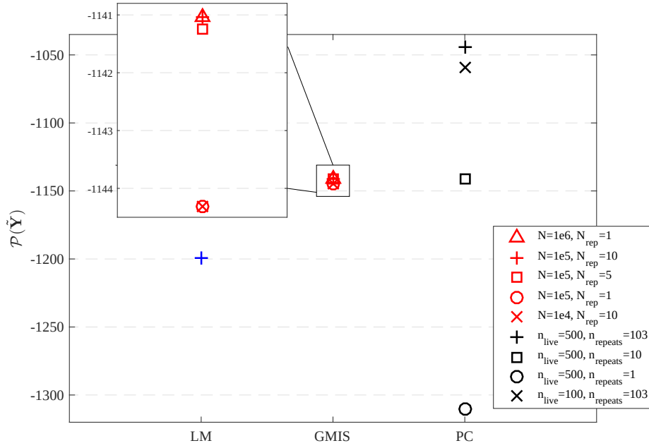
Figure A.12 – Evidence in \log_{10} space, \mathcal{P}(\tilde{\mathbf{Y}}) derived from the GMIS, LM and PC estimators using different setting as shown in the legend. In the case of the GMIS method, N indicates the number of importance samples and N_{rep} is the number of evidence estimates used to compute the mean evidence. Colour coding is used to differentiate among the different methods.
