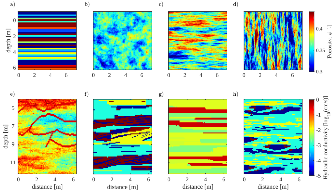
Figure 1.1 – Examples of conceptual models of subsurface (hydro)geological heterogeneity parameterised with the (a) zonation, (b-d) variogram-based and (e-h) multiple-point geostatistics approaches. The different spatial parameterisations consist of (a) horizontal layers, (b) multi-Gaussian with isotropy, (c) multi-Gaussian with horizontal anisotropy, (d) multi-Gaussian with vertical anisotropy and (e) conductive channels overlapped on a multi-Gaussian field (i.e., combination of continuous and categorical fields) and (f-h) categorical fields (i.e., each facies has a specific value of the hydrogeological property).
