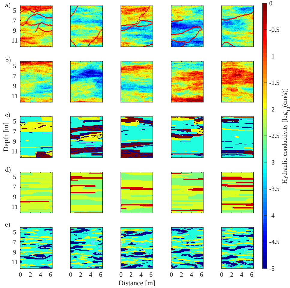
Figure 4.3 – Five prior realisations of hydraulic conductivity fields generated from the training images of Figure 4.2 with the Graph Cuts algorithm for the (a) hybrid, (b) multi-Gaussian, (c) analog-based, (d) lithofacies-based and (e) outcrop-based conceptual model of the MADE site.
