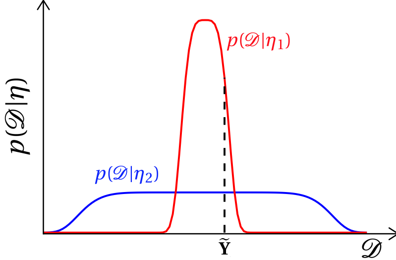
Figure 1.2 – The principle of parsimony in Bayesian model selection. The evidence is here interpreted as the normalised probability distribution, p(\mathcal{D}|\eta) , on the space of all possible data sets of fixed size n , \mathcal{D} . A more simple conceptual model, \eta_1 , spreads the probability distribution, p(\mathcal{D}|\eta_1) (red line), over a smaller range of data sets than a more complex model, \eta_2 , (blue line). Given the observed data set, \tilde{Y} (dotted black line), then it is clear that the simpler model \eta_1 receives a higher evidence than \eta_2 provided that the two conceptual models fit (almost) equally well \tilde{Y} and they have equal prior probability. (Figure inspired by the figures from MacKay (2003); Ghahramani (2013)).
