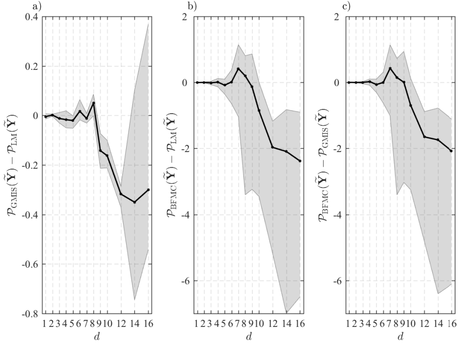
Figure 2.3 – Difference in the evidence estimates derived from different pairs of two methods as function of model complexity, (a) GMIS and LM, (b) BFMC and LM, and (c) BFMC and GMIS. The solid black line in each graph portrays the difference in the mean evidence estimates, and the grey shaded region quantifies the range associated with the difference in the mean evidence estimates of each method. Note, we use \log_{10} transformed value of the evidence estimates.
