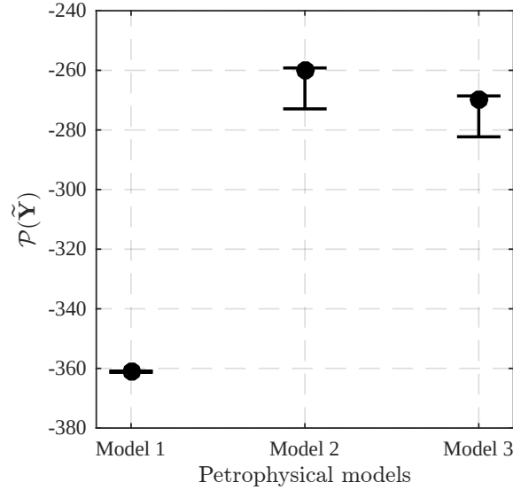
Figure 3.12 – Mean values of the evidence in \log_{10} space, \mathcal{P}(\tilde{\mathbf{Y}}) , and corresponding uncertainty (error bars) derived from the Gaussian mixture importance sampling method for (Model 1) a perfect linear petrophysical relationship as shown in Eq. (3.9), (Model 2) scattered linear petrophysical relationship such that \Delta \mathbf{p} is taken into account as shown in Eqs. (3.9) and (3.11), (Model 3) scattered quadratic petrophysical relationship where \Delta \mathbf{p} is taken into account as shown in Eqs. (3.10)-(3.11).
