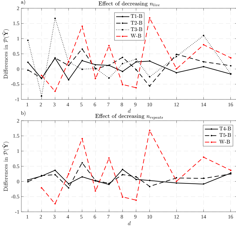
Figure A.7 – Difference in the evidence estimates derived from tests T1, T2, T3, T4, T5 (Table A.1) with respect to the "best" case, B, where n_{live} and n_{repeats} are set as suggested by Handley et al. (2015b,a). (a) effect of decreasing n_{live} from 25d to d while keeping n_{repeats} constant and (b) effect of decreasing n_{repeats} from 5d to d while keeping n_{live} constant. The red line depicts the differences in evidence estimates between the "best" setting, B, and "worst" setting, W. Note, we use \log_{10} transformed differences of the evidence estimates.
