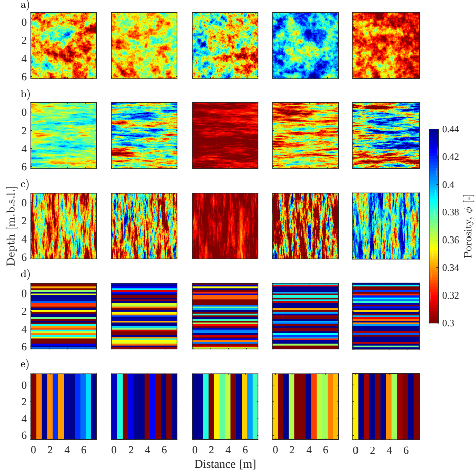
Realizations drawn randomly from the prior distribution for the (a) isotropic multi-Gaussian model, (b) multi-Gaussian model with horizontal anisotropy, (c) multi-Gaussian model with vertical anisotropy, (d) horizontally layered model with 37 layers of equal thickness, and (e) vertically layered model with 12 layers of equal thickness.
