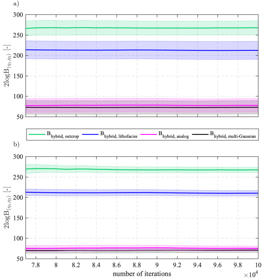
Figure 4.9 – Twice the natural logarithm of the Bayes factors of the "best model" (hybrid) with respect to the outcrop-based (green line), lithofacies-based (blue line), analog-based (magenta line) and multi-Gaussian (black line) conceptual model at the MADE site. Results are shown for (a) the thermodynamic integration method based on the corrected trapezoidal rule and for the (b) stepping-stone sampling method. The shaded areas represent the 95% confidence interval of the 2\log B_{\eta_1, \eta_2} measures.
