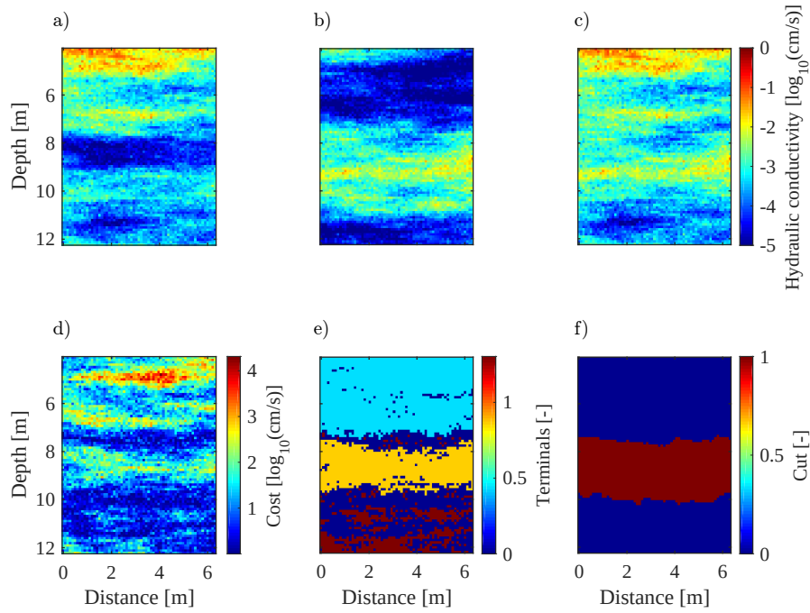
Figure 4.1 – Illustration of how model proposals are obtained using the Graph Cuts algorithm. (a) Current model realisation, \theta_{\text{cur}} , (b) section drawn randomly from the training image, \theta_{\text{new}} , and (c) the resulting model proposal, \theta_{\text{prop}} . This model proposal is obtained as follows: (d) the cost image, \delta , is defined as the absolute difference raised to the cost power, \delta_{cp} , that is \delta = |\theta_{\text{cur}} - \theta_{\text{new}}|^{\delta_{cp}} , (e) two disconnected regions of high differences (light blue and orange areas) of similar size are randomly selected and (f) the cut of minimum cost that separates the two regions is calculated and the resulting dark red region is cut from (b) \theta_{\text{new}} and pasted into (a) \theta_{\text{cur}} to create (c) \theta_{\text{prop}} .
