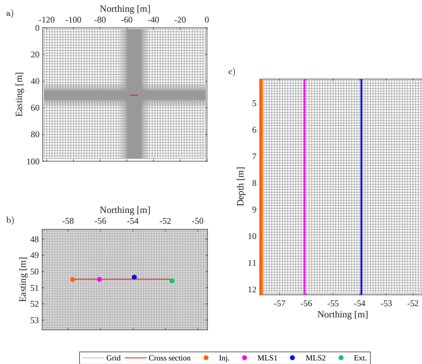
Figure 4.10 – (a) Aerial view of the 3D grid used for simulations with MODFLOW/MT3DMS; (b) zoom in the tracer test area, in which the grid size was refined to 0.1 m; (c) cross section used for simulations with MaFloT. The width of the lines in (c) is representative of the diameter of the four wells.
