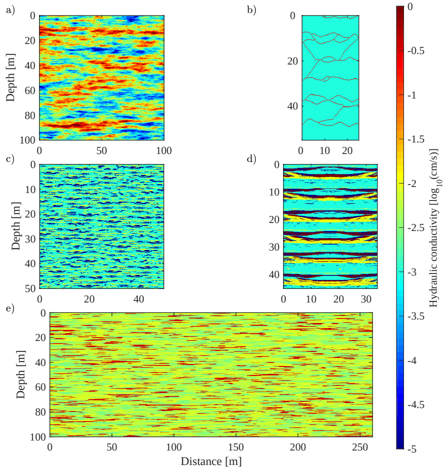
Figure 4.2 – Training images used in the MPS-based inversion to represent spatial hydraulic conductivity of the MADE site: (a) multi-Gaussian field (Bianchi et al., 2011a), (b) highly conductive channels in an homogeneous matrix (Strebelle, 2002; Ronayne et al., 2010; Linde et al., 2015a), (c) model based on a mapping study of a MADE outcrop (Rehfeldt et al., 1992; Linde et al., 2015a), (d) model based on a mapping study at the Herten site in Germany (Bayer et al., 2011; Comunian et al., 2011; Linde et al., 2015a) featuring representative alluvial deposit structures and (e) model based on lithological borehole data collected at the MADE site (Bianchi and Zheng, 2016).
