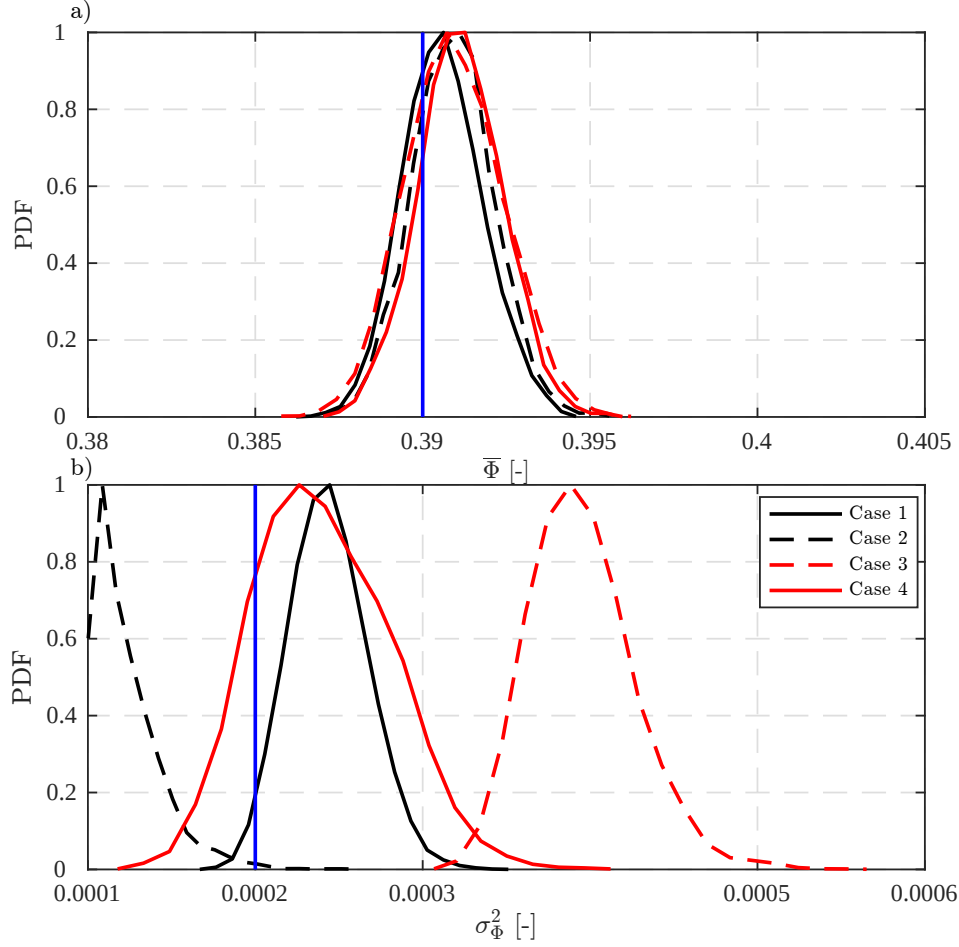
Figure 3.3 – (a) Posterior distributions of the inferred mean of the porosity field. (b) Posterior distributions of the inferred variance (i.e., sill) of the porosity field. The vertical blue lines depict the values of the true model. The posterior distributions are derived from MCMC simulation with the DREAM (ZS) algorithm using 8 chains with 2.5 \cdot 10^5 iterations.
