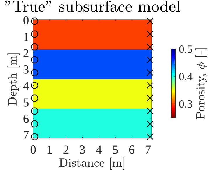
Figure A.3 – The "true" subsurface porosity model used in our synthetic crosshole-GPR experiment. The transmitter (black crosses) and receiver antennas (black circles) are indicated.
