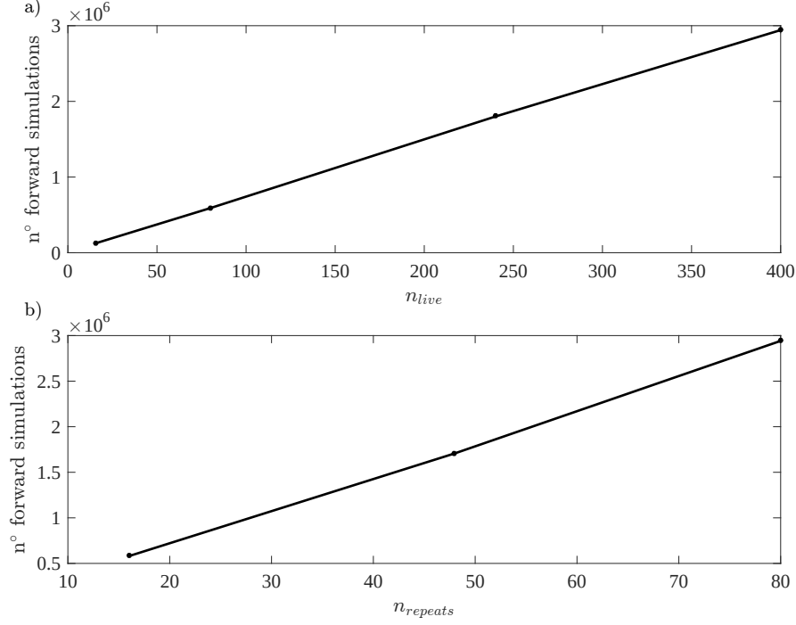
Figure A.6 – Linear relationship between the number of forward simulations and (a) n_{live} and (b) n_{repeats} in the case of the layered model with 16 layers.
