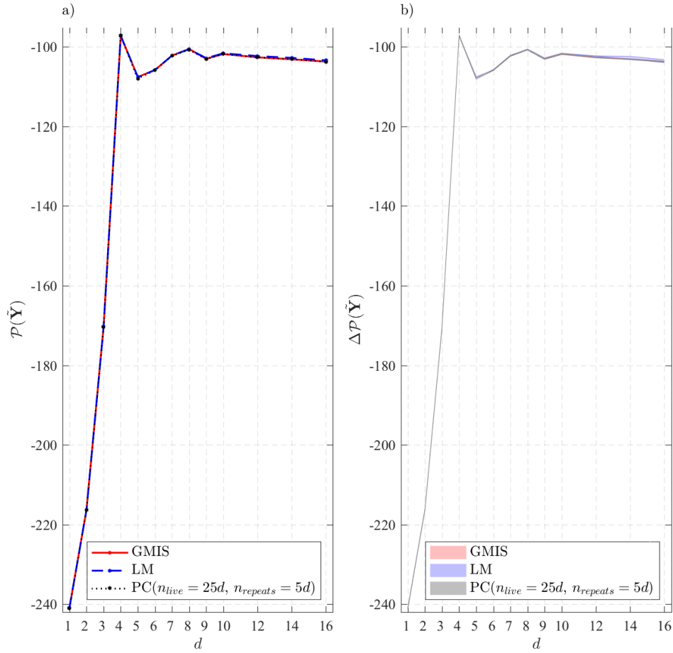
Figure A.4 – Evidence values in \log_{10} space, \mathcal{P}(\tilde{\mathbf{Y}}) (a: left graph), and their associated uncertainty (b: right graph) derived from the GMIS, LM and PC estimators for each model dimension, d , used herein. Colour coding is used to differentiate among the different methods. The evidence estimates of the GMIS, LM and PC estimators are in excellent agreement and their uncertainty is small.
