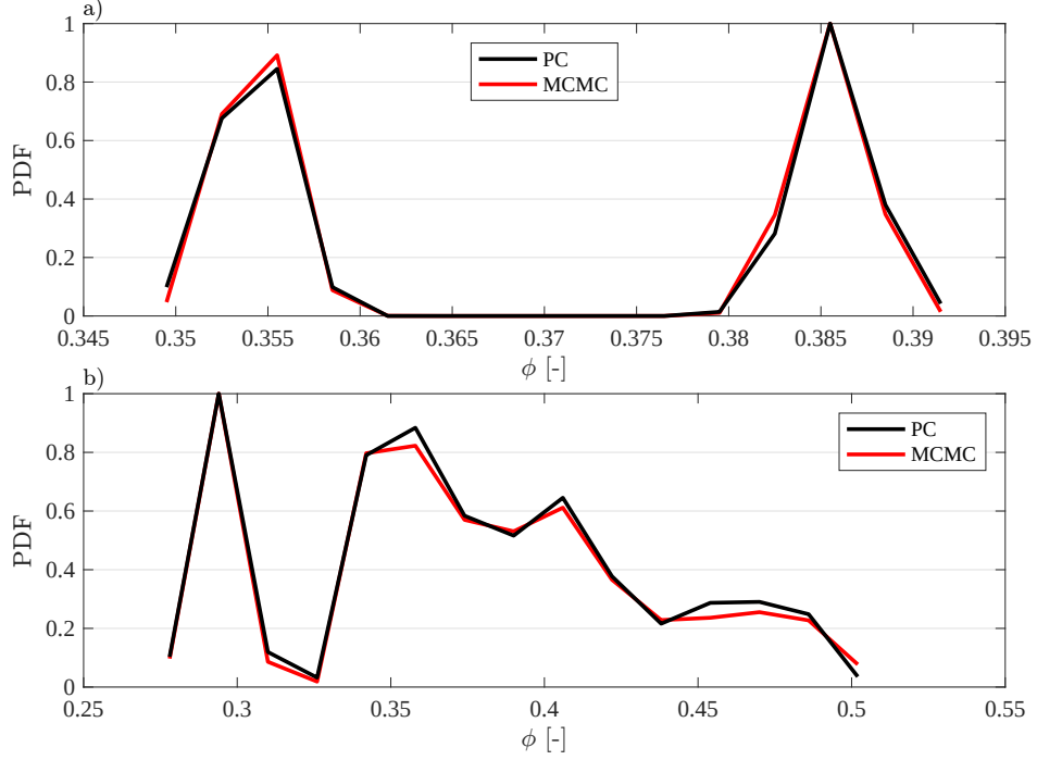
Figure A.8 – Marginal posterior distributions of the inferred porosity, \phi , for the horizontally layered model with (a) 2 layers and (b) 10 layers. The posterior distributions inferred by PC refer to the setting with n_{live} = 25d and n_{repeats} = 5d (Test B). The densities in each plot are normalized and colour coding is used to differentiate among the different methods to infer the posterior distributions.
