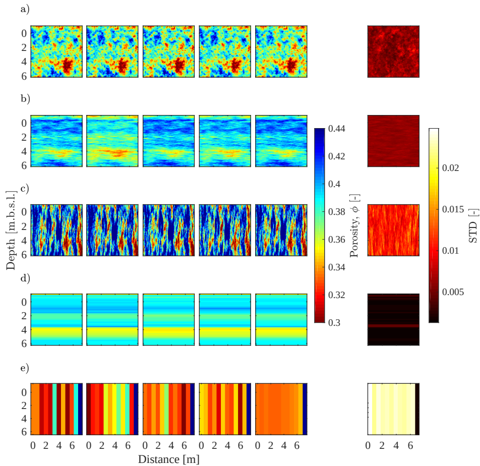
Figure 2.5 – Four realizations drawn randomly from the posterior distribution (first four columns), the posterior mean porosity field (fifth column) and the standard deviations of the posterior porosity estimates (last column) for the (a) isotropic multi-Gaussian model, (b) multi-Gaussian model with horizontal anisotropy, (c) multi-Gaussian model with vertical anisotropy, (d) horizontally layered model with 37 layers of equal thickness, and (e) vertically layered model with 12 layers of equal thickness.
