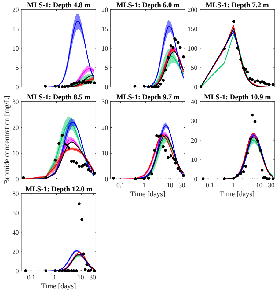
Figure 4.12 – Simulated (solid lines) and measured (black dots) bromide breakthrough curves from the MADE-5 experiment in the monitoring well MLS-1 at different depths. The simulated breakthrough curves are summarised by the mean of the posterior realisations and their thicknesses depict the 95% confidence intervals for the hybrid (red line), multi-Gaussian (black line), analog-based (magenta line), lithofacies-based (blue line) and outcrop-based conceptual model (green line).
