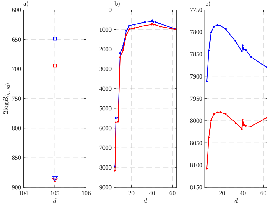
Figure 2.8 – Twice the natural logarithm of the Bayes factors of the best model (isotropic multi-Gaussian) of the ensemble with respect to the (a) multi-Gaussian model with horizontal anisotropy (squares) and vertical anisotropy (triangles), and the two conceptual models with (b) horizontal and (c) vertical layering of the porosity. Results are shown for the LM (blue) and the GMIS (red) methods.
