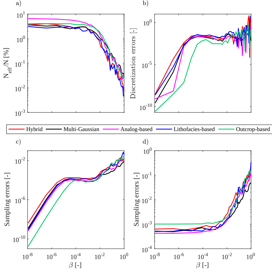
Figure 4.8 – (a) Percentage ratio between the effective and the total number of MCMC samples, (b) discretisation errors in the thermodynamic integration method (square root of Eq. 4.10), (c) sampling errors in the thermodynamic integration method (square root of Eq. 4.9) and (d) sampling errors in the stepping-stone sampling method (square root of Eq. 4.15) as a function of \beta -values. Note that all the x- and y-axes are in \log_{10} scale.
