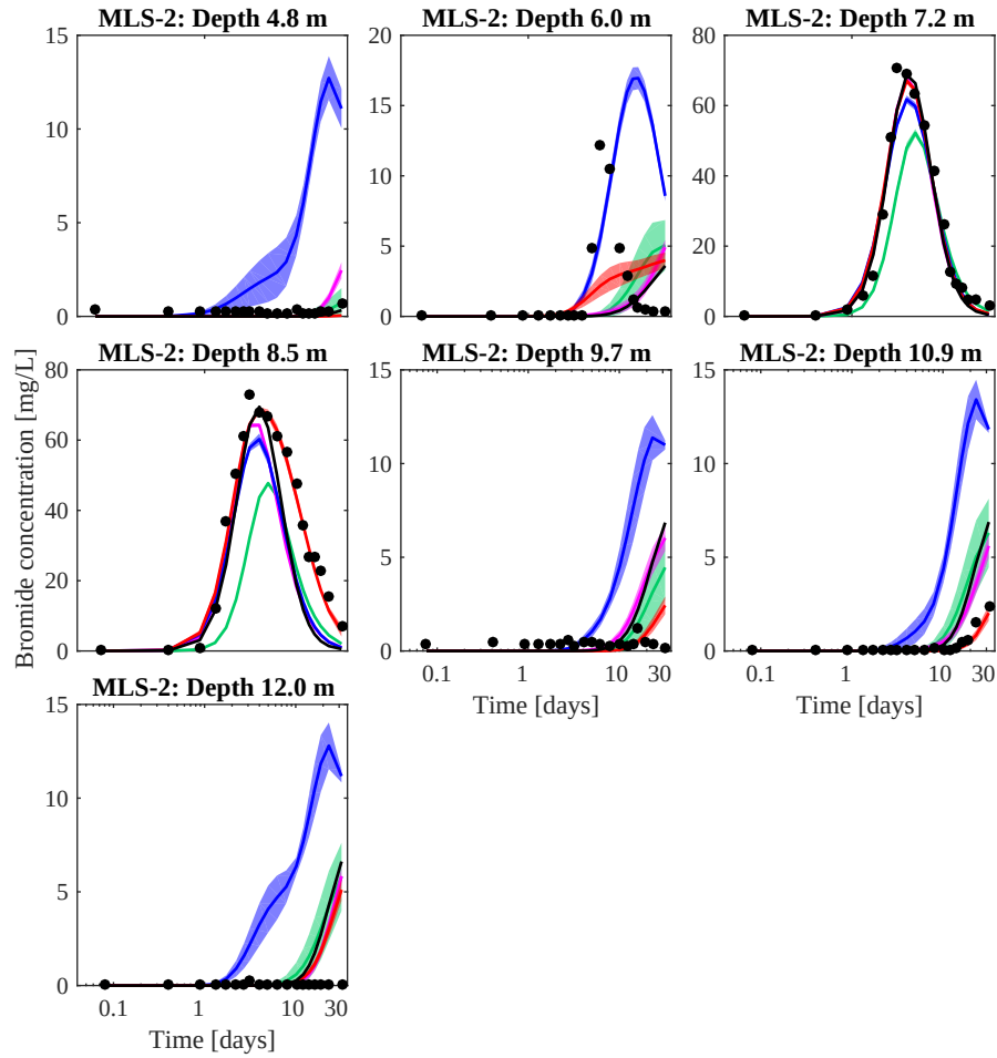
Figure 4.13 – Simulated (solid lines) and measured (black dots) bromide breakthrough curves from the MADE-5 experiment in the monitoring well MLS-2 at different depths. The simulated breakthrough curves are summarised by the mean of the posterior realisations and their thicknesses depict the 95% confidence intervals for the hybrid (red line), multi-Gaussian (black line), analog-based (magenta line), lithofacies-based (blue line) and outcrop-based conceptual model (green line).
