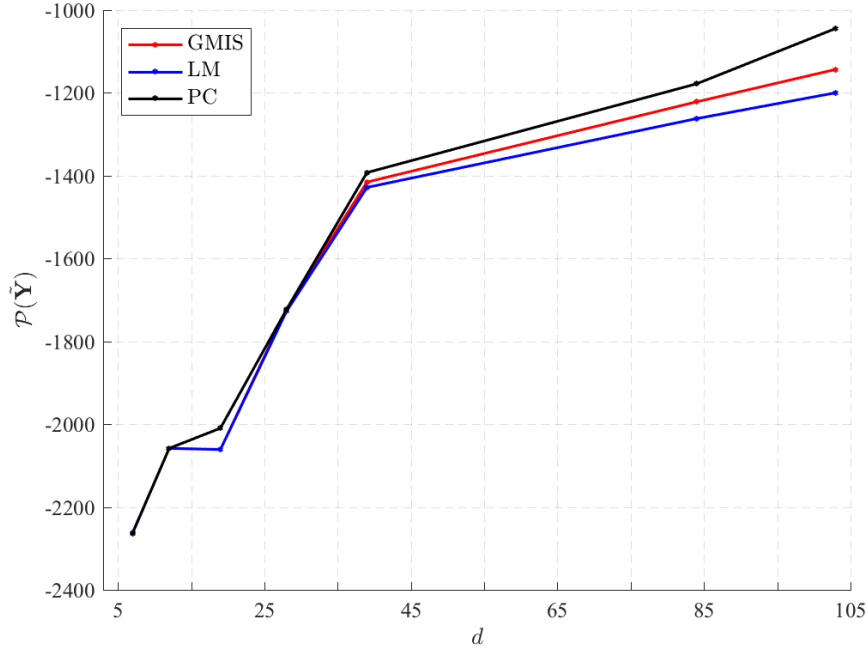
Figure A.11 – Evidence in \log_{10} space, \mathcal{P}(\tilde{\mathbf{Y}}) derived from the GMIS, LM and PC estimators for each model dimension, d , used herein. Colour coding is used to differentiate among the different methods.
