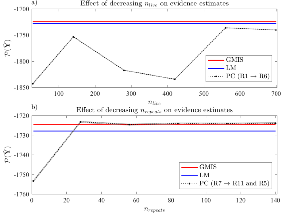
Figure A.9 – Evidence values in \log_{10} space, \mathcal{P}(\tilde{\mathbf{Y}}) , as function of (a) n_{live} and (b) n_{repeats} for a uniform gridded conceptual model with 5 \times 5 grid cells. The evidence estimated by GMIS and LM methods are indicated with the red line and the blue line, respectively.
