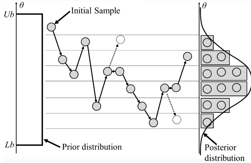
Figure 1.3 – Simplified representation of a Markov chain for a model parameter, \theta , drawn from an uniform prior distribution \mathcal{U}(L_b, U_b) . The circles indicate the states of the chain and the arrows indicate the moves from one state to another. The dotted arrows and circles represent the proposed moves and samples that were not accepted based on the acceptance criterion, \alpha (Figure modified from Lee et al. (2015)).
