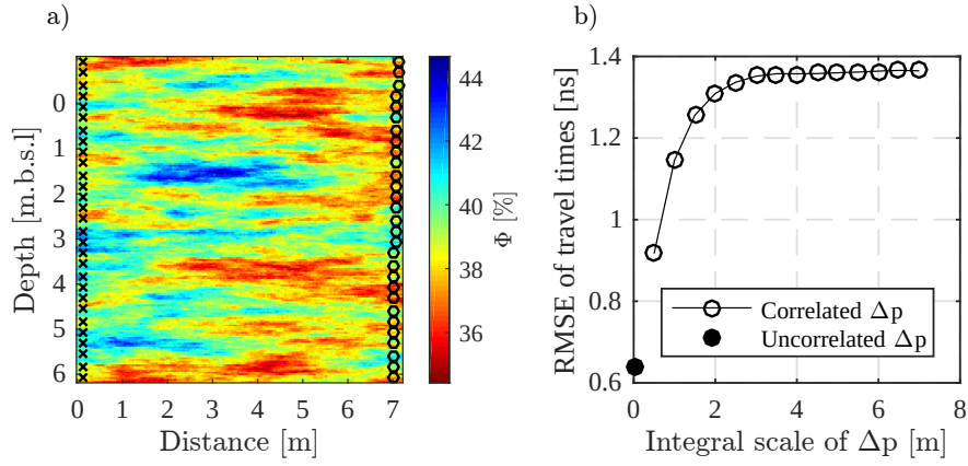
Figure 3.2 – (a) The true porosity model used in our synthetic examples. The 29 GPR transmitter (black crosses) and 29 receiver (black circles) locations are indicated. (b) Root mean square error of GPR travel time data as a consequence of observational errors and petrophysical prediction uncertainty with increasing correlation. In the absence of petrophysical prediction uncertainty, the RMSE is 0.5 ns.
