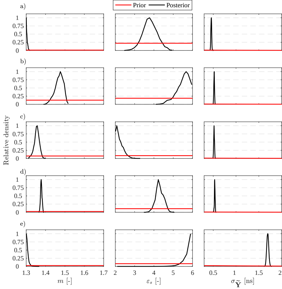
Figure 2.6 – Marginal posterior distributions of the inferred cementation index, m (first column), the relative permittivity of the mineral grains \varepsilon_s (second column), and the inferred data error, \sigma_{\tilde{Y}} (third column) for the multi-Gaussian models with (a) isotropy, (b) horizontal anisotropy, and (c) vertical anisotropy of the porosity values, and the two models with (d) horizontal and (e) vertical layering. The prior distribution is indicated separately in each plot using the red lines. The densities in each plot are normalized so that they all share the units of the y -axis on the left.
