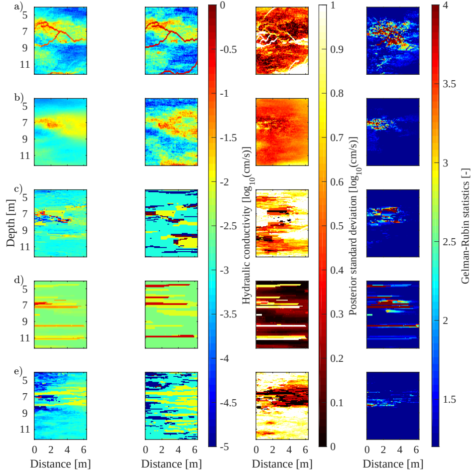
Figure 4.4 – Mean (first column), maximum a-posteriori (second column), and standard deviation (third column) of the posterior hydraulic conductivity realisations for the (a) hybrid, (b) multi-Gaussian, (c) analog-based, (d) lithofacies-based and (e) outcrop-based conceptual model at the MADE site. In the last column, the Gelman-Rubin statistic for each pixel is reported. Dark-blue regions represent values equal or less than 1.2 and indicate that convergence has been reached for those pixels.
