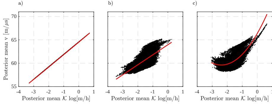
Figure 3.11 – Scatter plots of the mean posterior hydraulic conductivity estimates against the mean posterior GPR velocity estimates assuming a (a) perfect linear, (b) scattered linear and (c) scattered quadratic petrophysical relationship. The red lines depict the inferred mean petrophysical relationship, while the scatter represents the inferred mean petrophysical prediction uncertainty.
