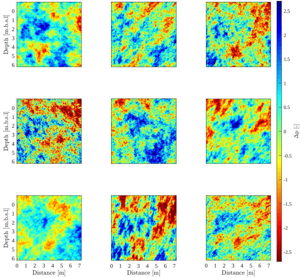
Figure 3.8 – Nine realizations of the petrophysical prediction uncertainty field drawn randomly from the posterior distribution obtained from MCMC simulation with the DREAM (ZS) algorithm using 8 chains with 2.5 \cdot 10^5 iterations. The petrophysical prediction uncertainty is conceptualized by a multi-Gaussian field with isotropy.
