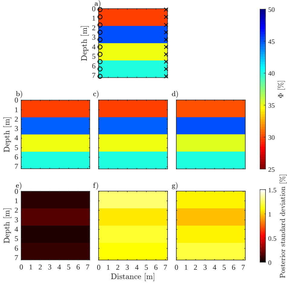
Figure 3.1 – (a) The "true" subsurface porosity model used in our toy example with the different measurement depths of the GPR transmitters (black crosses) and receivers (black circles) indicated. Mean porosity fields of the posterior distribution derived from MCMC simulation with the DREAM (ZS) algorithm using a conceptual model with four layers in the case where (b) the petrophysical prediction uncertainty is not taken into account, (c) the petrophysical prediction uncertainty is sampled by MCMC and (d) the petrophysical prediction uncertainty is sampled by MC-within-MCMC. The corresponding posterior standard deviations of the porosity estimates are shown in (e), (f) and (g), respectively. All these plots were obtained with \sigma_{\tilde{Y}} = 0.5 ns
