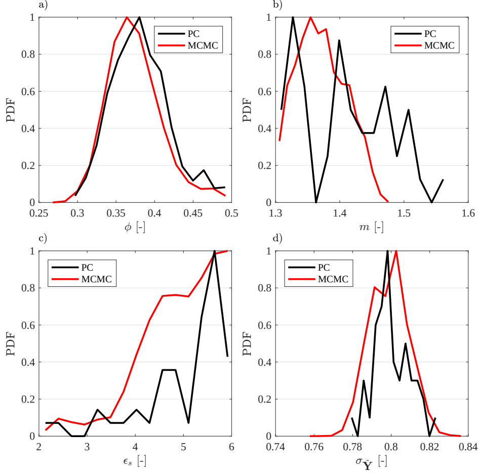
Figure A.10 – Marginal posterior distributions of (a) the inferred porosity, \phi , (b) the inferred cementation index, m , (c) the inferred relative permittivity of the mineral grains, \epsilon_s and (d) the inferred data error, \sigma_{\tilde{Y}} , for the gridded model with 5 \times 5 grid cells. The posterior distributions inferred by PC refer to the setting with n_{live} = 300 and n_{repeats} = d (i.e., in this case d is equal to 28). The densities in each plot are normalized and colour coding is used to differentiate among the different methods used to infer the posterior distributions.
