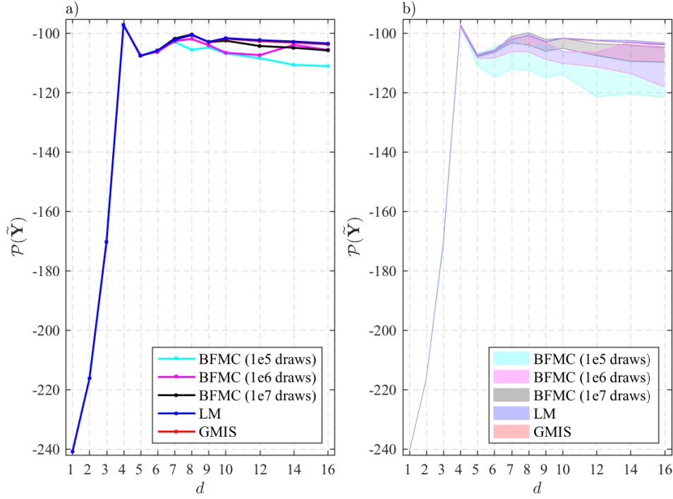
Figure 2.2 – Mean values of the evidence in \log_{10} space, \mathcal{P}(\tilde{\mathbf{Y}}) (a: left graph), and their associated uncertainty (b: right graph) derived from the BFMC, LM, and GMIS estimators for each model complexity, d used herein. Color coding is used to differentiate among the different methods. The evidence estimates of the LM and GMIS estimators are in excellent agreement and their uncertainty is negligibly small.
