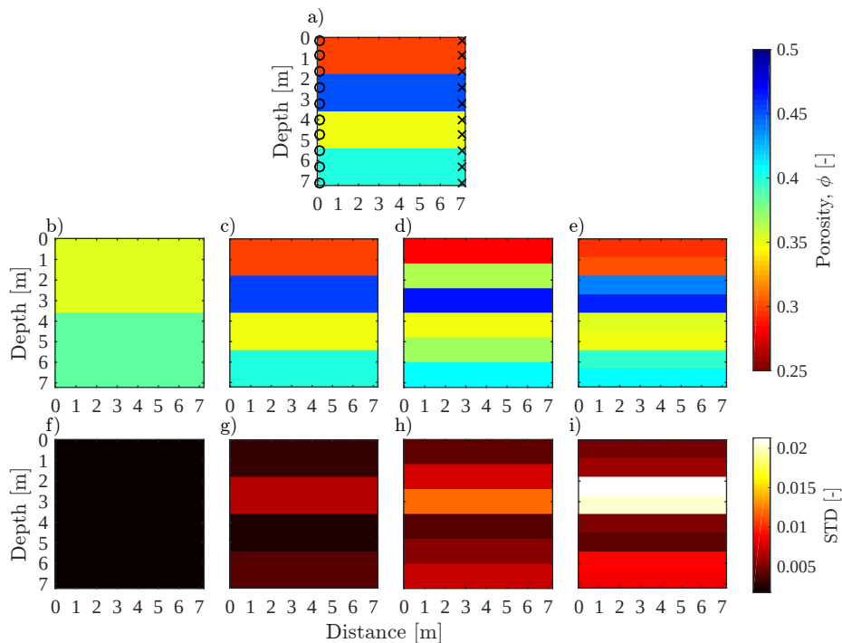
Figure 2.1 – a) The "true" subsurface porosity model used in our synthetic crosshole-GPR experiment. The different measurement depths of the transmitter antenna (black crosses) and receiver antenna (black circles) are separately indicated. Mean porosity fields of the posterior distribution derived from MCMC simulation with the DREAM (ZS) algorithm using four different conceptualizations of the subsurface involving (b) two, (c) four, (d) six, and (e) eight horizontal layers. The corresponding posterior standard deviations of the porosity estimates for the four different conceptualizations of the subsurface are shown in (f), (g), (h) and (i), respectively.
