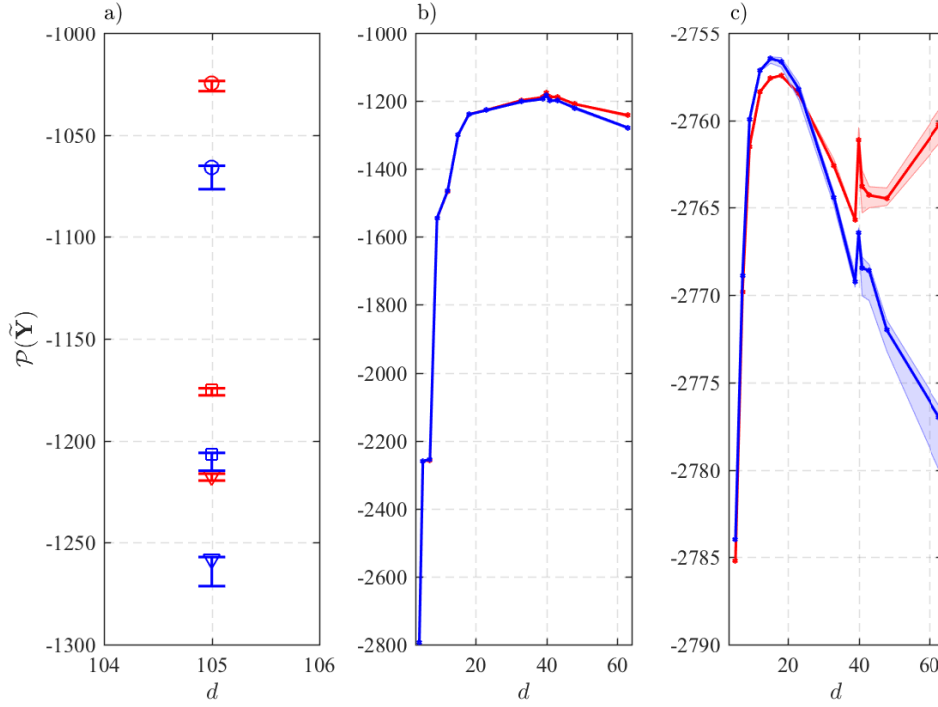
Figure 2.7 – Mean values of the evidence in \log_{10} space, \mathcal{P}(\tilde{\mathbf{Y}}) , derived from the LM (blue) and GMIS (red) methods for (a) the multi-Gaussian models with isotropy (circles), horizontal anisotropy (squares), and vertical anisotropy (triangles), and the two models with (b) horizontal, and (c) vertical layering of the porosity. The error bars in (a) and the shaded areas in (b) and (c) summarize the ranges of the evidence estimates as derived from the different independent trials with both methods.
