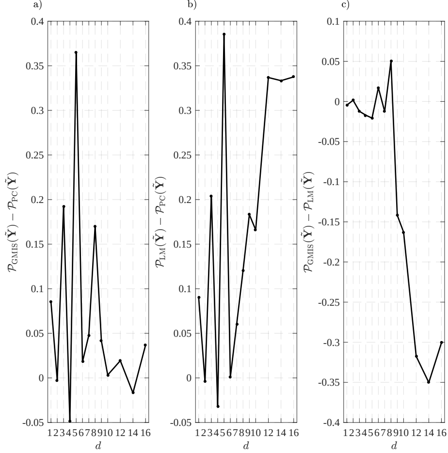
Figure A.5 – Difference in the evidence estimates derived from different pairs of two methods as function of model dimension, (a) GMIS and PC, (b) LM and PC, and (c) GMIS and LM. Note, we use \log_{10} transformed value of the evidence estimates.
