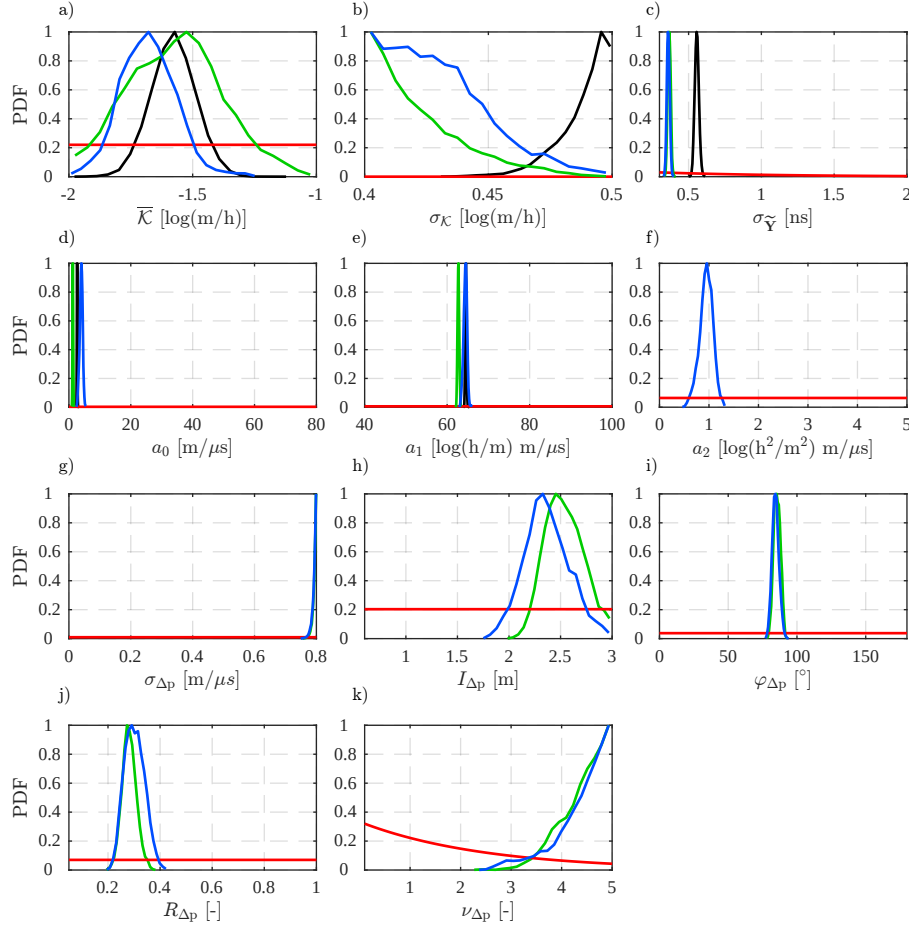
Figure 3.9 – Posterior distributions derived from MCMC simulation with the DREAM (ZS) algorithm using 8 chains with 5 \cdot 10^5 iterations of the (a) mean, \bar{\mathcal{K}} , and (b) standard deviation, \sigma_{\mathcal{K}} , of the log-hydraulic conductivity field. Posterior distributions of the (c) standard deviation of the measurement errors, \sigma_{\tilde{Y}} , and the polynomial coefficients of the (d) constant, a_0 , (e) linear, a_1 and (f) quadratic, a_2 , terms describing the petrophysical relationships of Eqs. (3.9)-(3.11). Posterior distributions of the geostatistical parameters of the petrophysical prediction uncertainty field: (g) standard deviation, \sigma_{\Delta p} , (h) integral scale along the major axis of anisotropy, I_{\Delta p} , (i) anisotropy angle, \varphi_{\Delta p} , (j) ratio of the integral scales along the minor and major axis of anisotropy, R_{\Delta p} , and (k) shape parameter of the Matérn variogram, \nu_{\Delta p} . The results for the perfect linear, scattered linear and scattered quadratic petrophysical relationship are depicted with black, green and blue lines, respectively. The red lines indicate the corresponding prior distributions. The densities in each plot are normalized.
