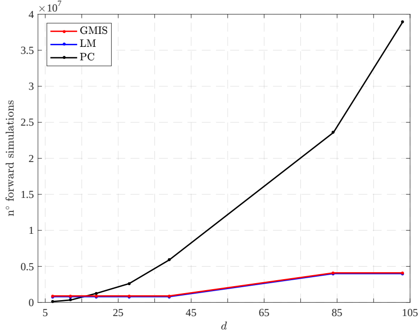
Figure A.13 – Number of forward simulations required for estimating the evidence by GMIS (red), LM (blue) and PC (black) as a function of model dimension. At high model dimensions, the number of forward simulations required by PC is at least one order of magnitude larger than the ones required by GMIS and LM estimators.
