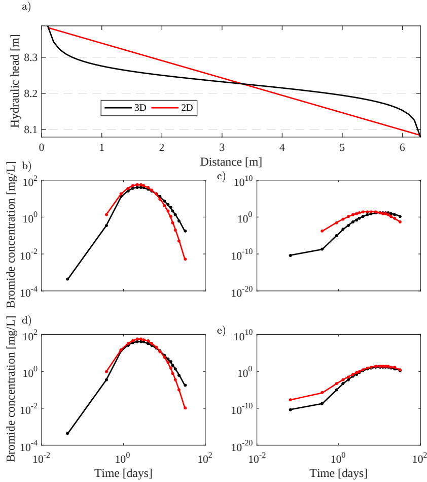
Figure 4.11 – (a) Hydraulic head profiles between the injection and extraction wells arising from 2D and 3D flow simulations in a uniform hydraulic conductivity field. Simulated breakthrough curves at 7 m depth in (b) MLS-1 and (c) MLS-2 without corrections. The shifts in the 2D simulations are removed when (d-e) applying the correction factors.
