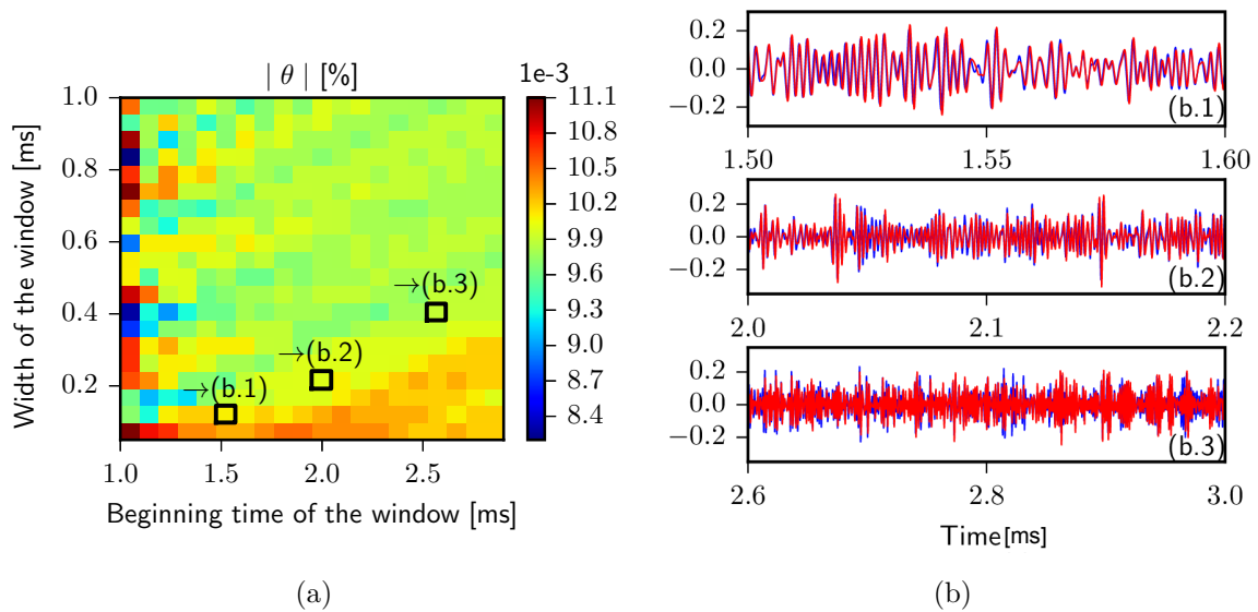
FIGURE 2.3 – (a) Absolute value of the relative variation in velocity |\theta| for different beginning times of the windows and different window lengths : b) Examples of temporal signals for three different windows : b.1) [1.5 ms, 1.6 ms], b.2) [2.0 ms, 2.2 ms], and b.3) [2.6 ms, 3.0 ms].
