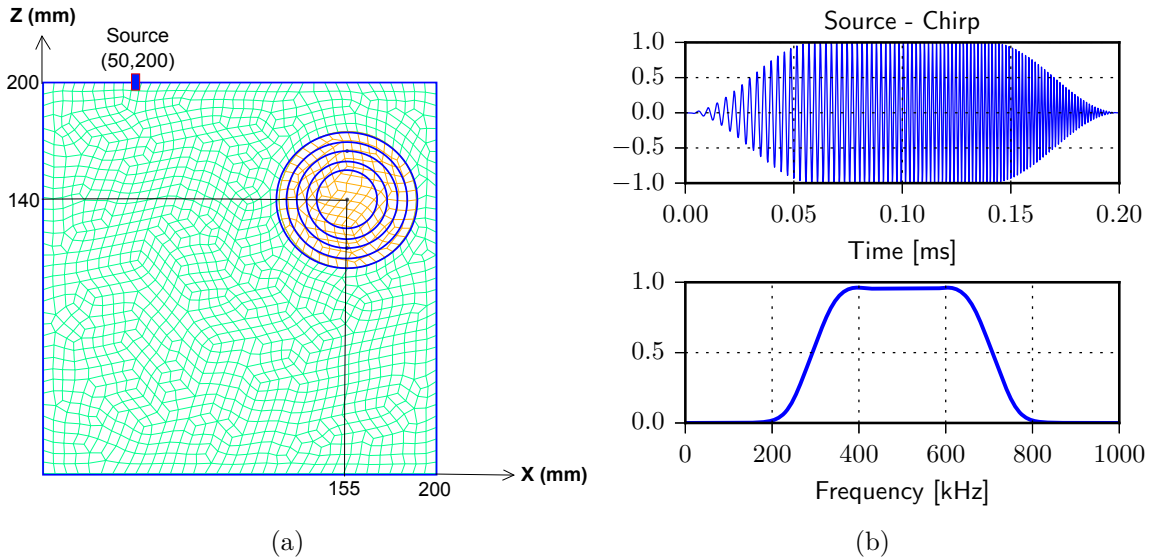
FIGURE 2.2 – Numerical configurations of the tests : a) Meshes of the configurations with five distinct Effective Damage Zones (EDZ) of various sizes. The blue lines represent the contour of both the matrix and the EDZ. For each model, the matrix size equals 200 \times 200 mm ^2 , and the circular EDZ center is located at (155 mm, 140 mm). The EDZ radius for each model varies from 15 mm to 35 mm. The source position is (50 mm, 200 mm); b) Probe wave source signal : top) chirp source in the time domain (normalized amplitude); bottom) chirp source in the frequency domain (Fourier transform) (normalized amplitude).
