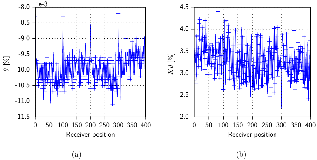
FIGURE 2.5 – CWI observables vs. receiver position. The model used is a matrix with a localized Effective Damage Zone (EDZ) of radius 25 mm ; the EDZ has been modeled by a change in Young’s modulus : E_{edz} = E_{mtx} \times (1 - 0.6\%) a) Relative variations in velocity \theta vs. receiver position, b) Remnant decorrelation coefficient Kd vs. receiver position.
